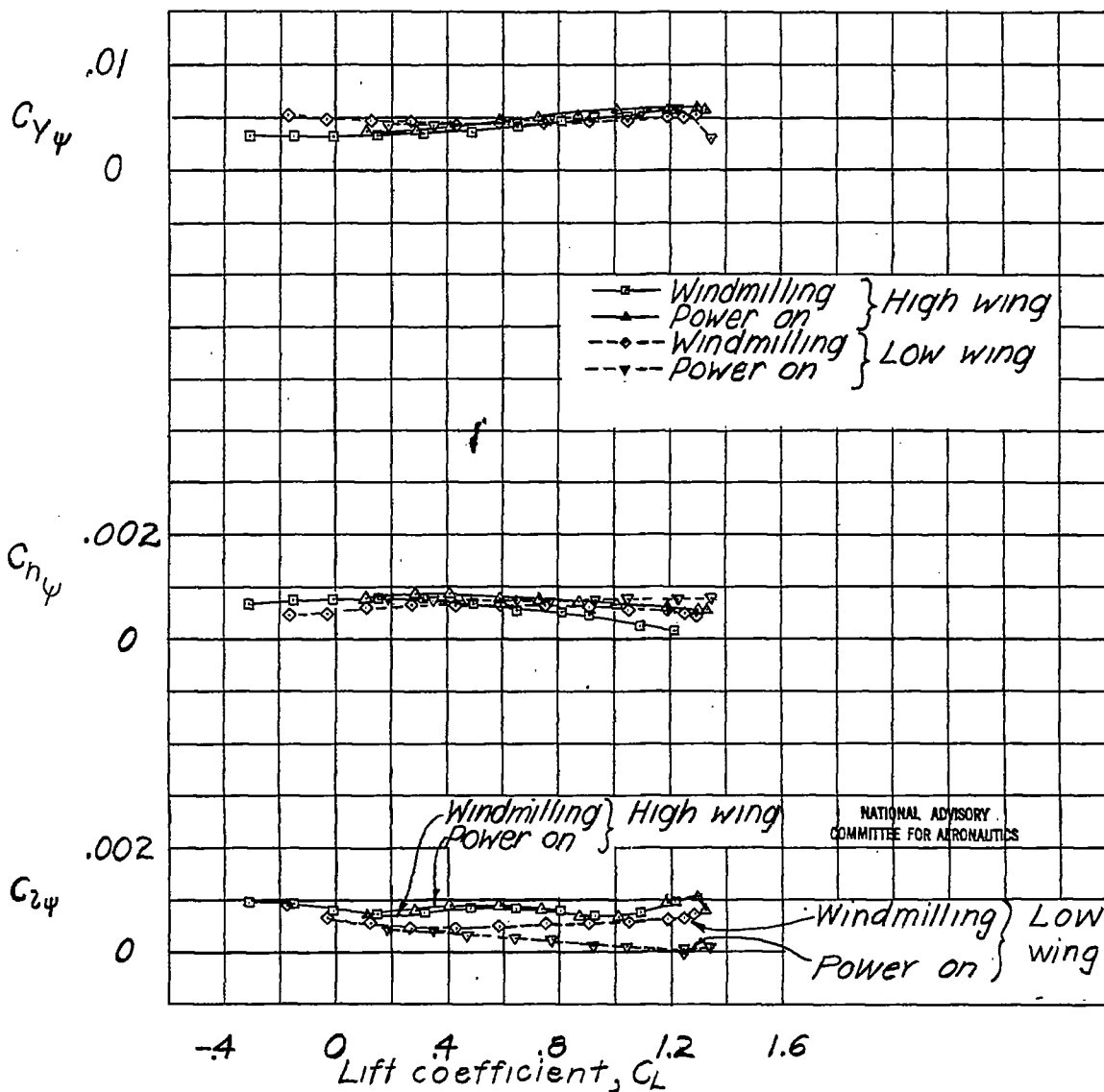
(a) Flaps retracted.
