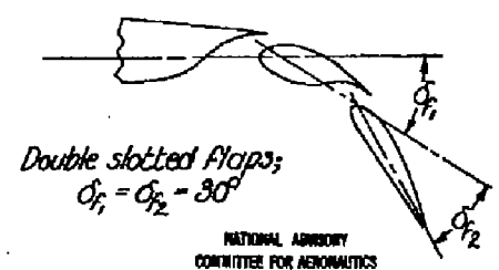
(b) Typical section, showing various flap arrangements; no scale.
