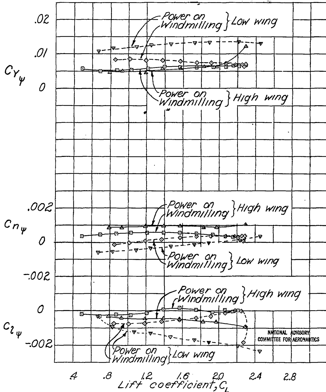
(b) Full-span single slotted flaps; \delta_f = 30^\circ .
