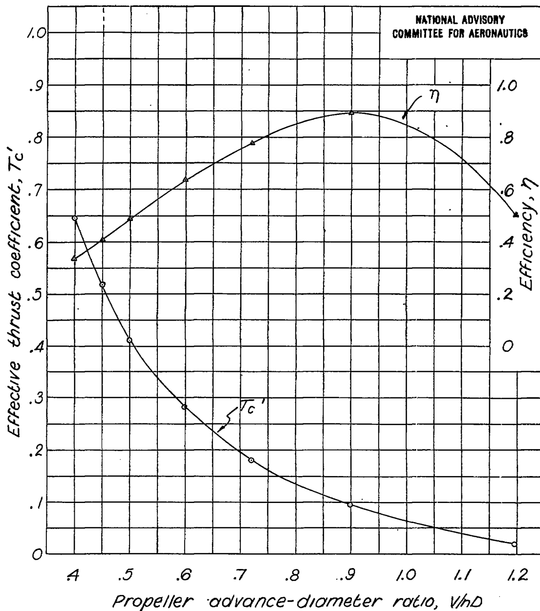
Figure 4.- Effective thrust coefficient and efficiency as functions of propeller advance-diameter ratio for the modified \frac{1}{3} -scale model of the Curtiss P-36A airplane. D=2.0 feet; \beta=25^\circ .
