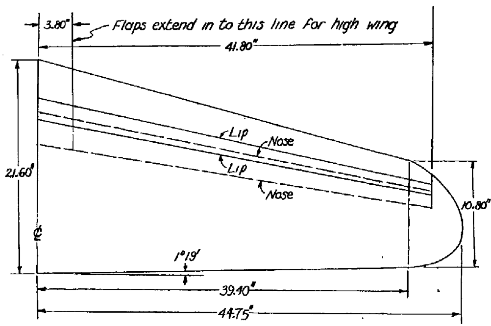
(a) Plan form of wing; \frac{1}{5} scale.
