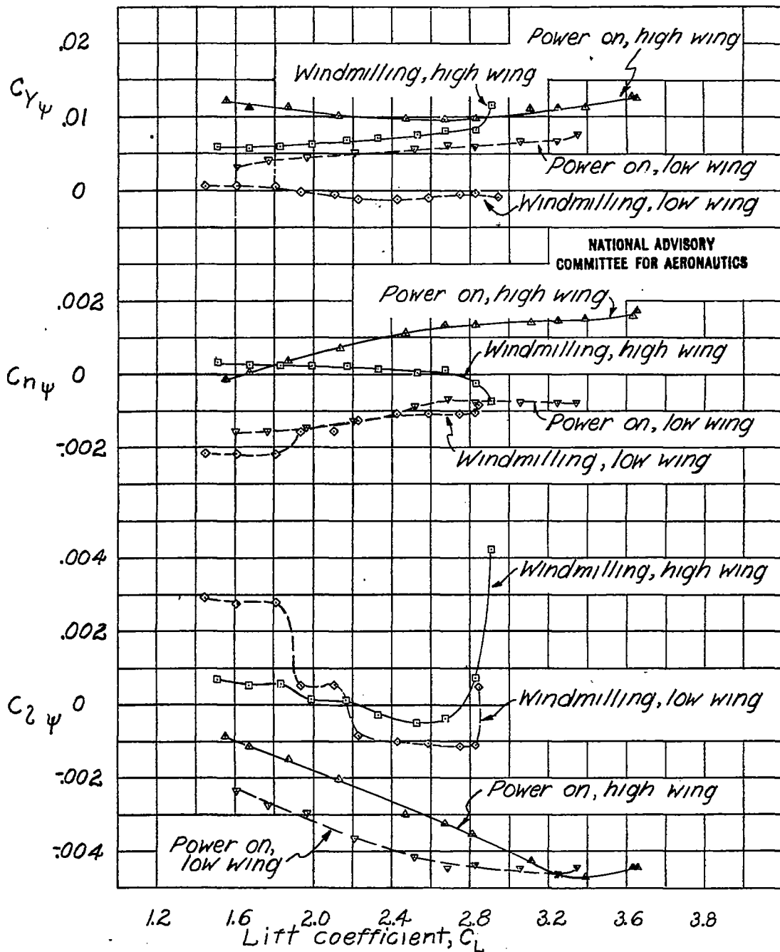
(c) Full-span double slotted flaps; \delta_{F_1} = \delta_{F_2} = 30^\circ .
