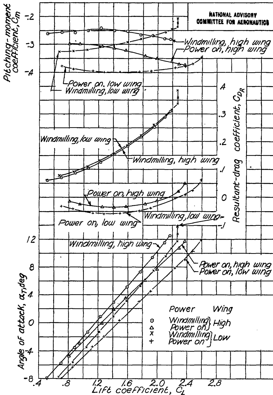
(b) Full-span single slotted flaps ; \delta_f = 30^\circ .
