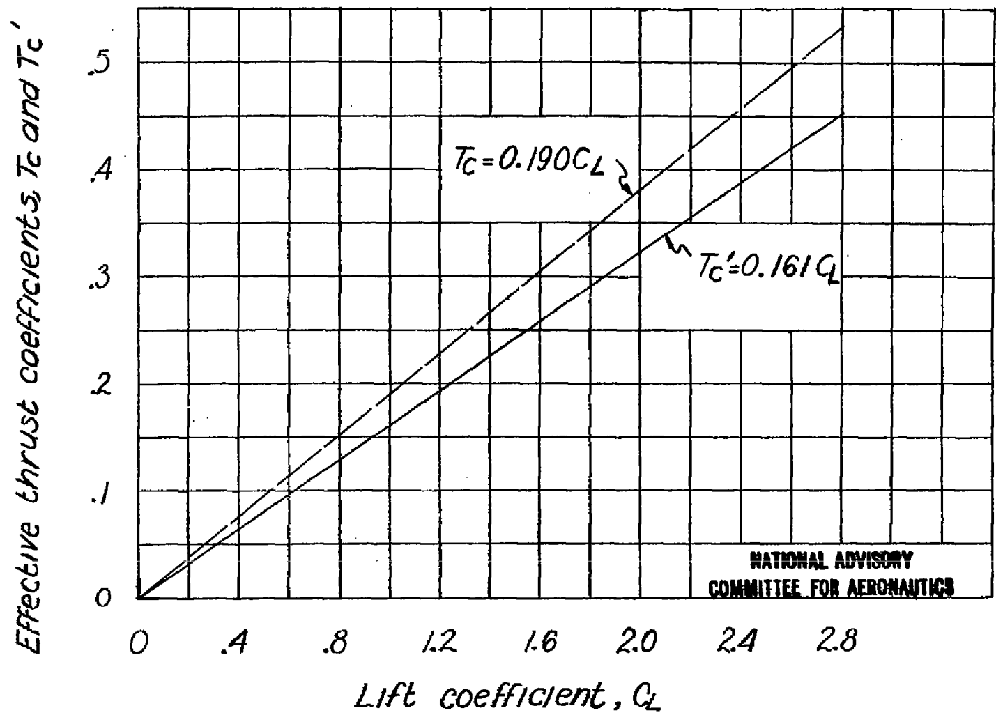
Figure 5.- Variation of effective thrust coefficients with lift coefficient.
