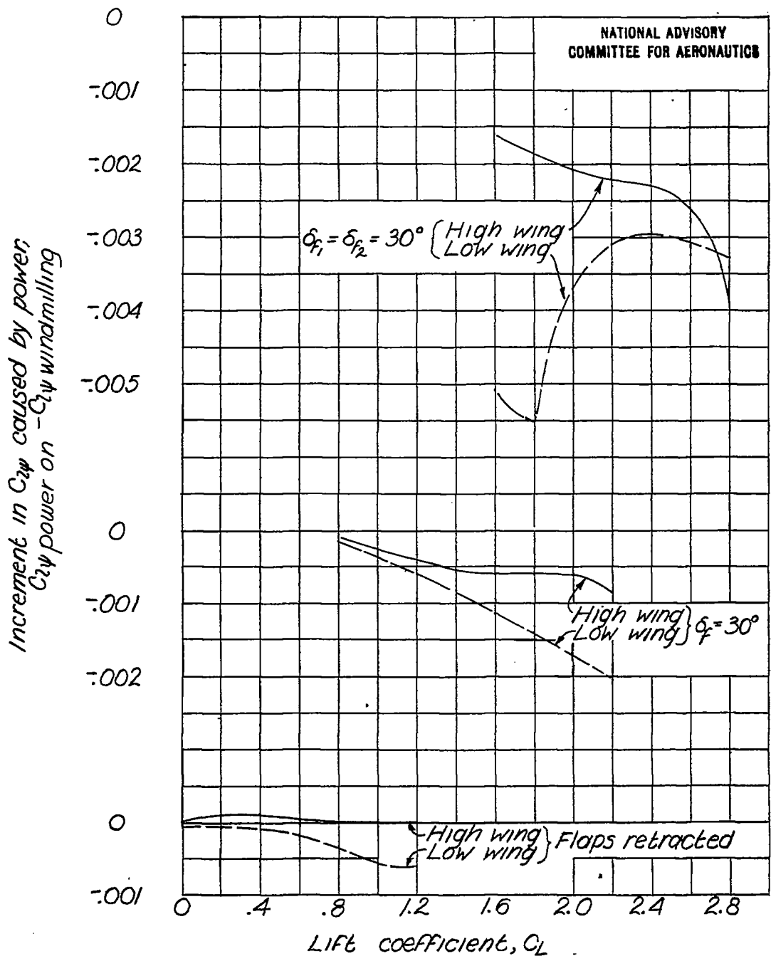
Figure 9.-Effect of power on C_{2\psi} . Modified \frac{1}{4} -scale model of the Curtiss P-36A airplane; tail removed.
