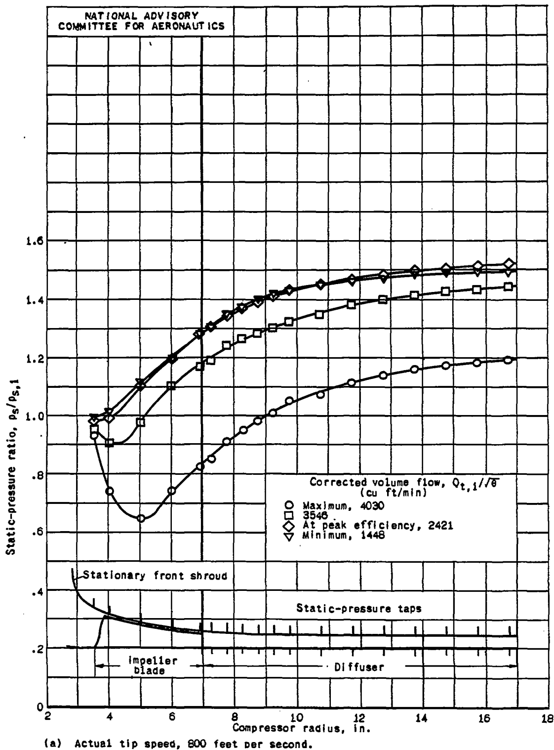
Figure 4. - Distribution of static-pressure ratio along radius of radial-inlet impeller and vaneless diffuser.
