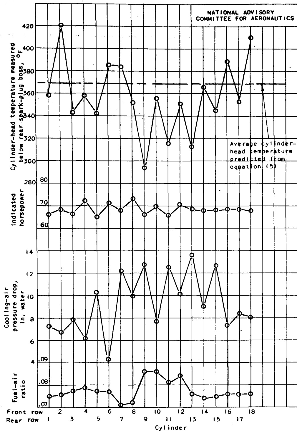
1a) Brake horsepower, 1000; engine speed, 2200 rpm.
