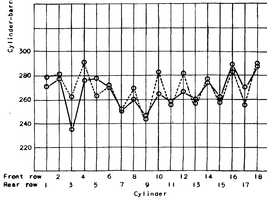
(b) Brake horsepower, 1400; engine speed, 2200 rpm.
