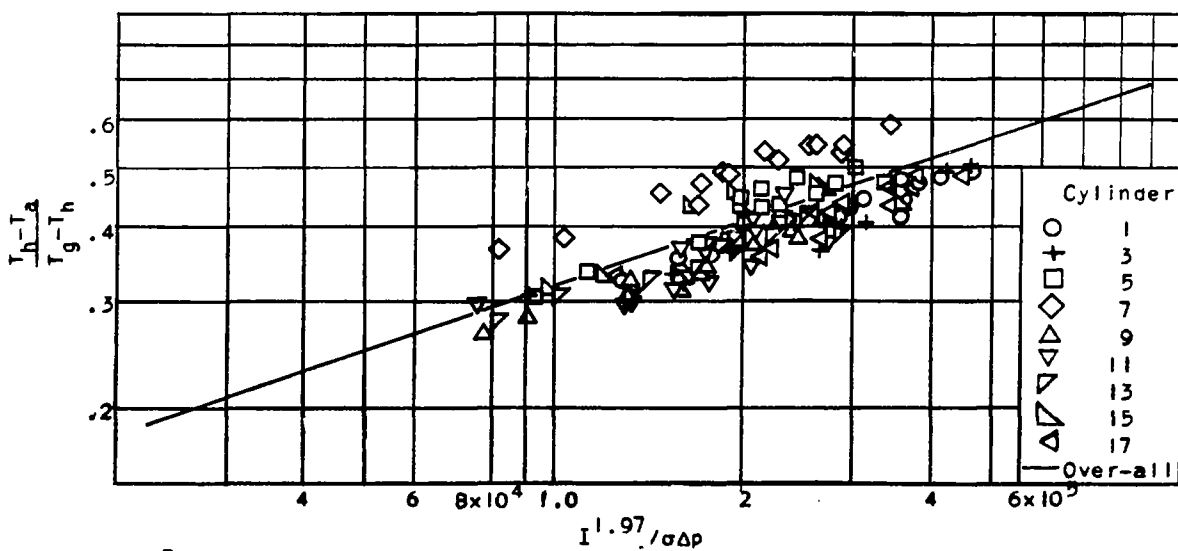
(a) Cylinder heads.
