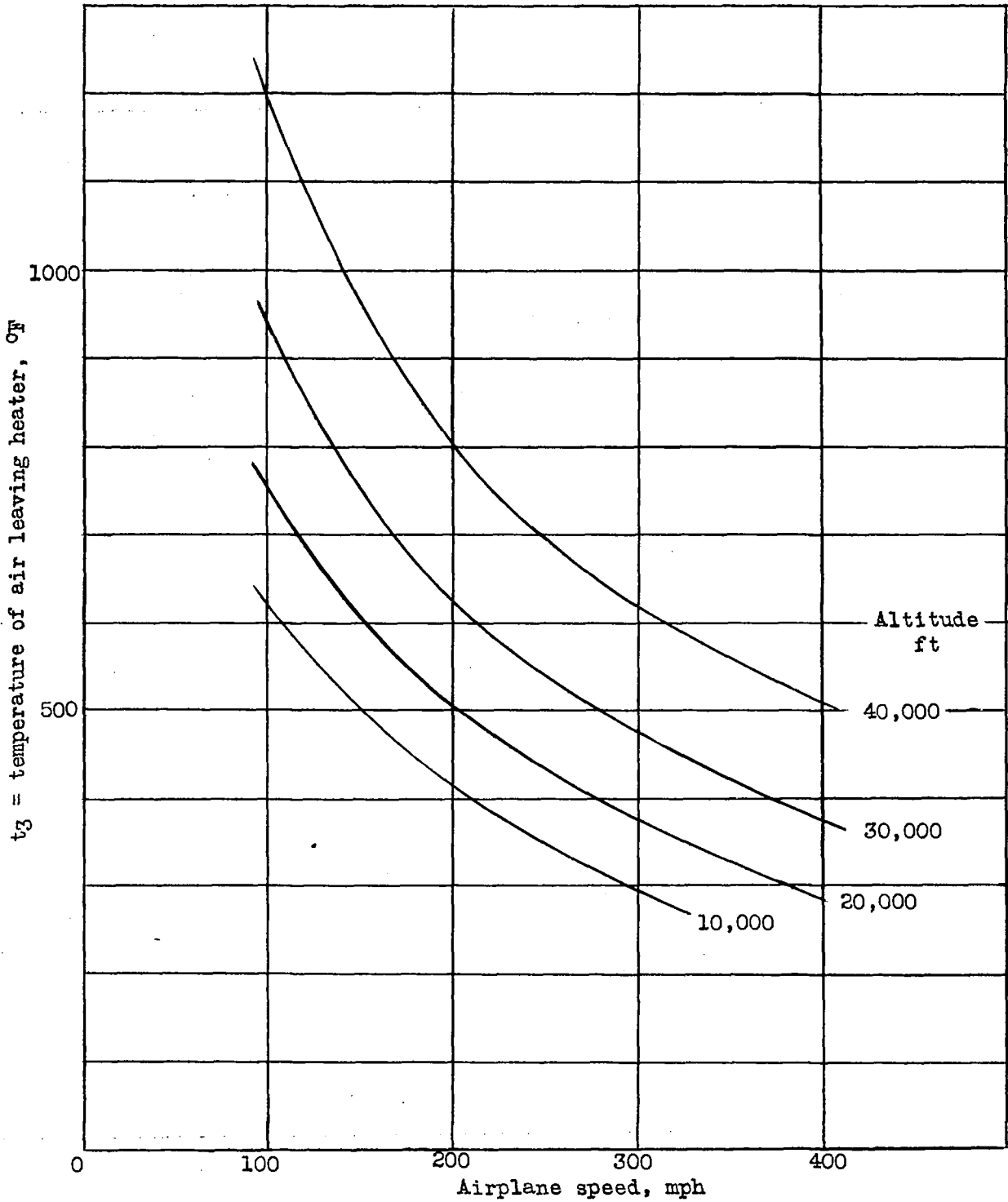
Figure 5.- Temperature of the air leaving the heater at various airplane speeds and altitudes.
