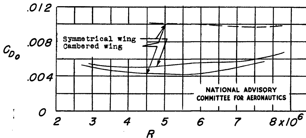
(b) High speed condition; C_L = 0.2 .
