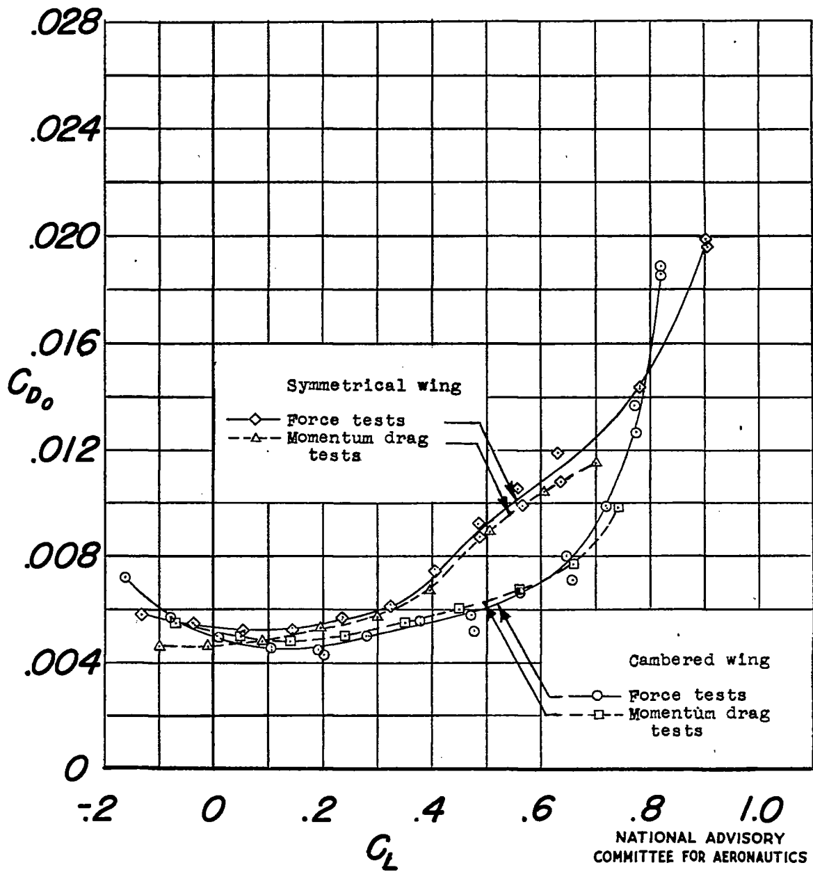
Figure 5.- Effect of airfoil modifications on the profile-drag coefficient; R=4,800,000 ; M = 0.13 .
