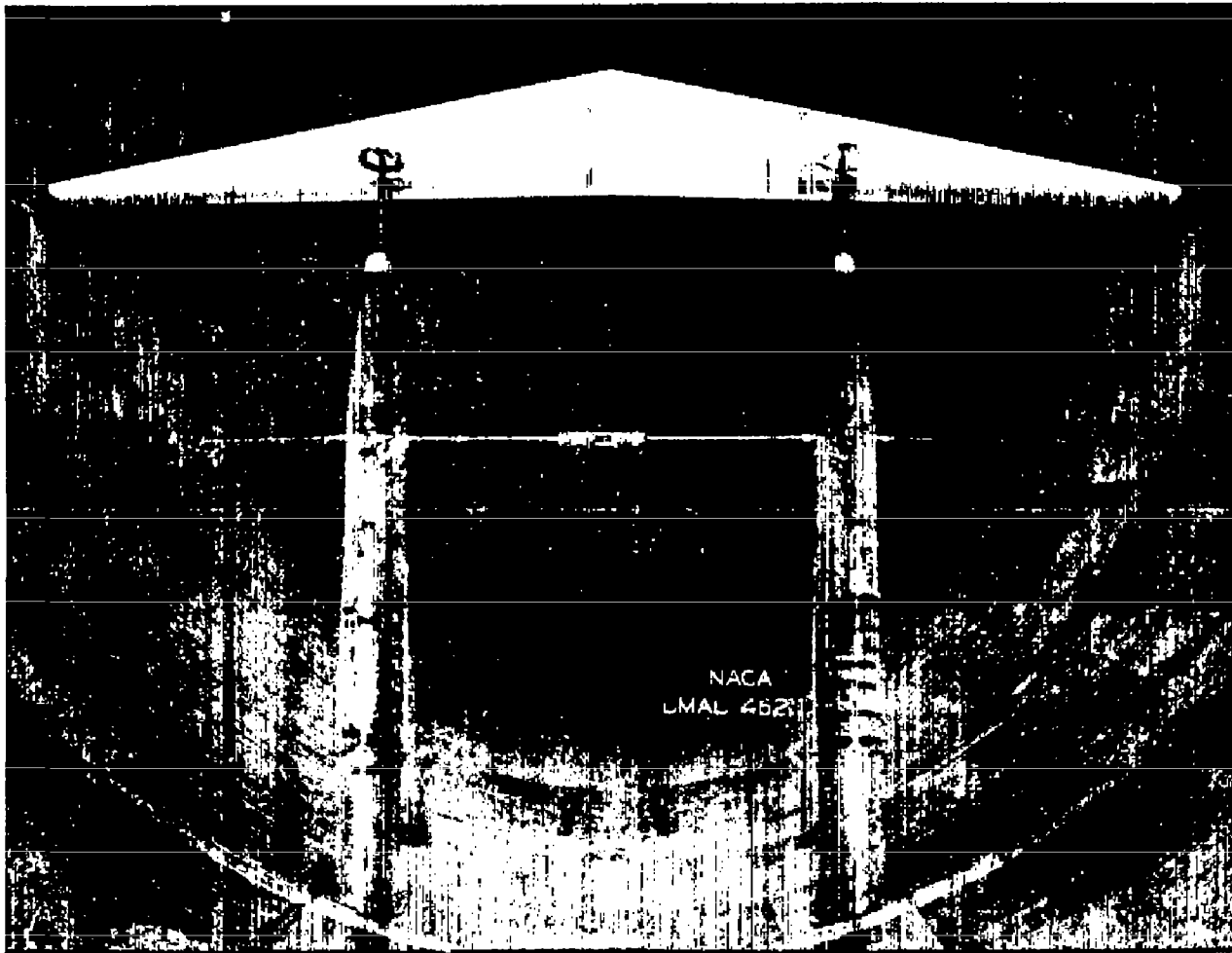
Figure 2.- Symmetrical wing mounted for testing in the Langley 19-foot pressure tunnel.
