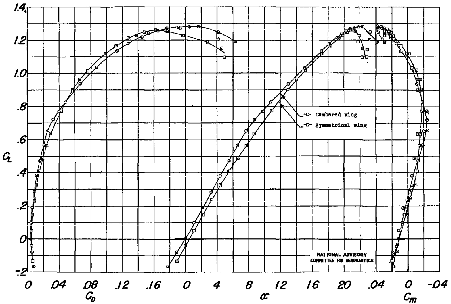
Figure 3.- Effect of airfoil modifications on aerodynamic characteristics; R=1,860,000 ; M = 0.15 .
