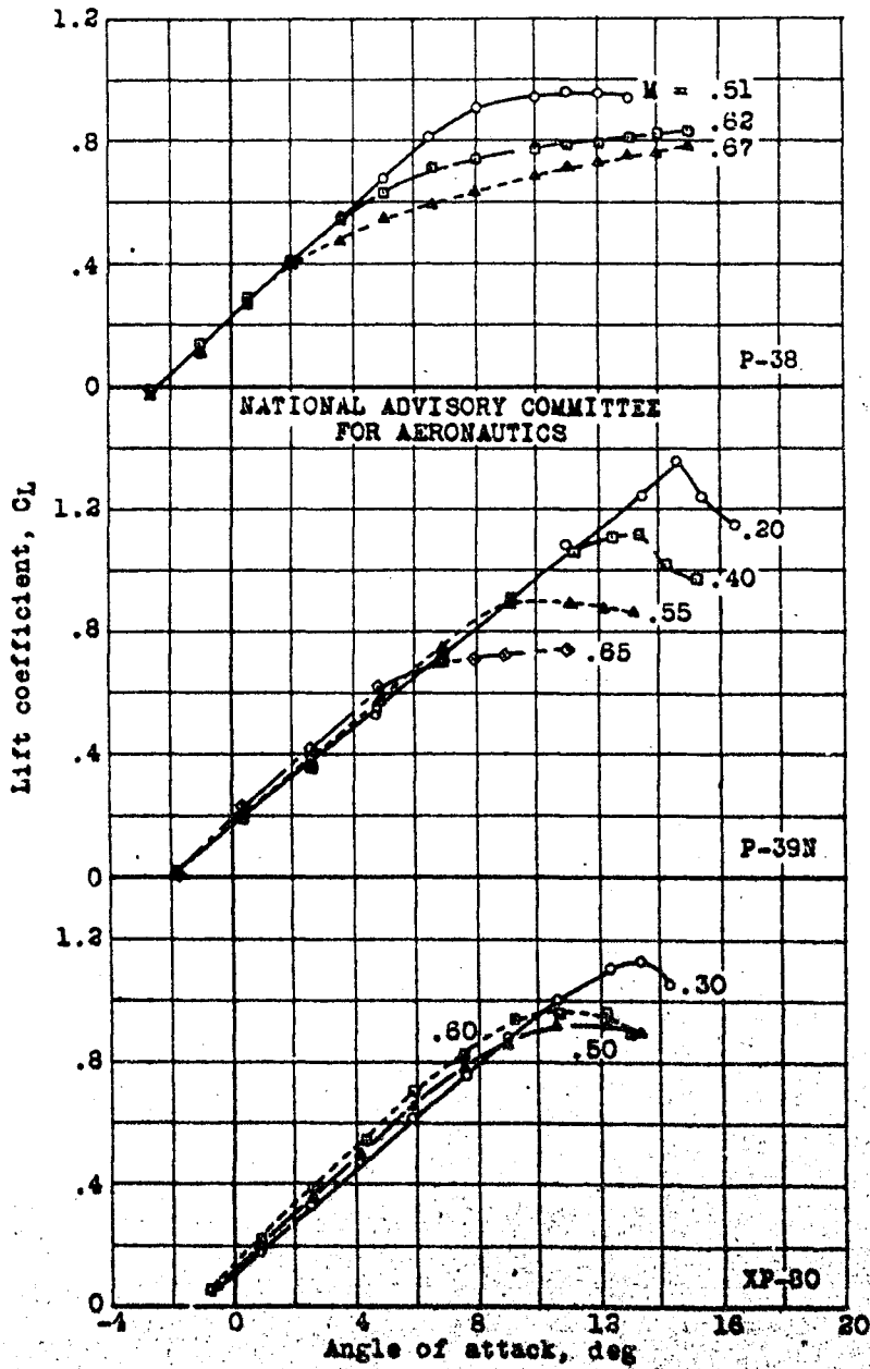
Figure 13.- Variation of lift coefficient with angle of attack at several Mach numbers for three models. Area 16-foot high-speed wind tunnel.
