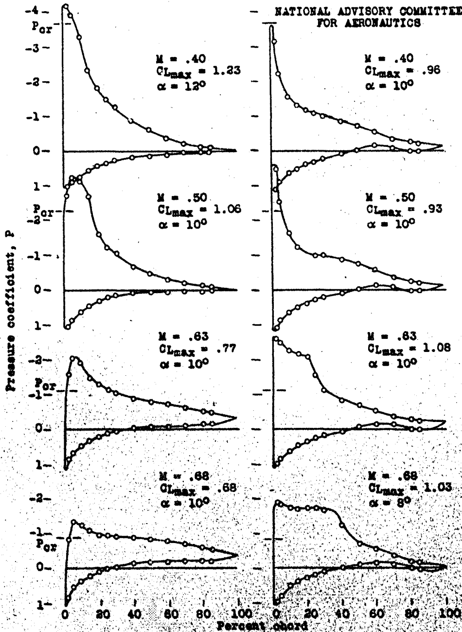
Figure 10. - Typical pressure distributions on NACA conventional and low-drag airfoils at maximum lift coefficient. Axes 1-by 3-1/2-foot high-speed wind tunnel.
