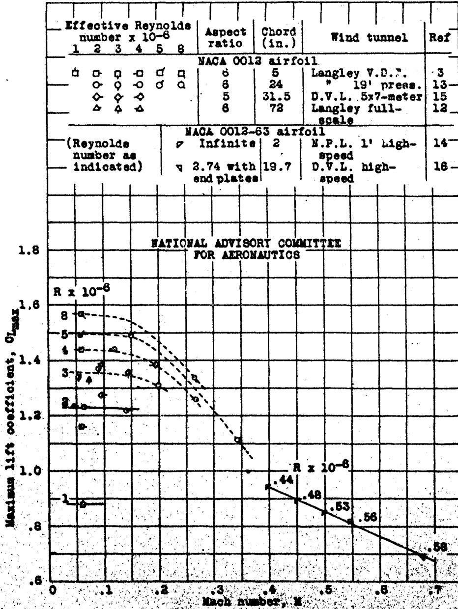
Figure 16.- Maximum lift coefficients of NACA 0012 and 0012-63 airfoils as measured in several wind tunnels.
