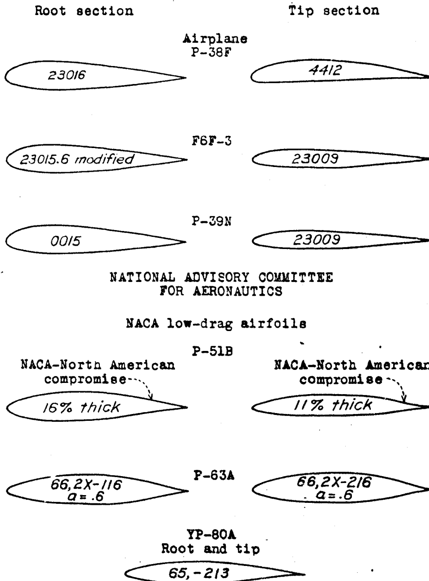
Figure 3.- Profiles of the wing root and tip sections of the test airplanes.
