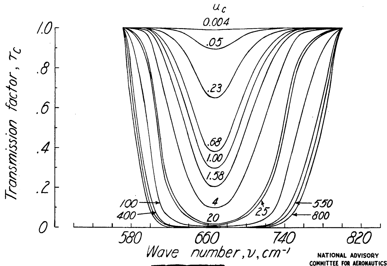
Figure 5.-Spectral transmission factor for the 667\text{ cm}^{-1} band of carbon dioxide. u_c , carbon-dioxide content, in centimeters, at 0^\circ\text{C} and 1013 millibars.
