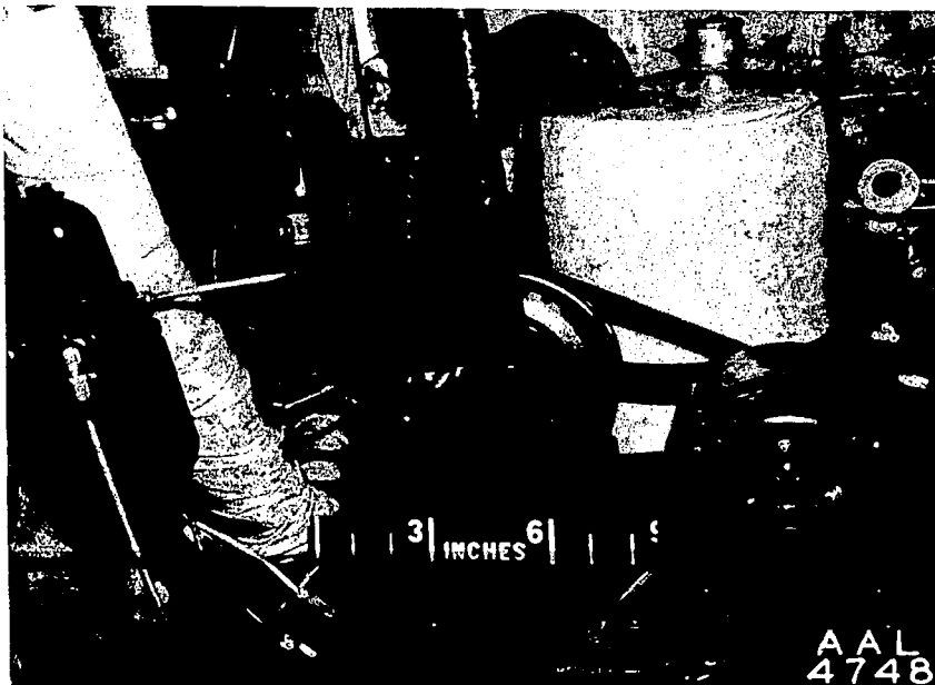
Figure 4.- Water-spray and windshield alcohol-supply-system equipment in the nose compartment of the Lockheed 12A airplane.
