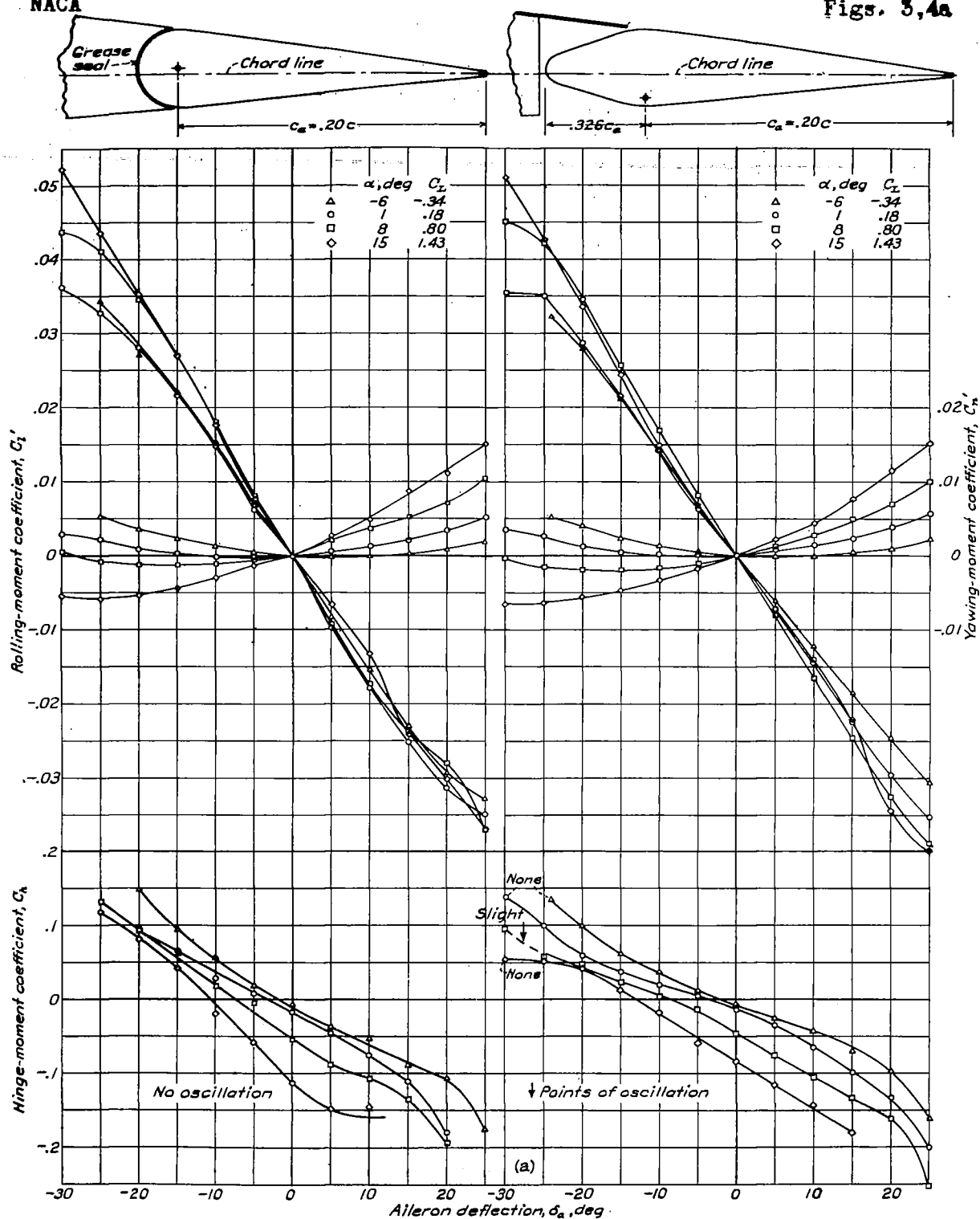
Figure 3.- Aerodynamic characteristics of a 0.20c by 0.37 b/2 plain grease-sealed aileron without balance on an NACA 23012 airfoil. V, 40 mph.
