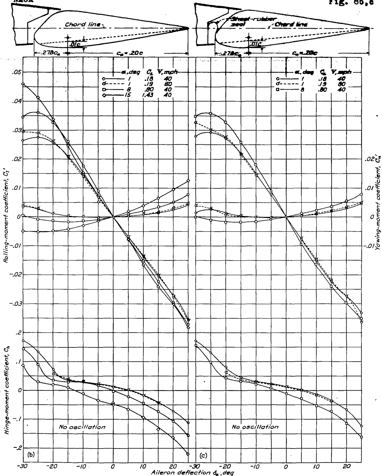
(b) No seal; 0.01c lower-surface bulge. (c) Sheet-rubber seal; 0.01c lower-surface bulge.
