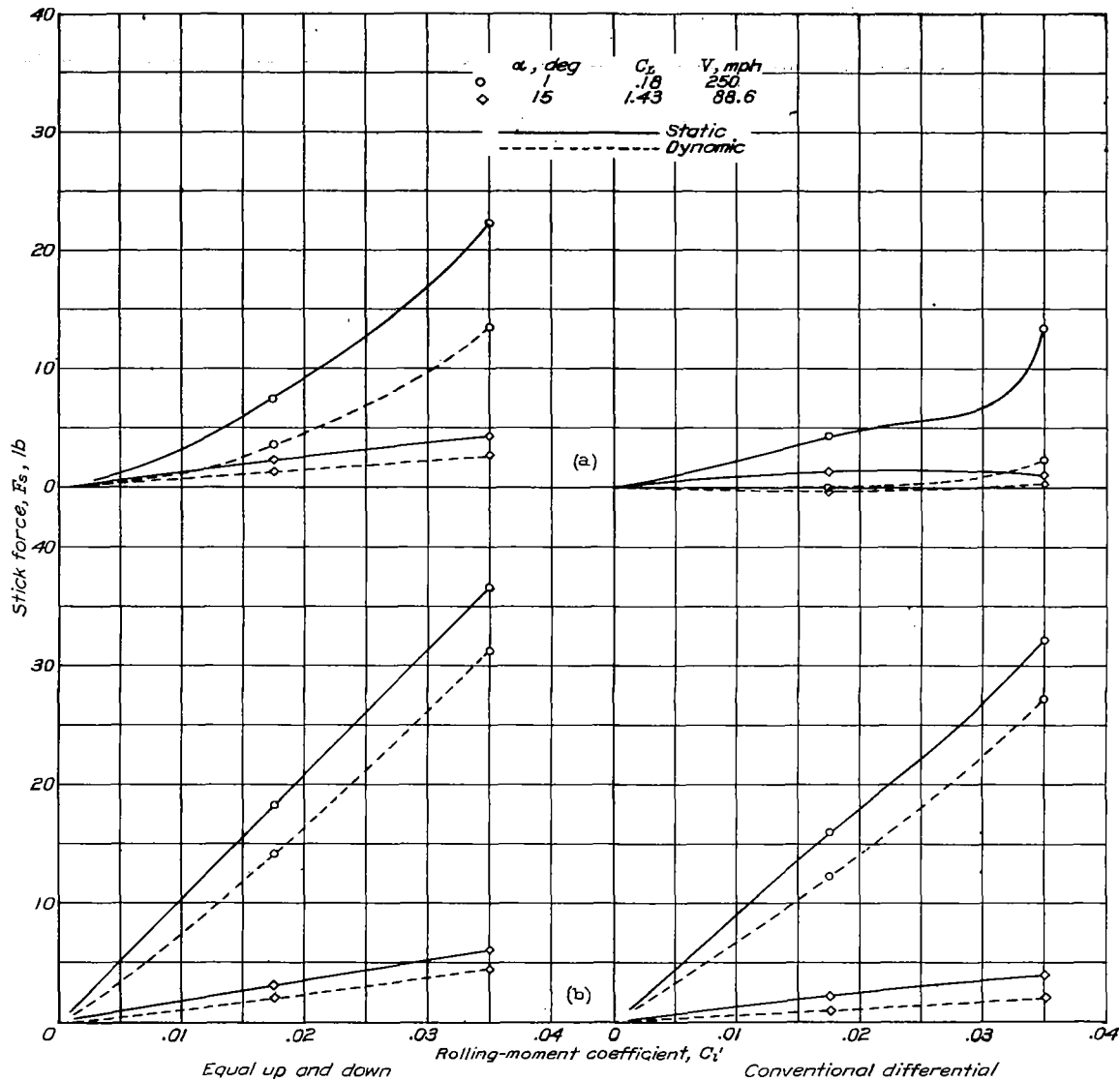
(a) Frise aileron with 0.326 c_a balance; no seal, no bulge. (b) Plain sealed aileron with 0.326 c_a balance; top cover plate only. Figures 17.- Effect of rolling on the stick-force characteristics of a pursuit airplane equipped with two arrangements of 0.20c by 0.37 b/2 ailerons and two aileron deflection systems.
