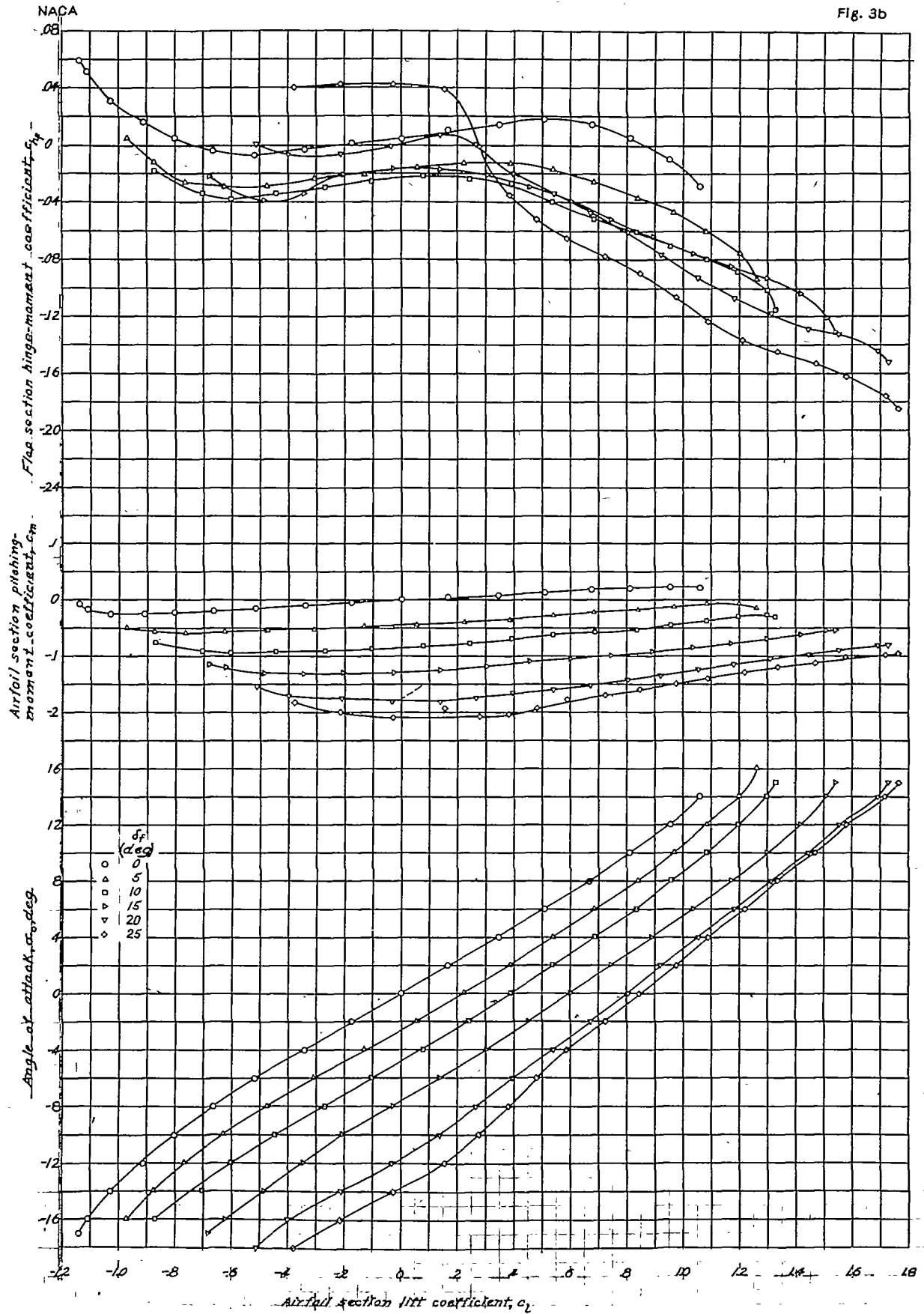
(b) 0.005c gap Figure 3. Concluded.
