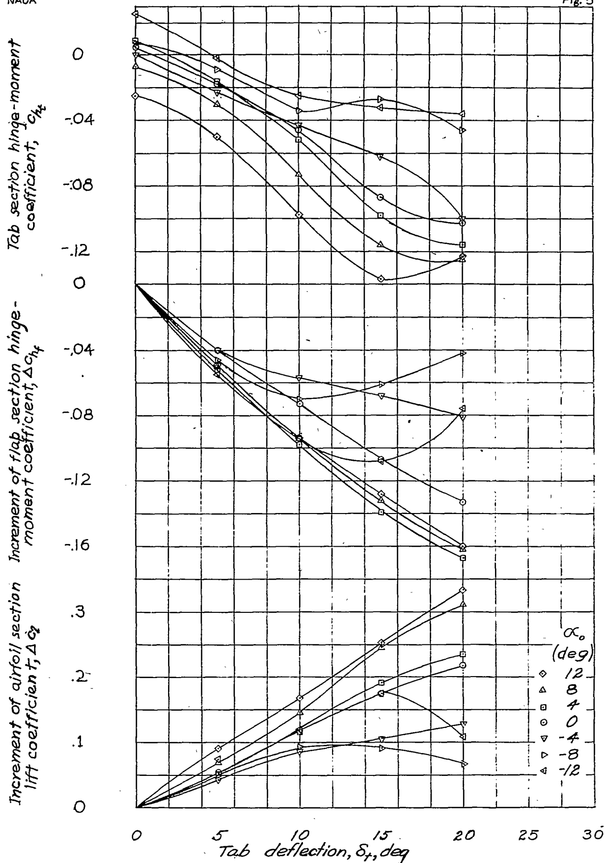
Figure 5.- Tab section hinge-moment coefficient and increments of airfoil section lift coefficient and flap section hinge-moment coefficient caused by deflection of a 6030c_f plain tab. Blunt nose 0.50c_f overhang with 0.005c flap gap and 0.001c tab gap. \delta_f = 0^\circ .
