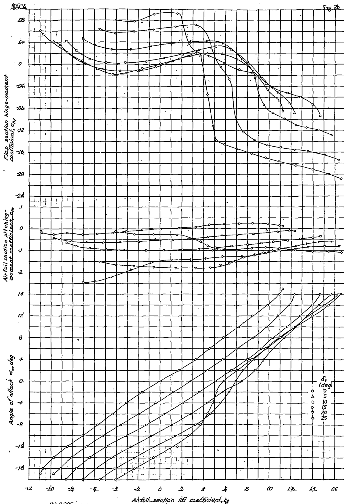
(b) 0.005c gap. Figure 2.- Concluded.
