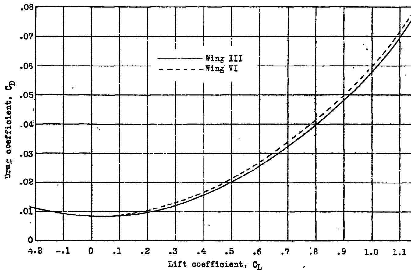
Figure 11.- Comparison of drag characteristics of wings III and VI; plain wing; R = 4,600,000 .
