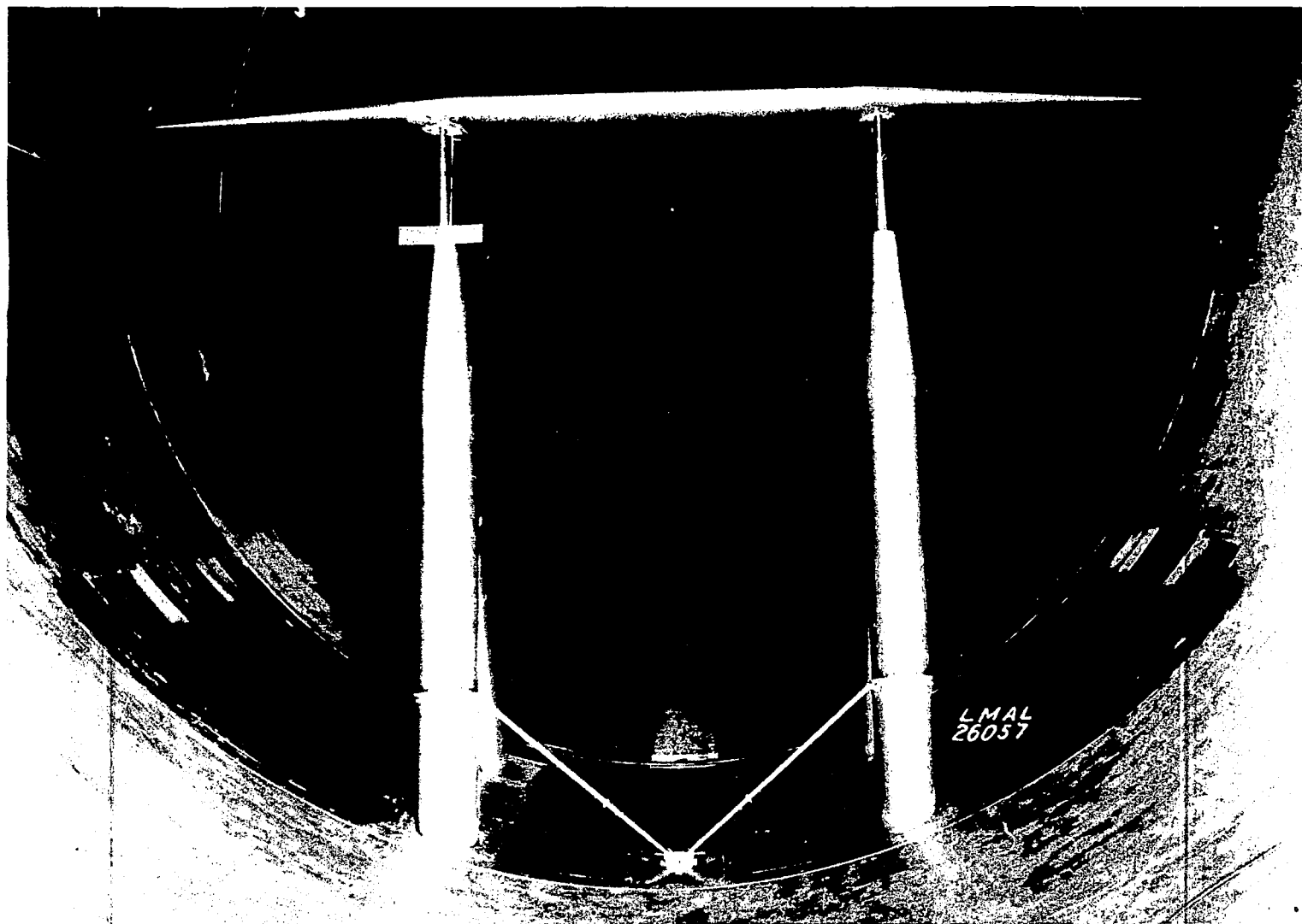
Figure 3.- Wing VI mounted in the 19-foot pressure tunnel.
