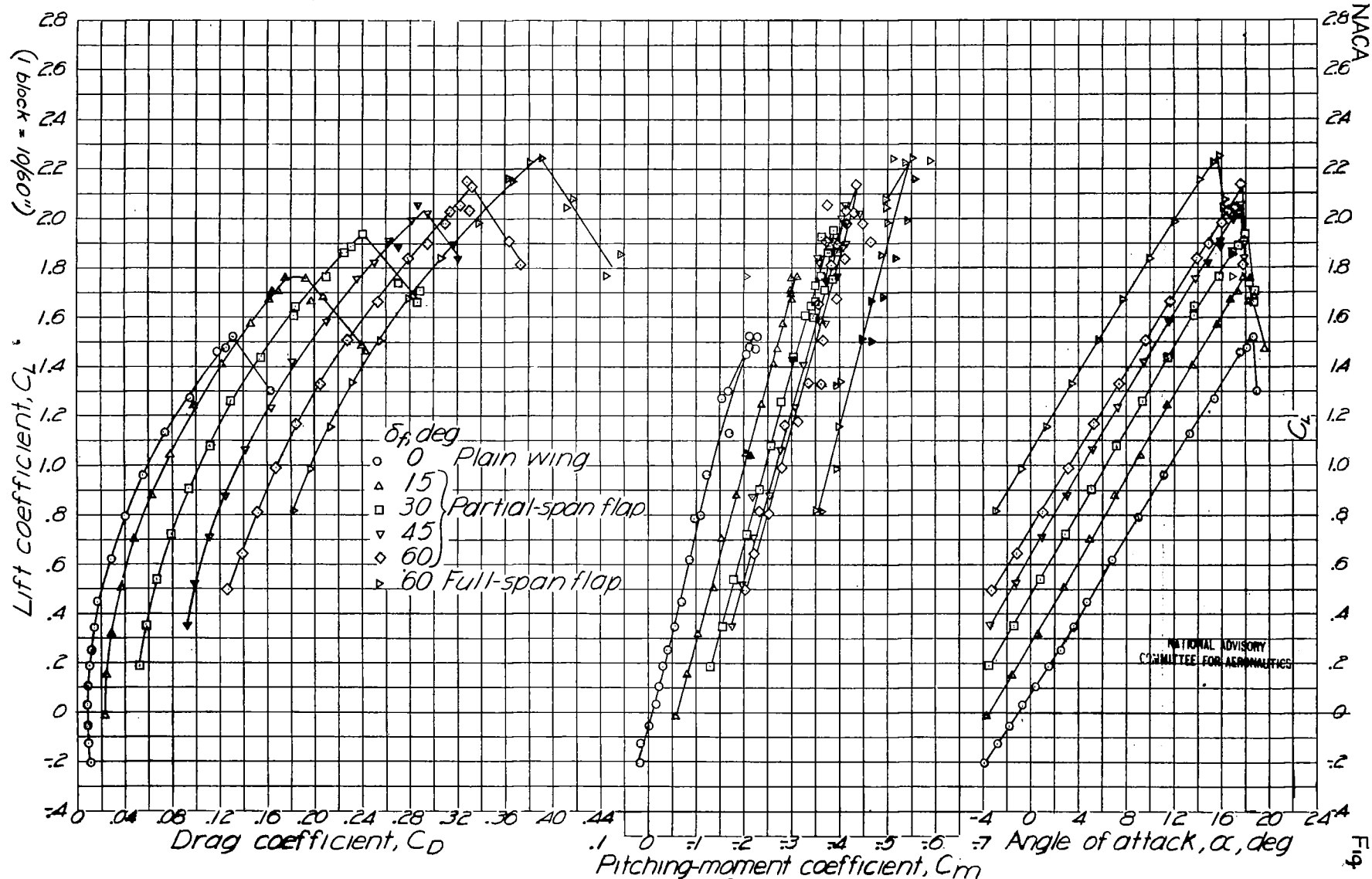
Figure 5.-Aerodynamic characteristics of wing VI with 0.20c split flaps. R=4,600,000 .
