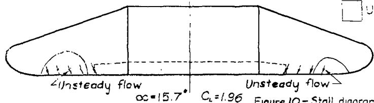
Figure 10.- Stall diagrams of an NACA 230 series tapered wing III with a 0.20-chord partial-span split flap: \delta_f = 60^\circ ; R = 4,500,000 .
