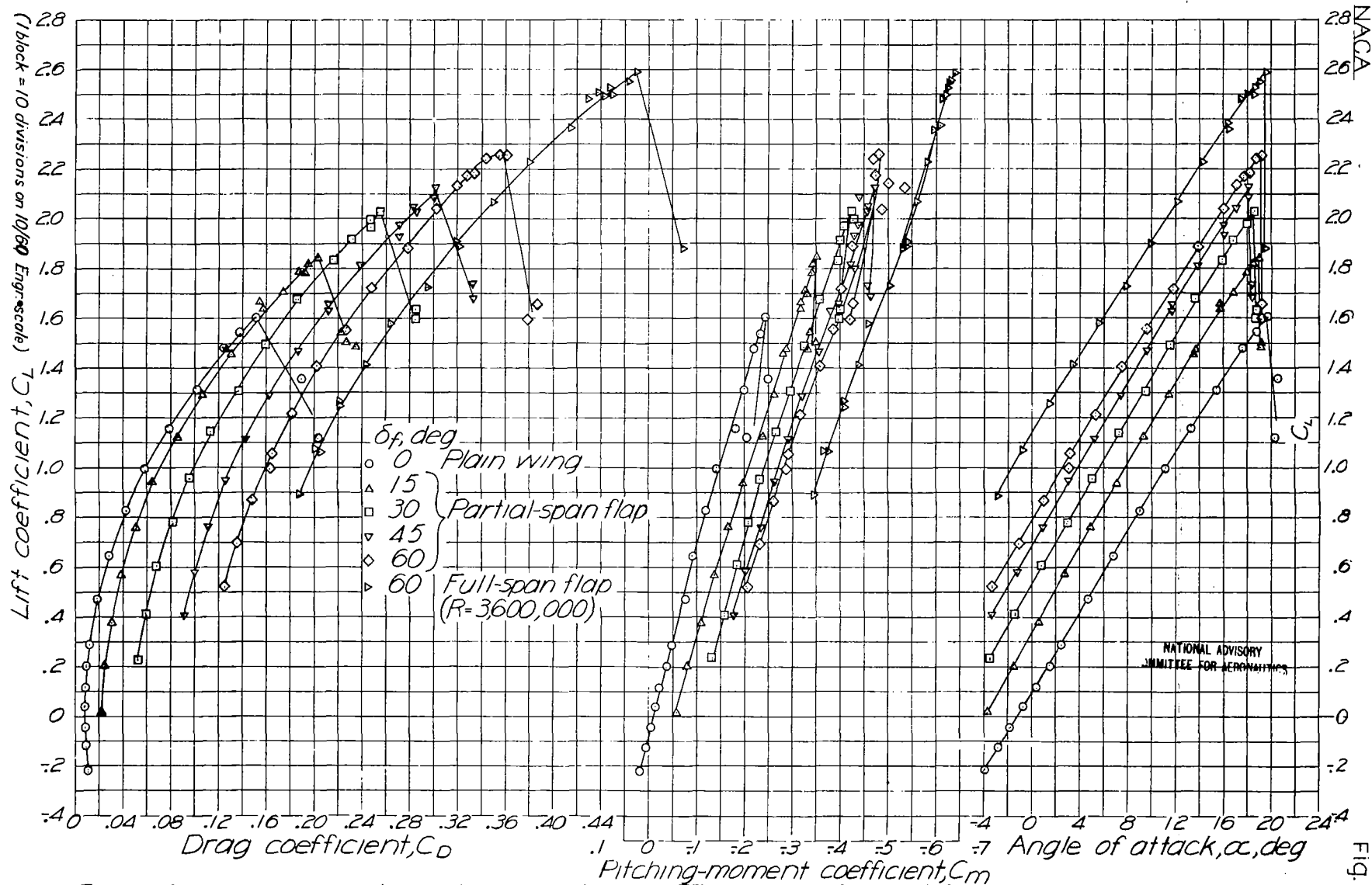
Figure 4.-Aerodynamic characteristics of wing III with 0.20c split flaps. R=4,600,000 .
