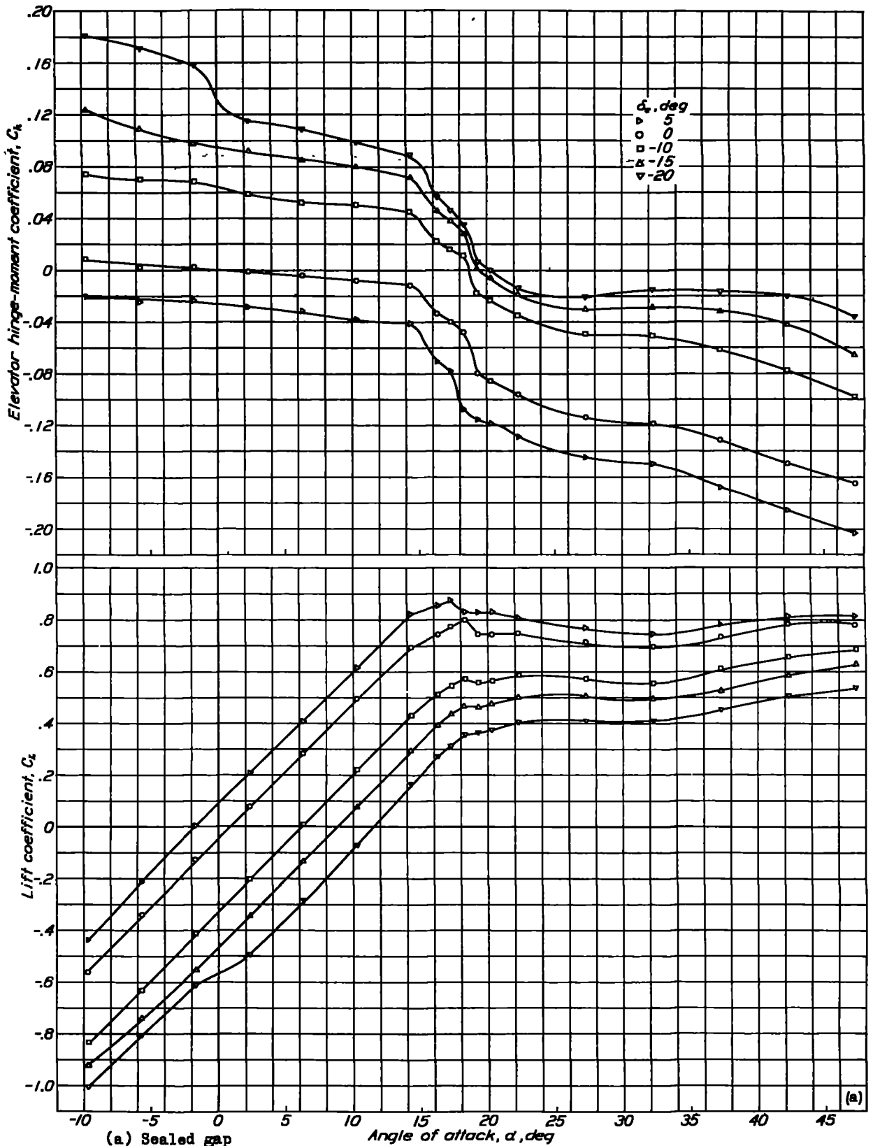
(a) Sealed gap Figure 6(a,b).- Lift and elevator hinge-moment coefficients as functions of angle of attack at various elevator deflections for fuselage and horizontal tail combination. Balanced elevator with 0.35c_o sharp nose overhang.
