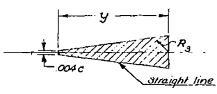
Elevator nose sharp
