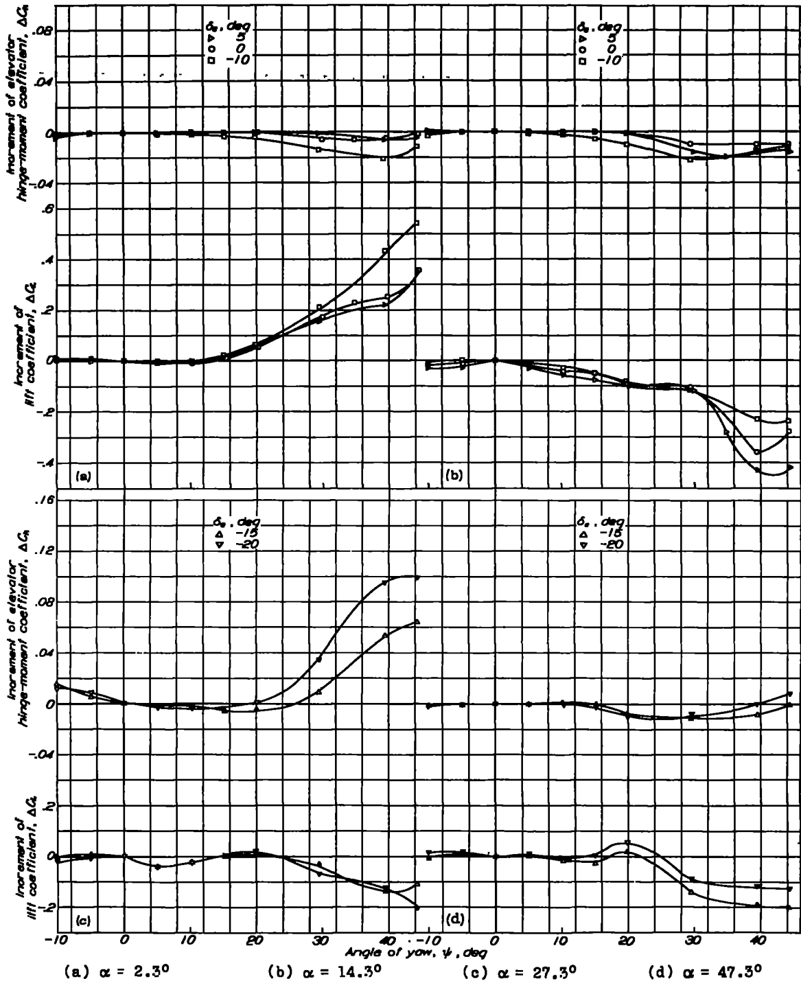
Figure 12.- Increments of lift and elevator hinge-moment coefficients due to angle of yaw as function of angle of yaw at various angles of attack and elevator deflections. Balanced elevator with 0.50c_e blunt nose overhang and sealed gap.
