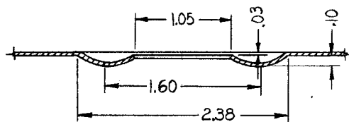
Figure 1.- Typical cross sections of flanges and beads.
