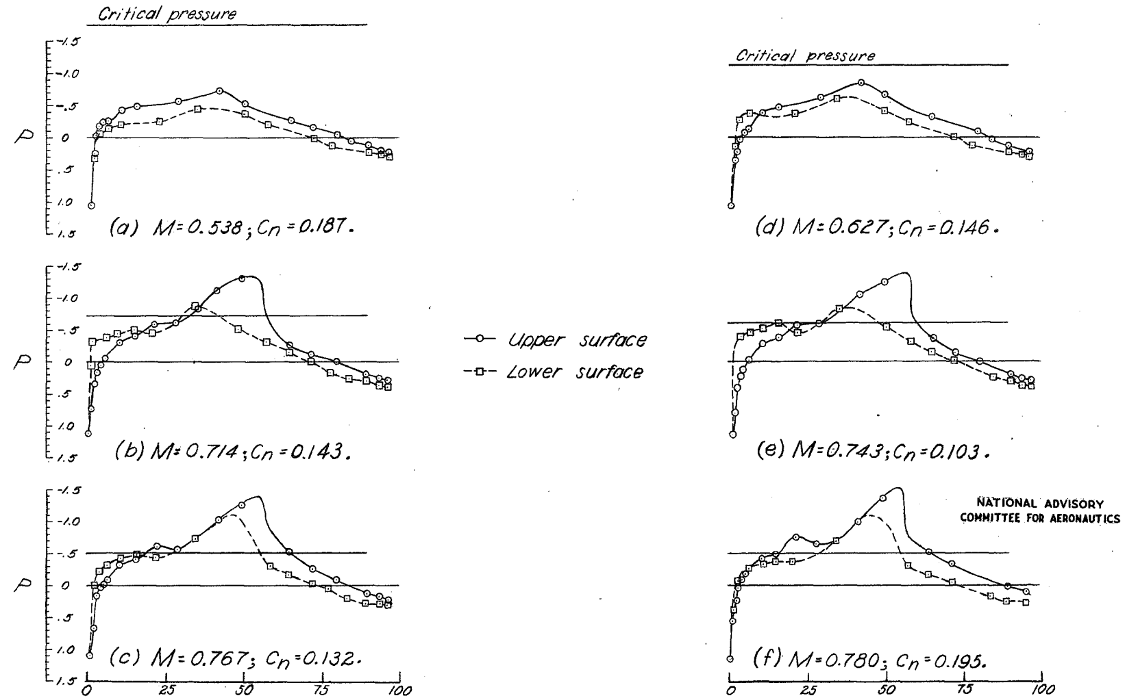
Figure 6.— Pressure distributions corresponding to wake distributions of figure 5. 0.1 < C_n < 0.2 .
