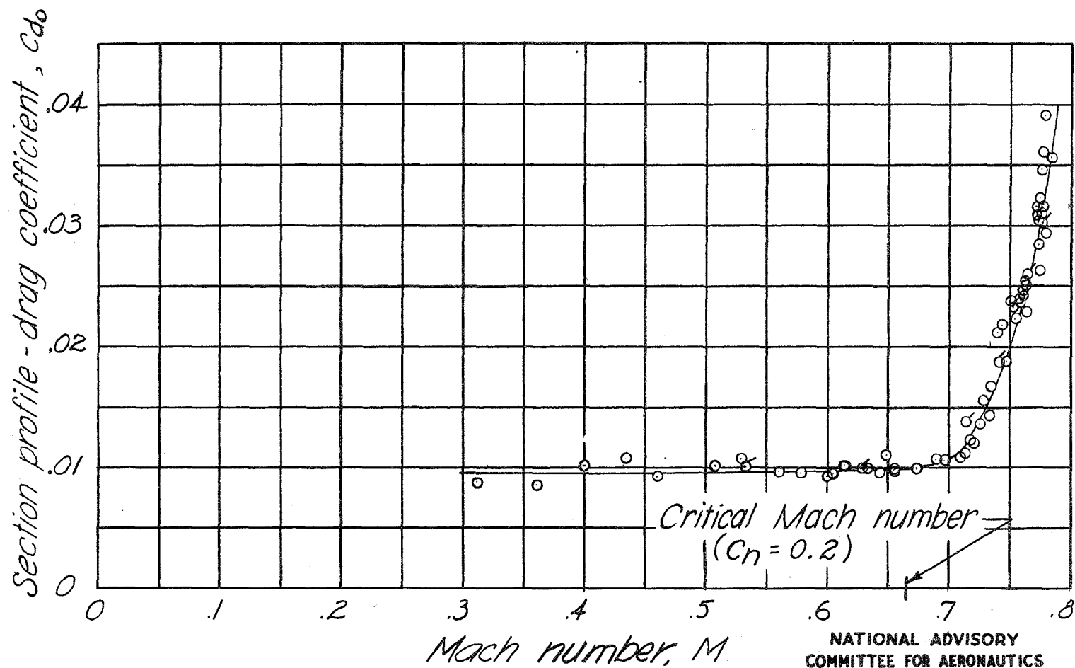
Figure 7. - Variation of section profile-drag coefficient with Mach number at semispan station. 0 < C_n < 0.4 . Symbols with tails attached represent points from figure 5.
