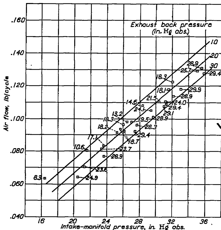
FIGURE 9.—Variation of air flow with intake-manifold pressure and exhaust back pressure at constant engine speed for 14-cylinder engine of 2600-cubic-inch displacement. Engine speed, 2000 rpm; air flow corrected to intake-manifold temperature of 100° F. (Numerical values are exhaust back pressures, in. Hg absolute.)
