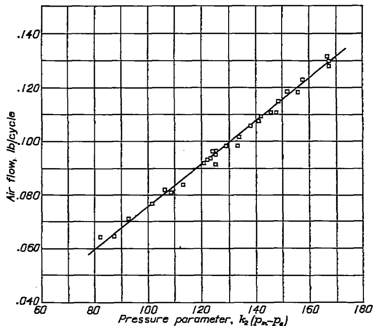
FIGURE 10.—Variation of air flow with pressure parameter for 14-cylinder engine of 2600-cubic-inch displacement. Engine speed, 2000 rpm; air flow corrected to intake-manifold temperature of 100° F.
