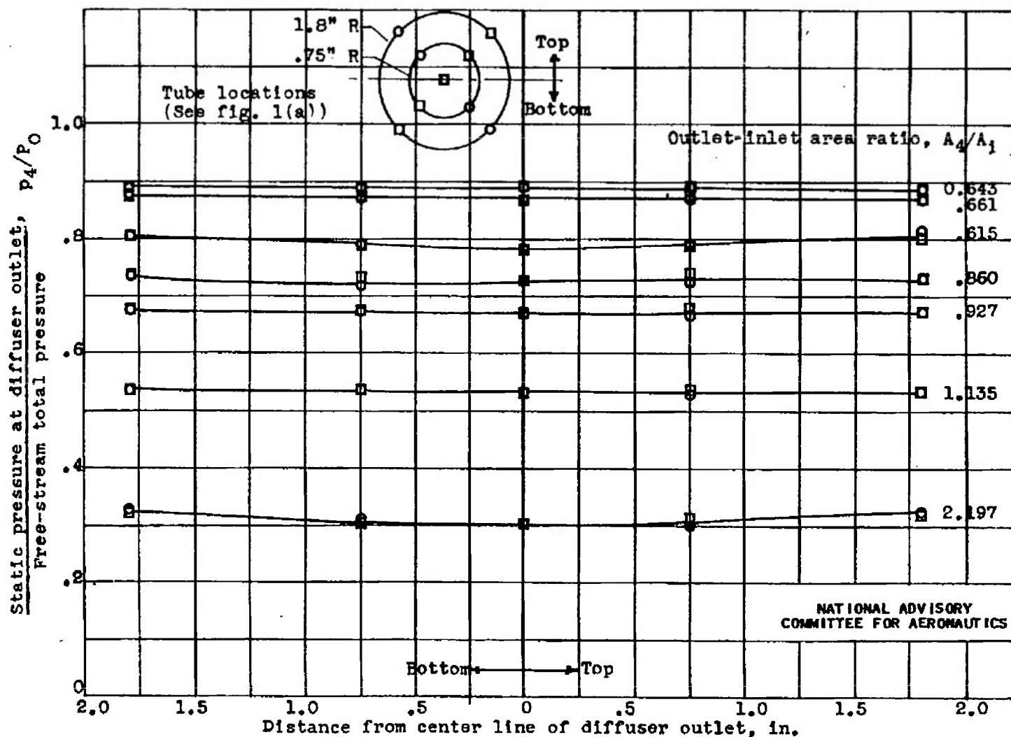
(c) Static-pressure distribution at 5^\circ angle of attack.
