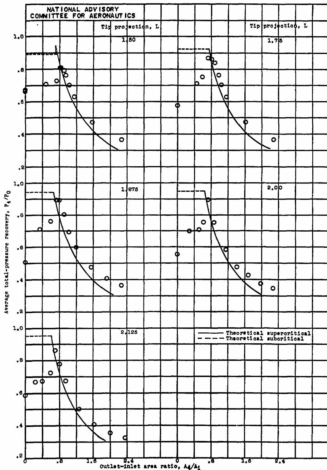
(b) 20-40 cones; curved inlet. Figure 7.- Continued. Variation of total-pressure recovery with outlet-inlet area ratio at angle of attack of 0^\circ .
