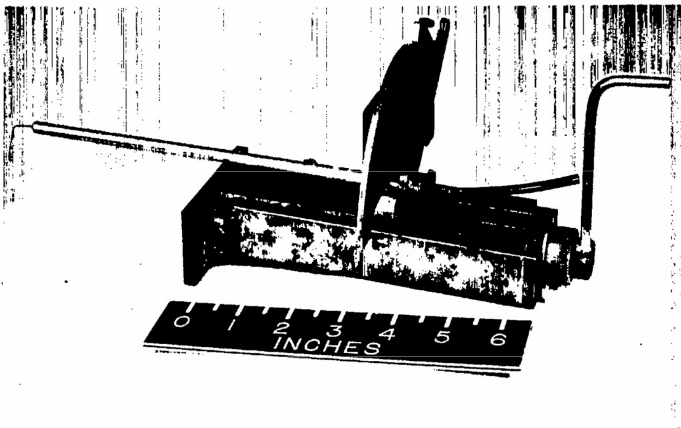
Figure 6.- Typical micrometer survey tube.
