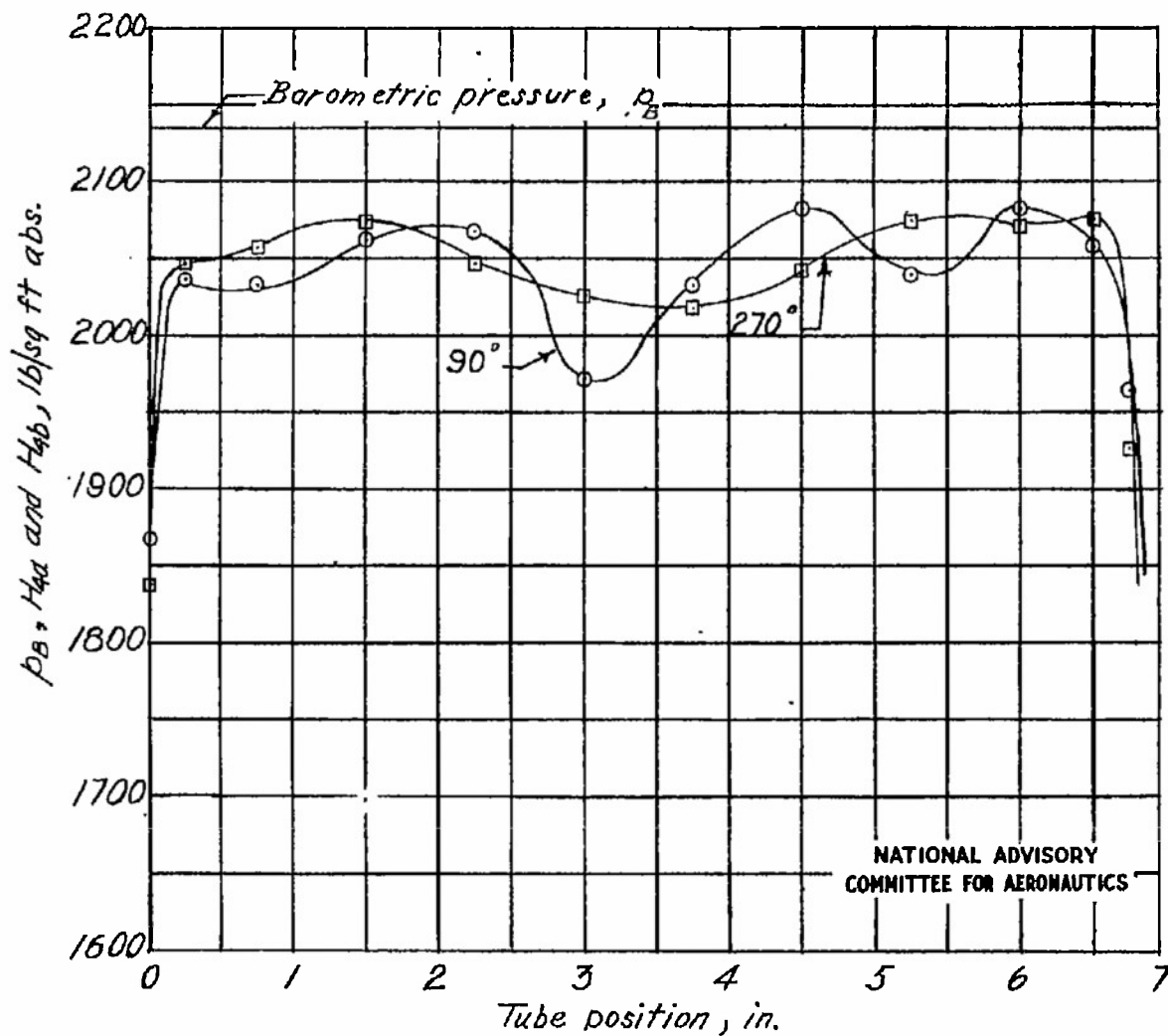
(e) Circumferential position, 90° and 270°; weight flow, 89.63 pounds per second. (Note that vertical scale changes from that on previous figures.)
