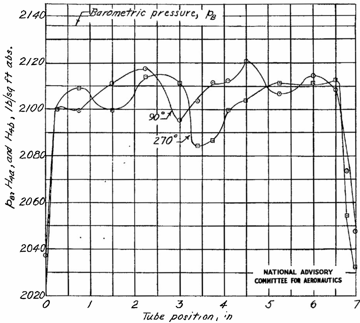
(d) Circumferential position, 90° and 270°; weight flow, 60.46 pounds per second.
