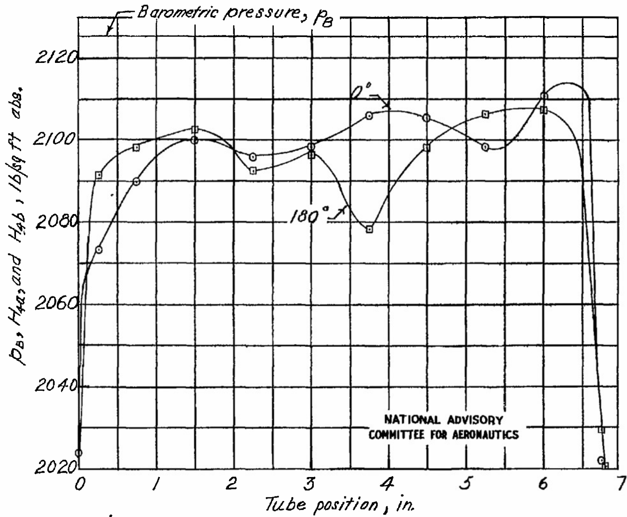
(c) Circumferential position, 0° and 180°; weight flow, 59.35 pounds per second.
