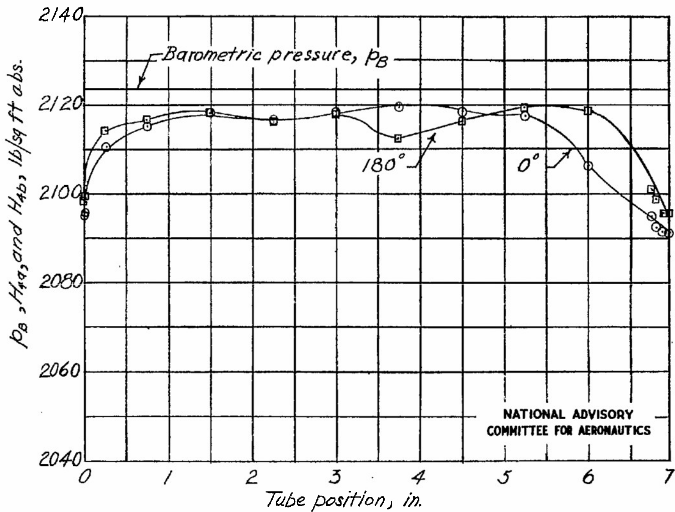
(a) Circumferential position, 0^\circ and 180^\circ ; weight flow, 29.67 pounds per second.
