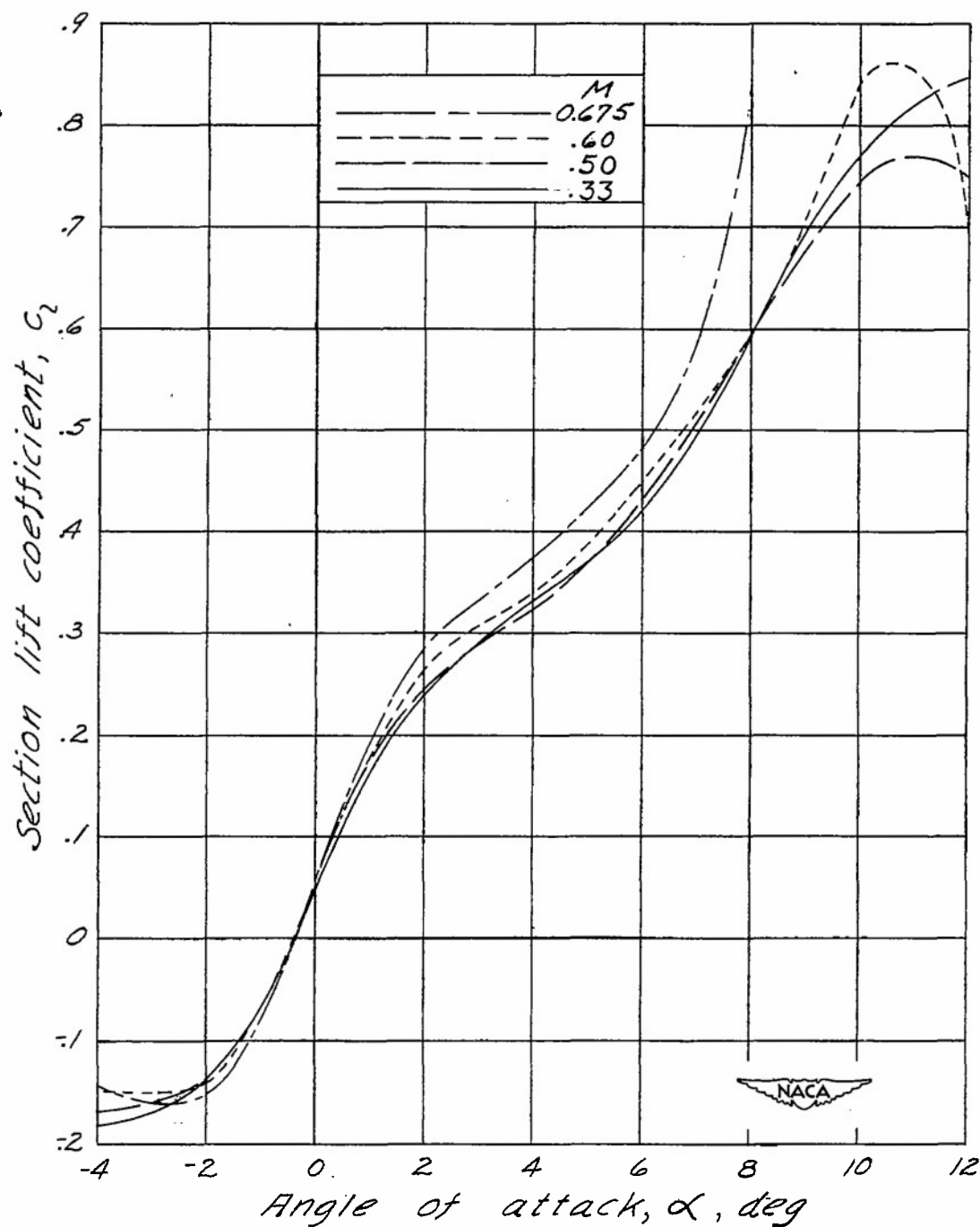
Figure 21 .- Variation of section lift coefficient with angle of attack for the NACA 16-115 airfoil. Data from Langley 24-inch high-speed tunnel.
