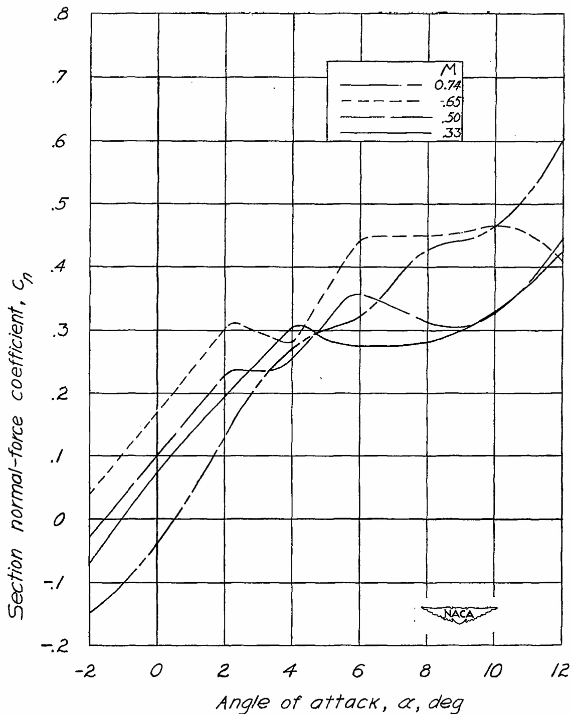
Figure 19.- Variation of section normal-force coefficient with angle of attack. NACA 16-025 airfoil.
