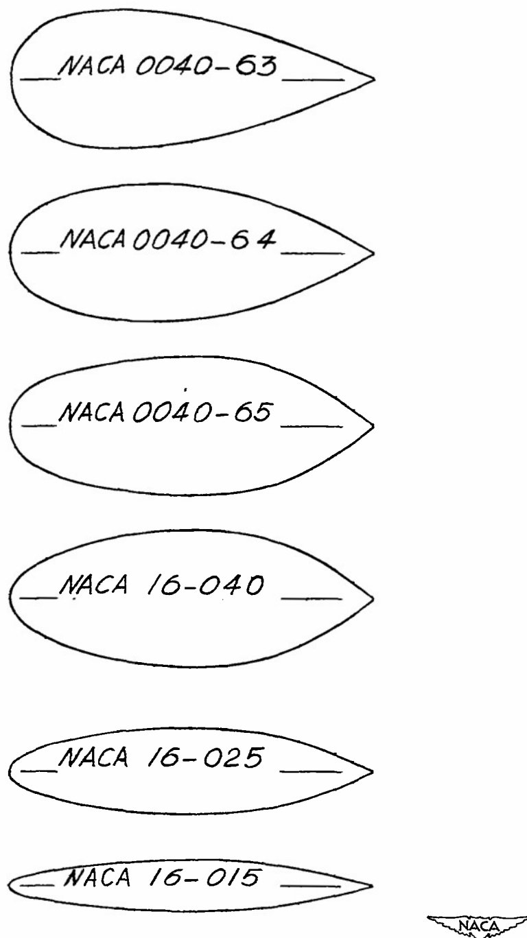
Figure 2 .- Profiles of airfoils tested in the Langley rectangular high-speed tunnel.
