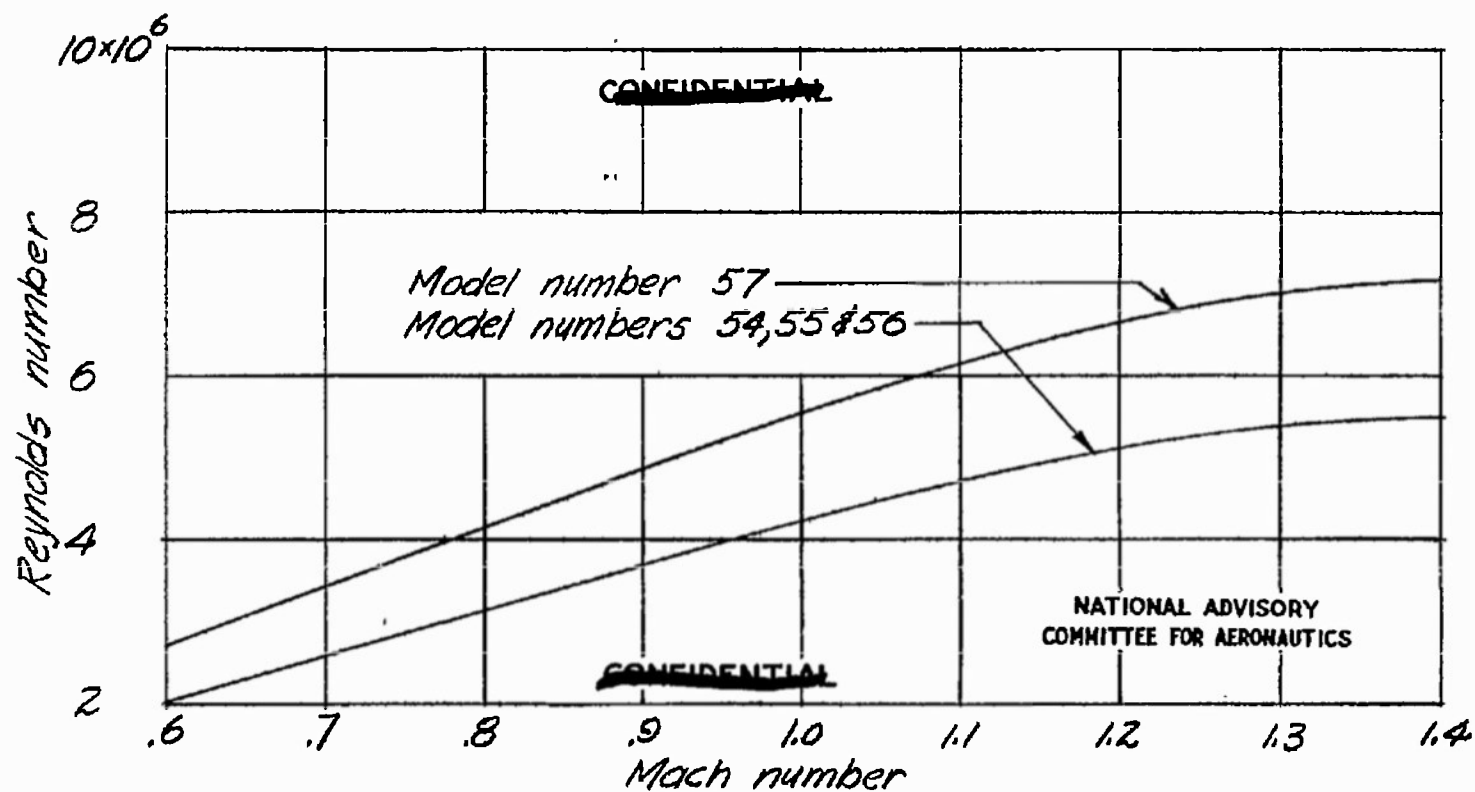
Figure 3.- Typical variation of Reynolds number with Mach number.
