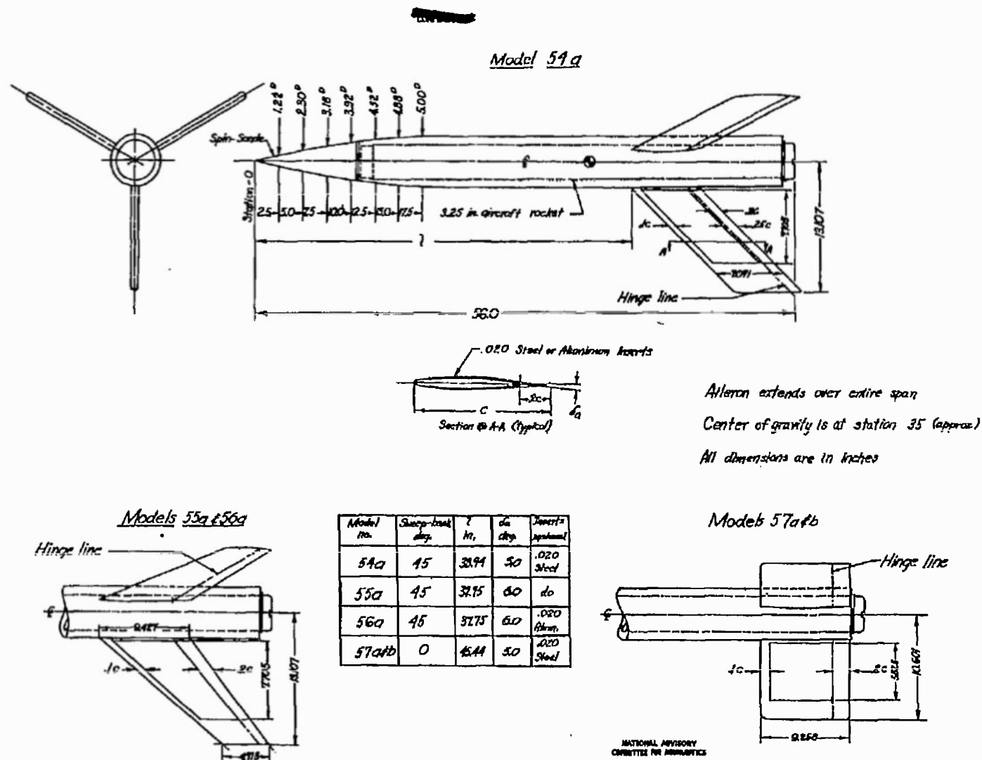
Figure 1.-General arrangement of RM-5 Models.
