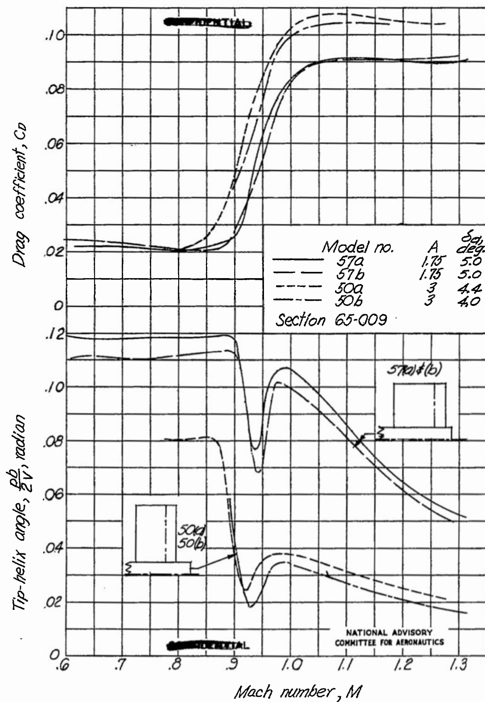
Figure 7.-Effect of aspect ratio on the variation of tip-helix angle and drag coefficient with Mach number. \Lambda = 0^\circ ; \lambda = 1.0 . Data for models 50(a) and 50(b) from reference 1.
