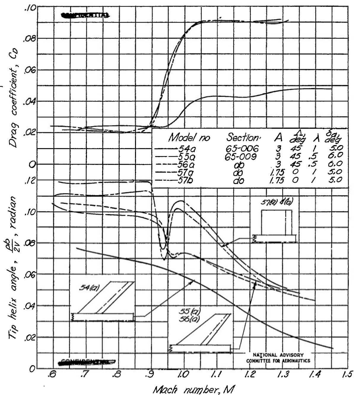
Figure 5.-Variation of tip helix angle and drag coefficient with Mach number for models of present investigation.
