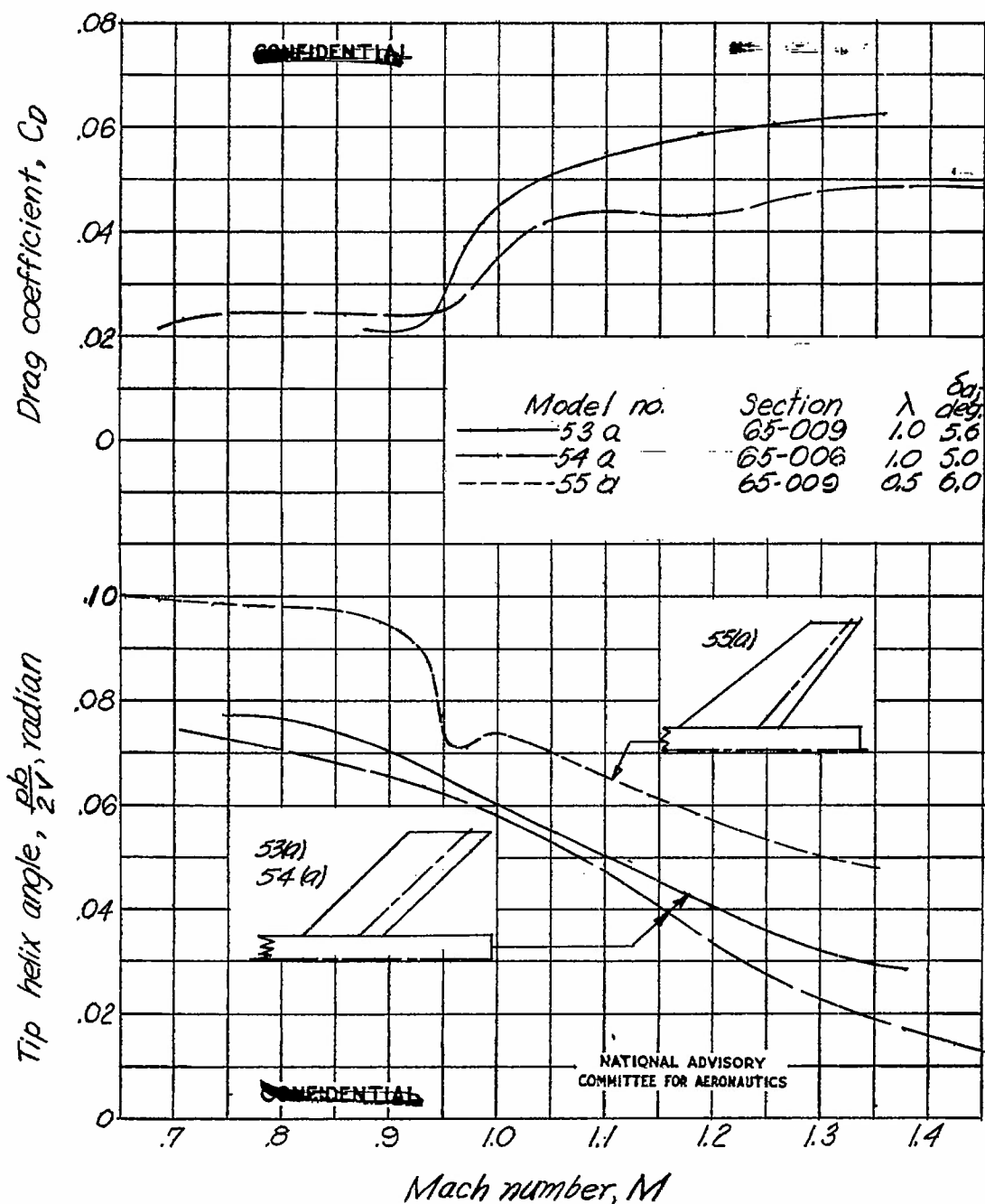
Figure 6 .- Effect of thickness and taper on the variation of tip helix angle and drag coefficient with Mach number. A=3.0 ; \Lambda=45 deg. Data for model 53a from reference 1.
