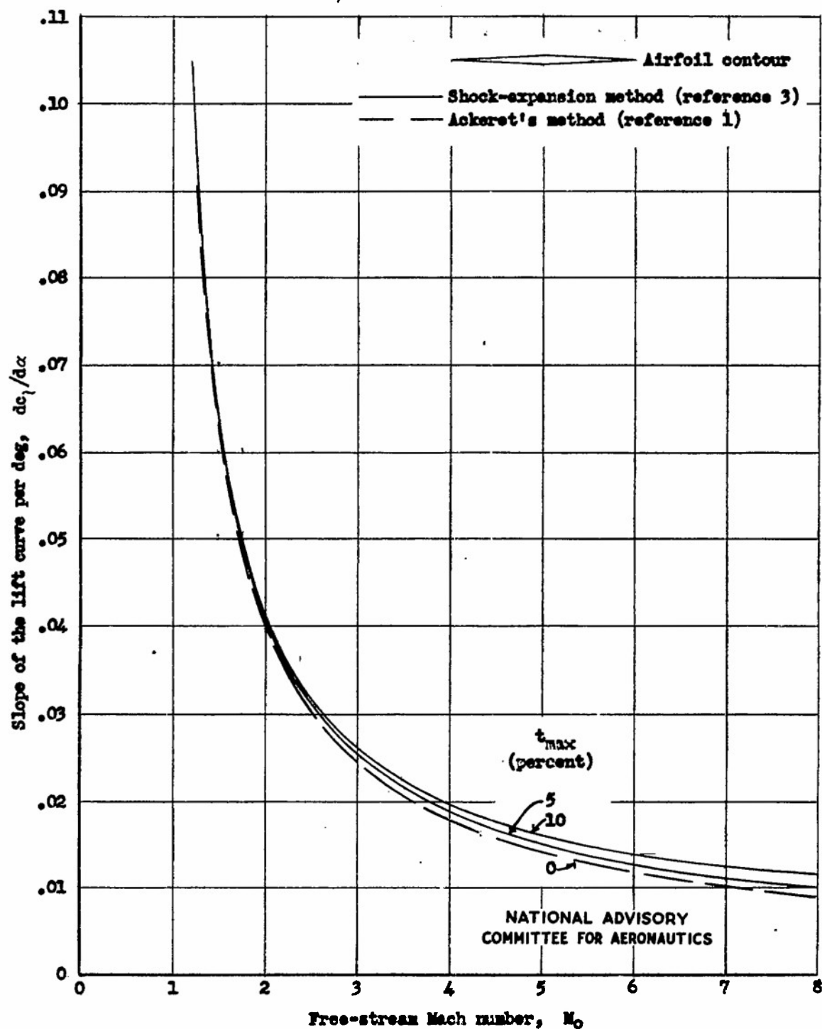
Figure 6.- Slope of lift curve of uncambered thin airfoil at supersonic speeds. t_{max} at midchord; \alpha = 0^\circ ; c_0 = 0 .
