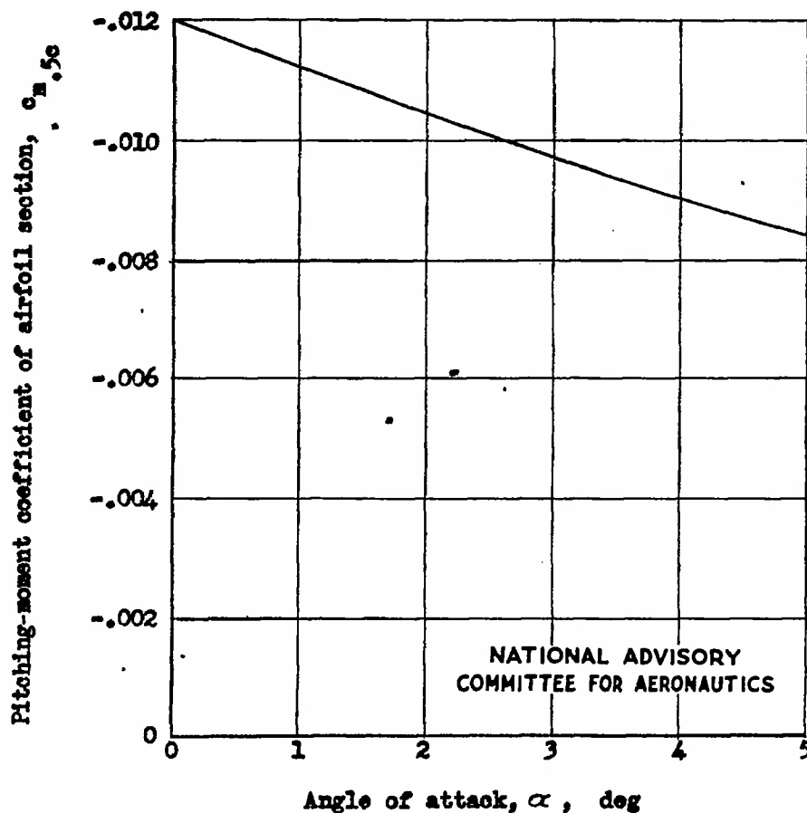
Figure 14.- Effect of angle of attack of airfoil section on section pitching-moment coefficient with 20 percent chord aileron deflected 10^\circ at M_0 = 4 . t_{max} at midchord, 5 percent; camber, 0.
