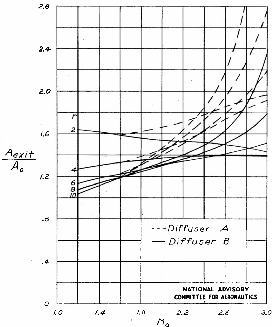
Figure 12.- Ratio of exhaust - nozzle exit area to air-inlet area as a function of free - stream Mach number. Altitude, stratosphere.
