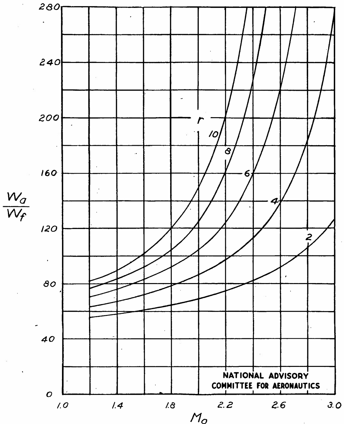
Figure 4.- Air-fuel ratio of turbojet system as a function of free-stream Mach number. Altitude, stratosphere; maximum temperature, 1500^{\circ}\text{F} .
