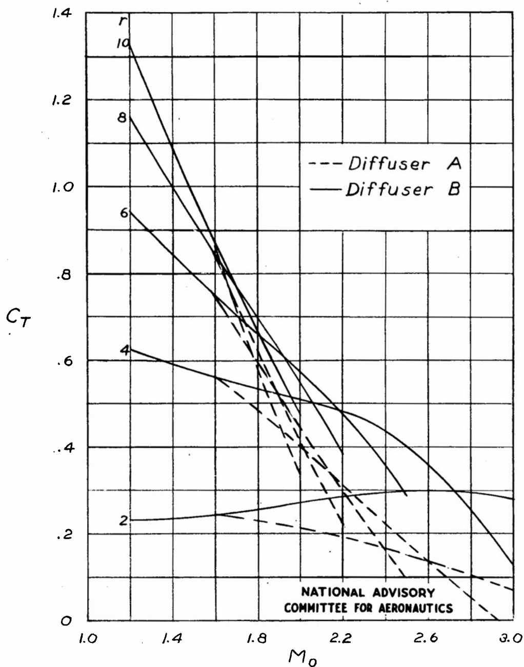
Figure 13.-Thrust coefficient as a function of free-stream Mach number. Altitude, stratosphere.
