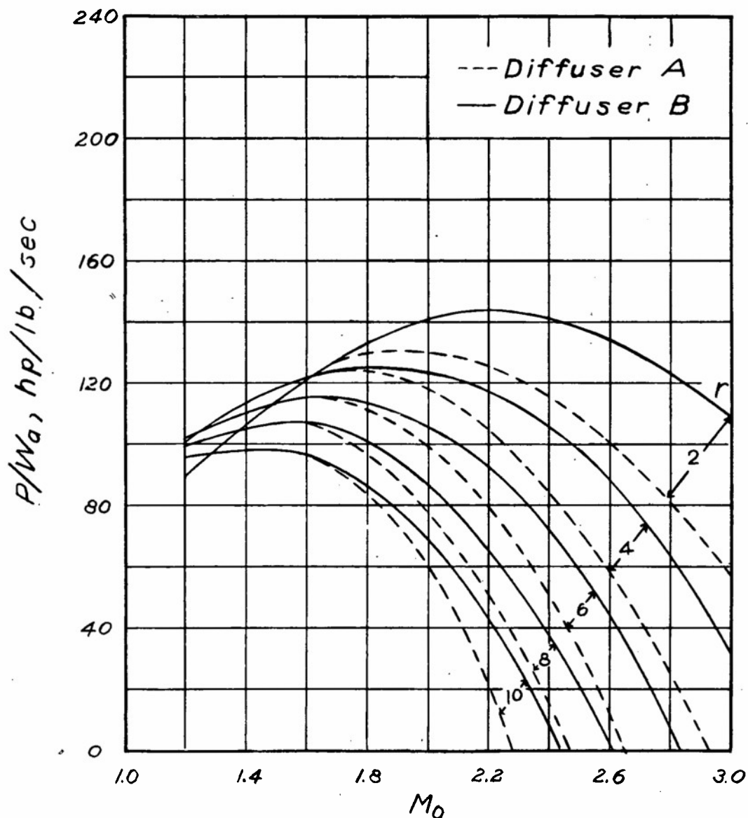
Figure 5.- Thrust power per pound of air per second as a function of free-stream Mach number. Altitude, stratosphere.
