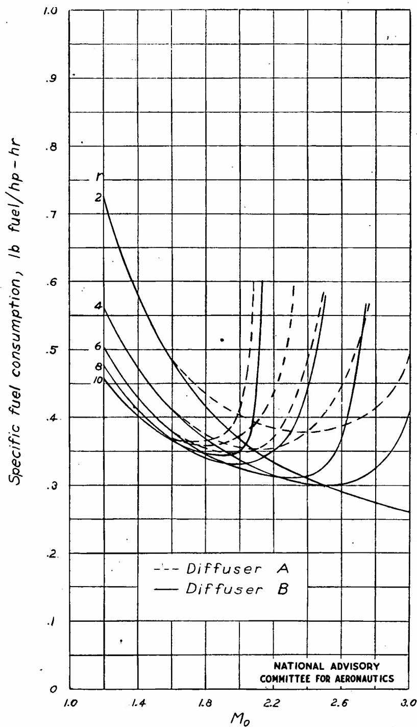
Figure 7.- Specific fuel consumption, pounds fuel per horsepower-hour, as a function of free-stream Mach number. Altitude, stratosphere.
