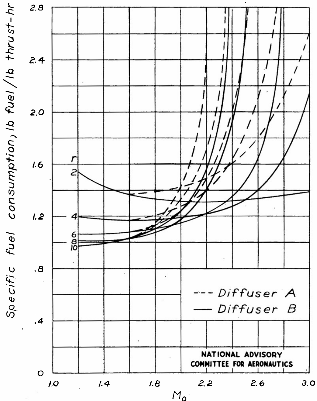
Figure 6.- Specific fuel consumption, pounds fuel per hour per pound thrust, as a function of free-stream Mach number. Altitude, stratosphere.
