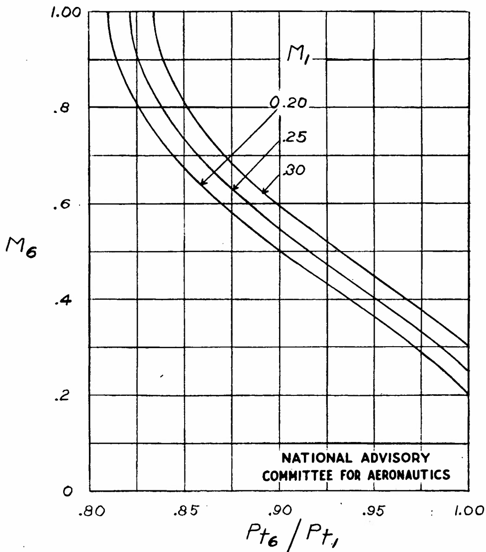
Figure 21. — Mach number following combustion as a function of the total-pressure ratio across the combustion chamber.
