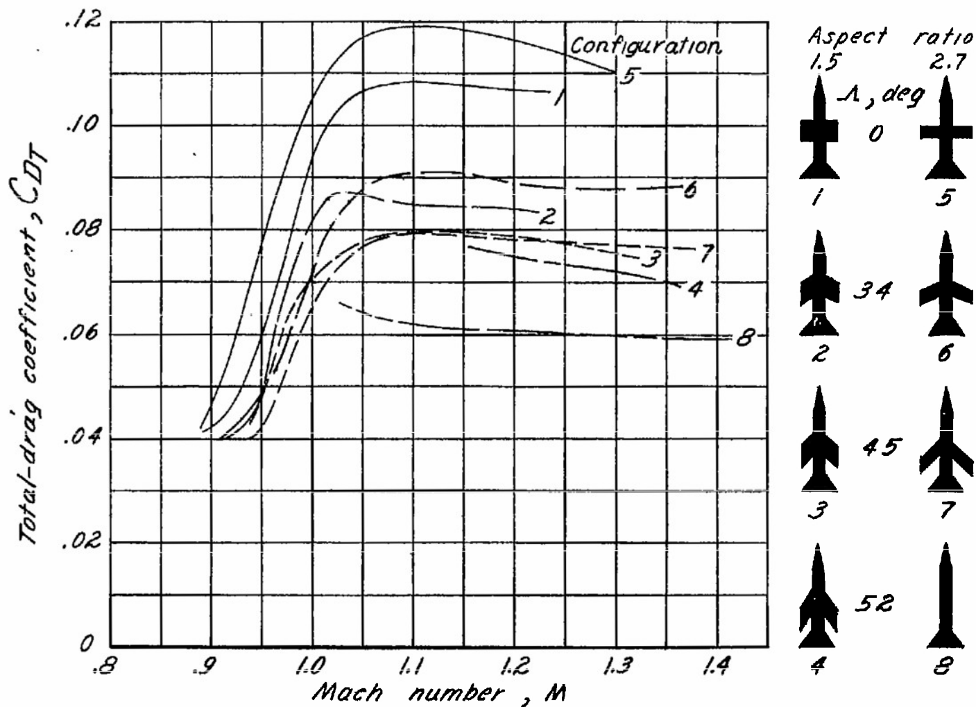
(a) Total-drag coefficient. Figure 9.- Effect of sweepback angle and aspect ratio on total-drag coefficient and wing-drag coefficient.
