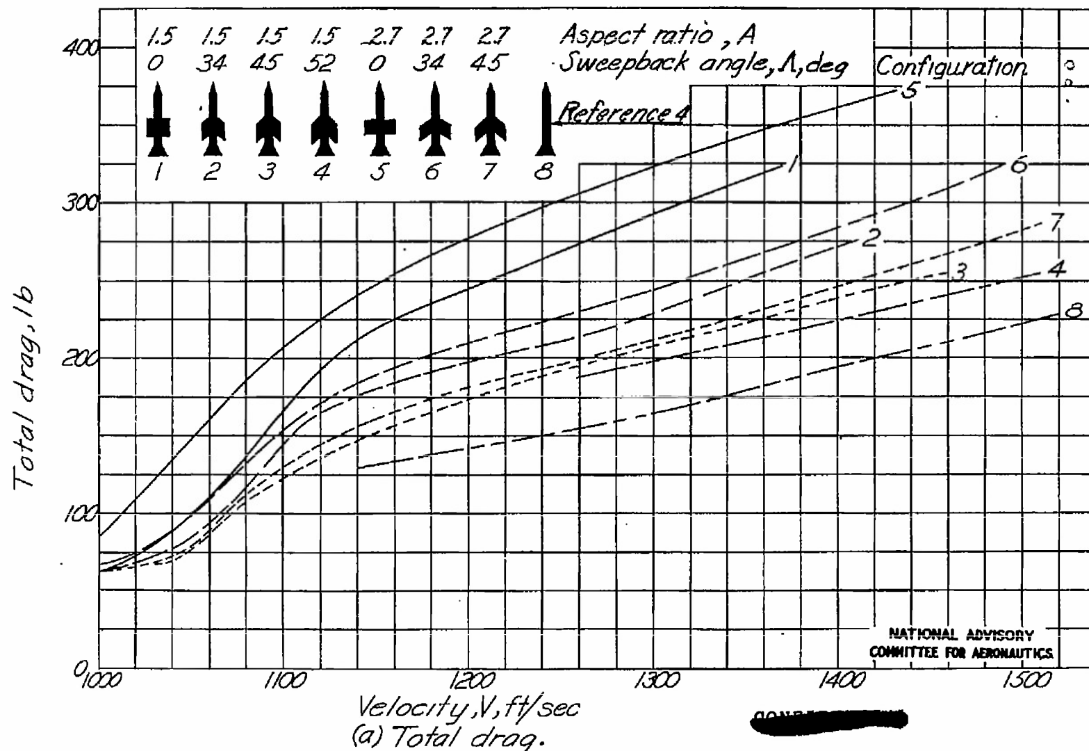
Figure 7.-Curves of total drag and wing drag for the sweepback angles and aspect ratios investigated.
