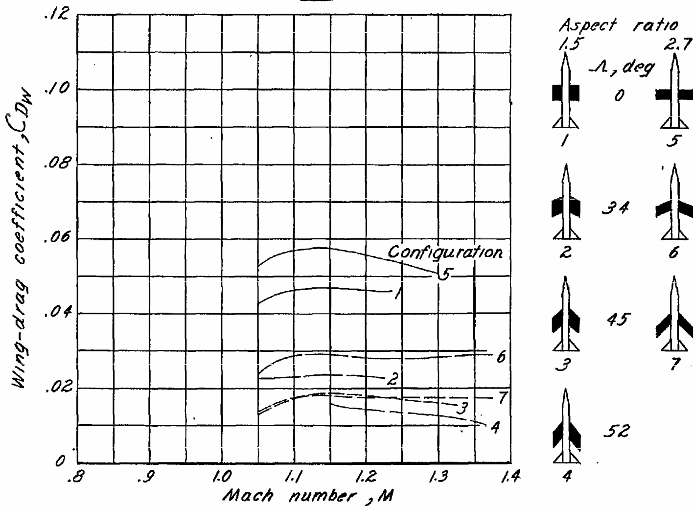
(b) Wing-drag coefficient. Figure 9. - Concluded.
