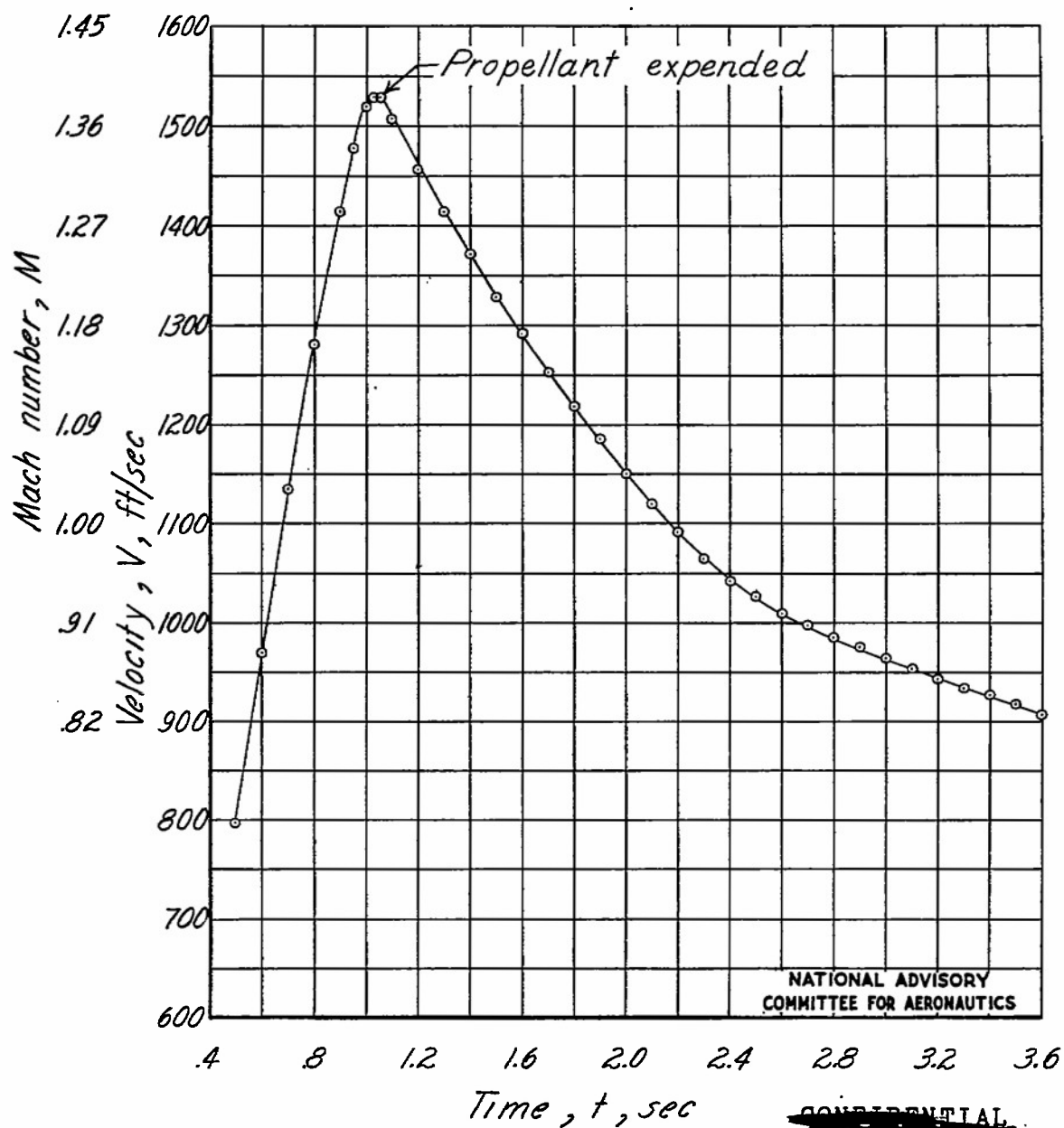
Figure 6.- Typical velocity-time curve.
