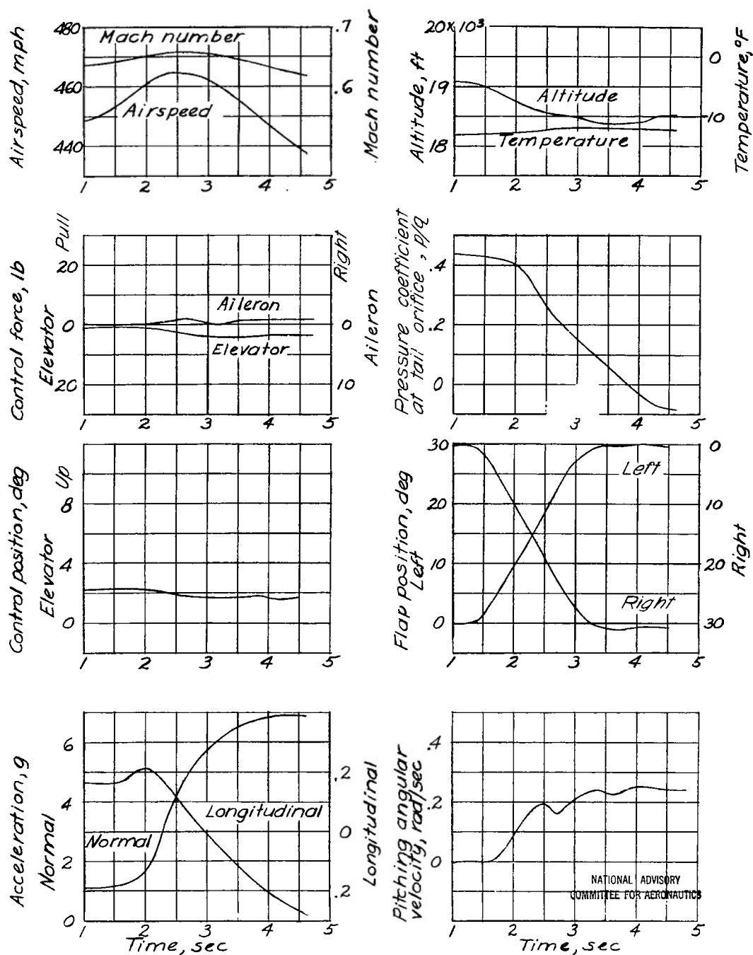
Figure 9.- Variation of basic measured quantities during dive-recovery-flap deflection. Dive-recovery-flap deflection, 30°; weight, 7750 pounds; center-of-gravity position, 28.05 percent mean aerodynamic chord.
