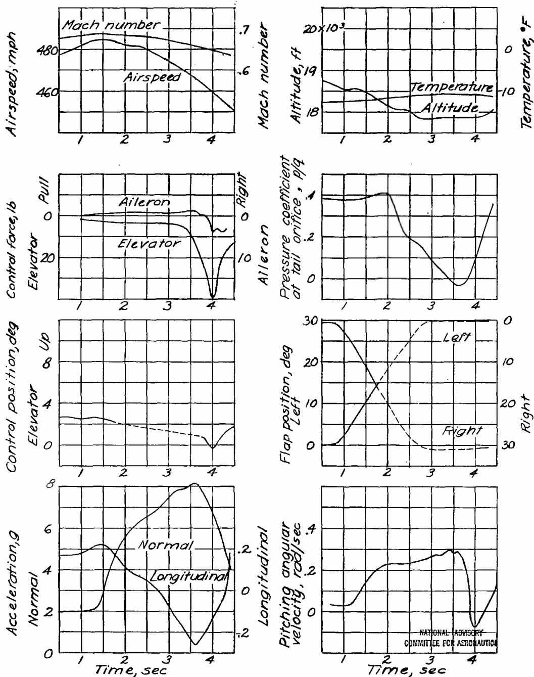
Figure 10.- Variation of basic measured quantities during dive-recovery-flap deflection. Dive-recovery-flap deflection, 30°; weight, 7630 pounds; center-of-gravity position, 27.73 percent mean aerodynamic chord.
