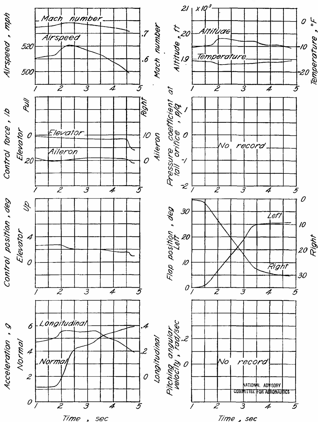
Figure 5.- Variation of basic measured quantities during dive-recovery-flap deflection. Dive-recovery-flap deflection, 30°; weight, 7850 pounds; center-of-gravity position, 28.63 percent mean aerodynamic chord.
