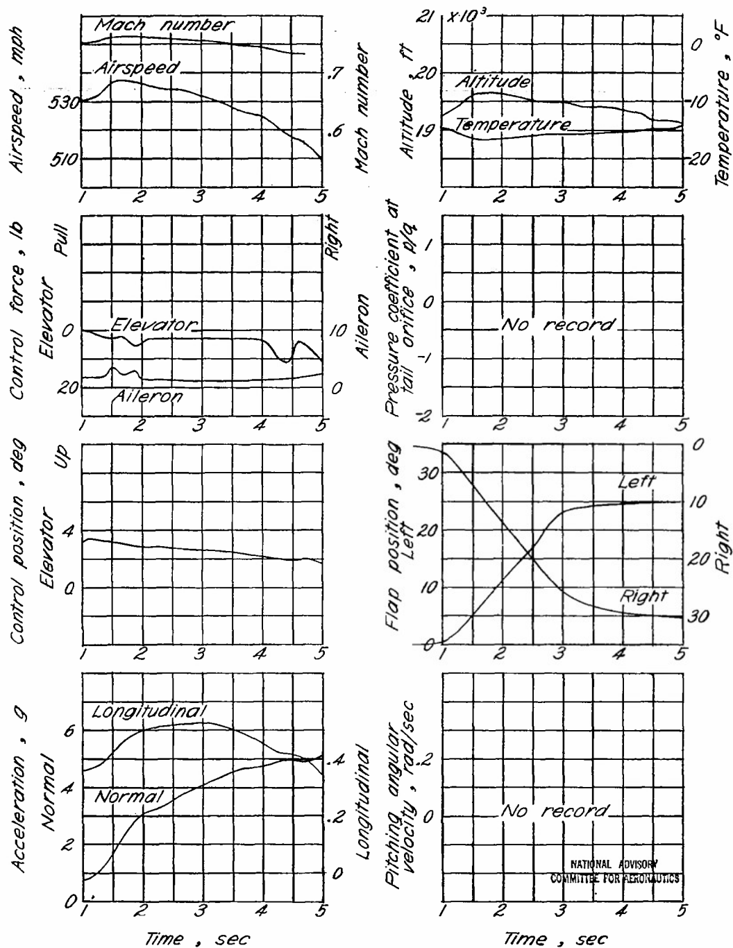
Figure 6.- Variation of basic measured quantities during dive-recovery-flap deflection. Dive-recovery-flap deflection, 30 ^{\circ} ; weight, 7810 pounds; center-of-gravity position, 28.55 percent mean aerodynamic chord.
