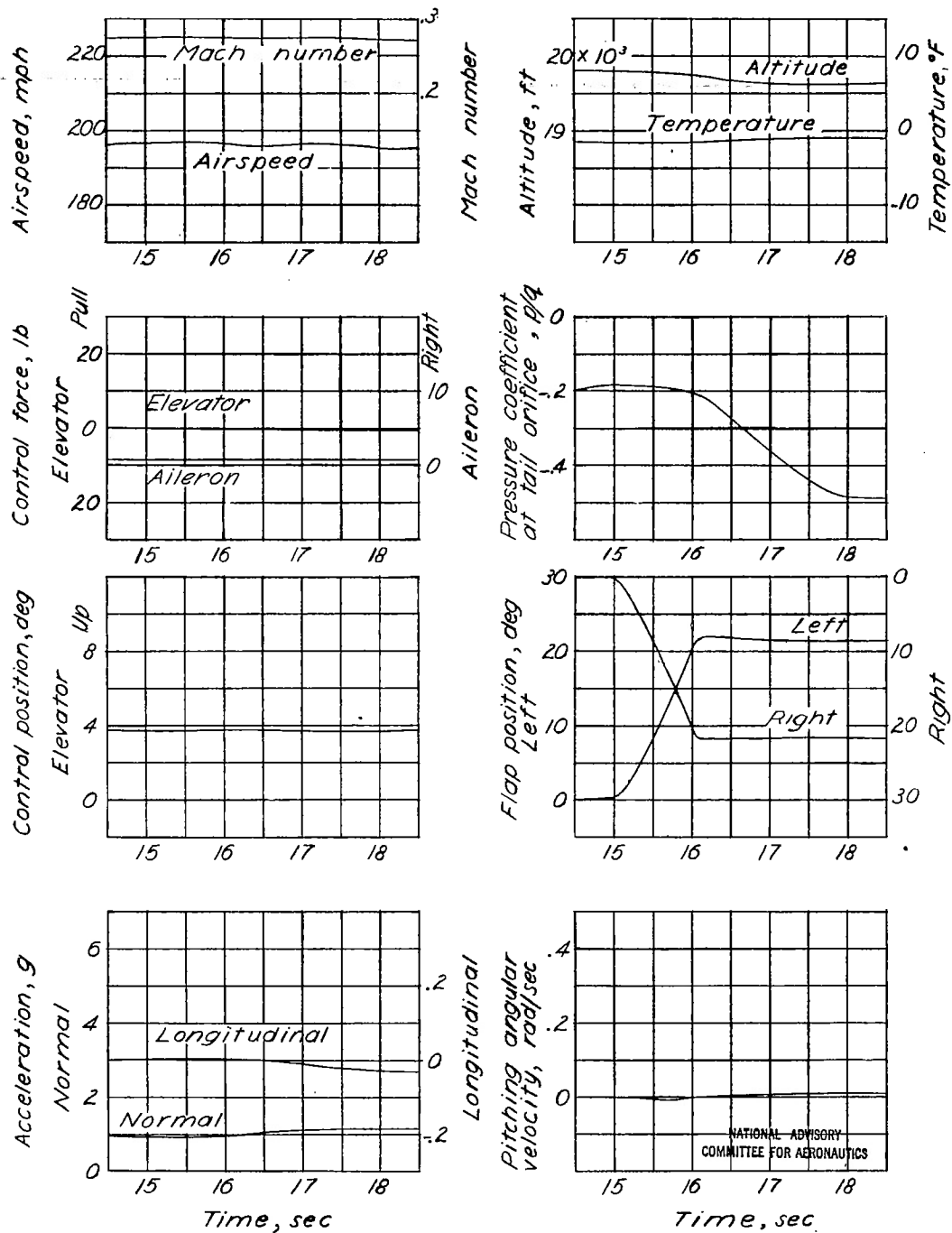
Figure 12.- Variation of basic measured quantities during dive-recovery-flap deflection. Dive-recovery-flap deflection, 21.5°; weight, 7870 pounds; center-of-gravity position, 28.36 percent mean aerodynamic chord.
