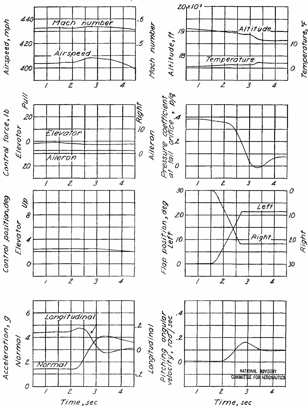
Figure 17.- Variation of basic measured quantities during dive-recovery-flap deflection. Dive-recovery-flap deflection, 21.5°; weight, 7720 pounds; center-of-gravity position, 27.97 percent mean aerodynamic chord.
