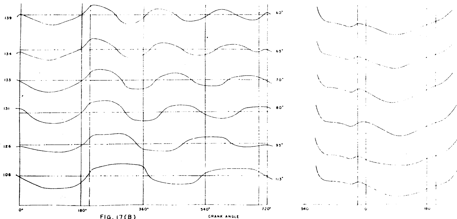
FIGURE 17. — PRESSURE IN PIPE AND CYLINDER FOR VARIOUS PIPE LENGTHS RPM 1600 PIPE DIAMETER 1.88 IN.
