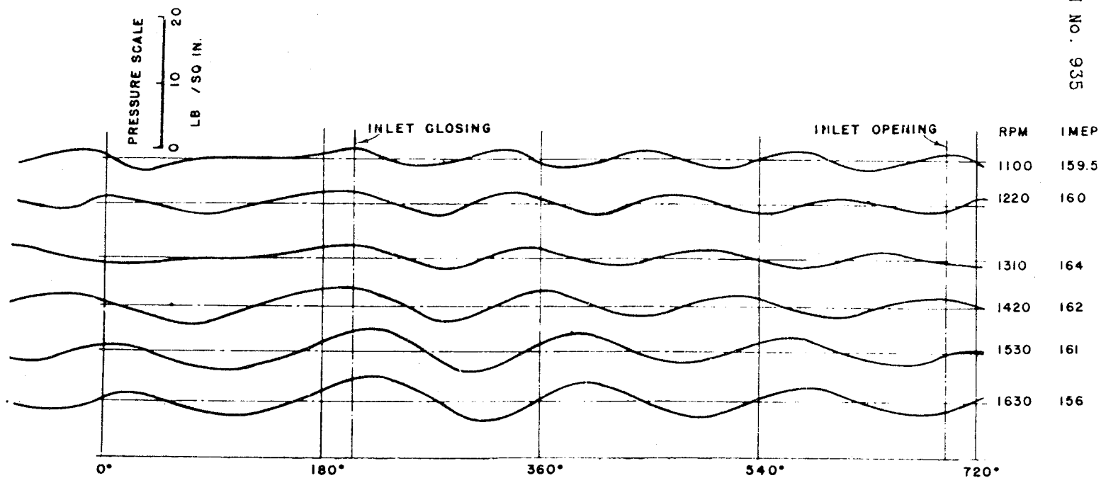
PRESSURE IN PIPE AT DIFFERENT RPM PIPE LENGTH 63 IN. DIAMETER 2.56 IN.
