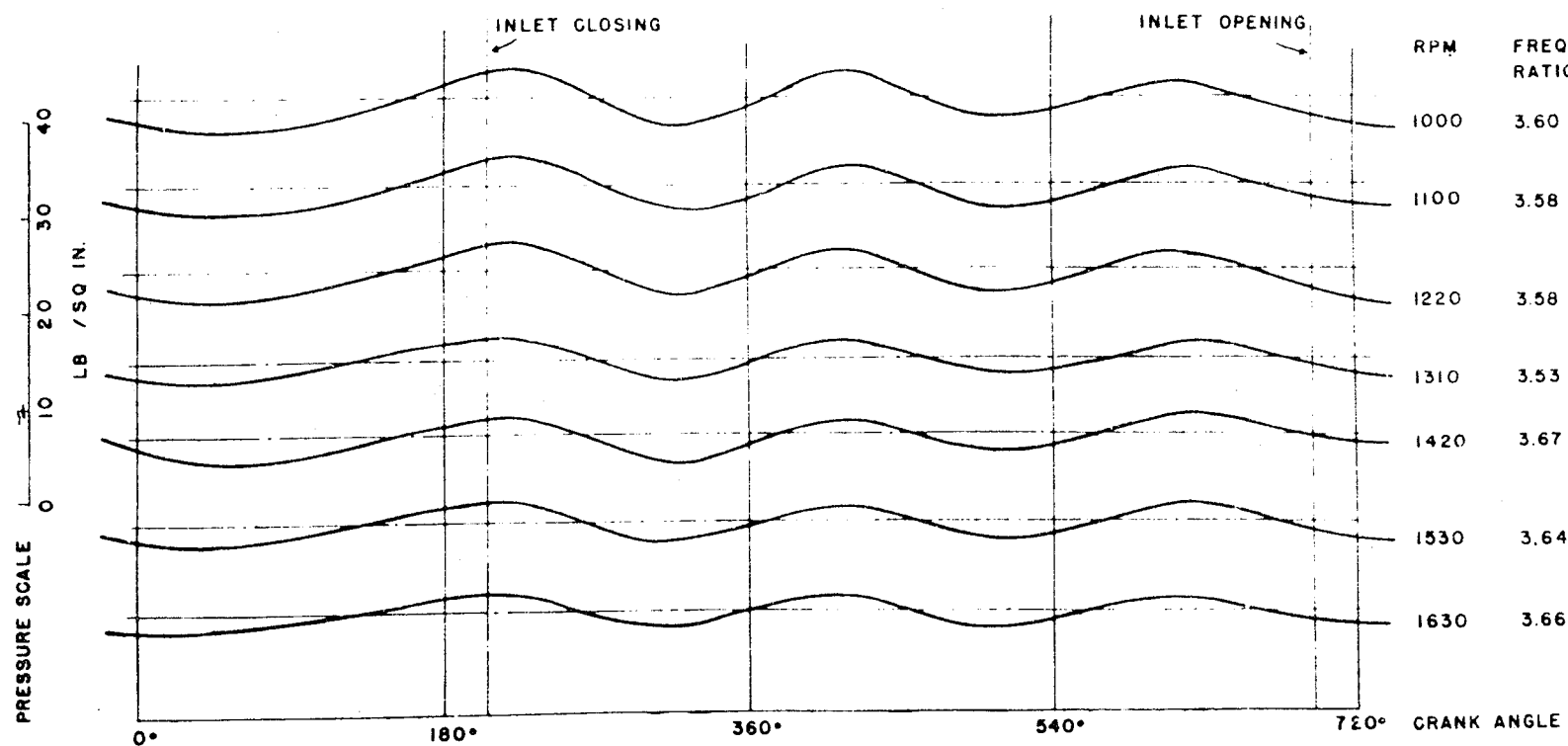
PRESSURE IN INLET PIPE FOR VARIOUS SPEEDS AT CONSTANT FREQUENCY RATIO
