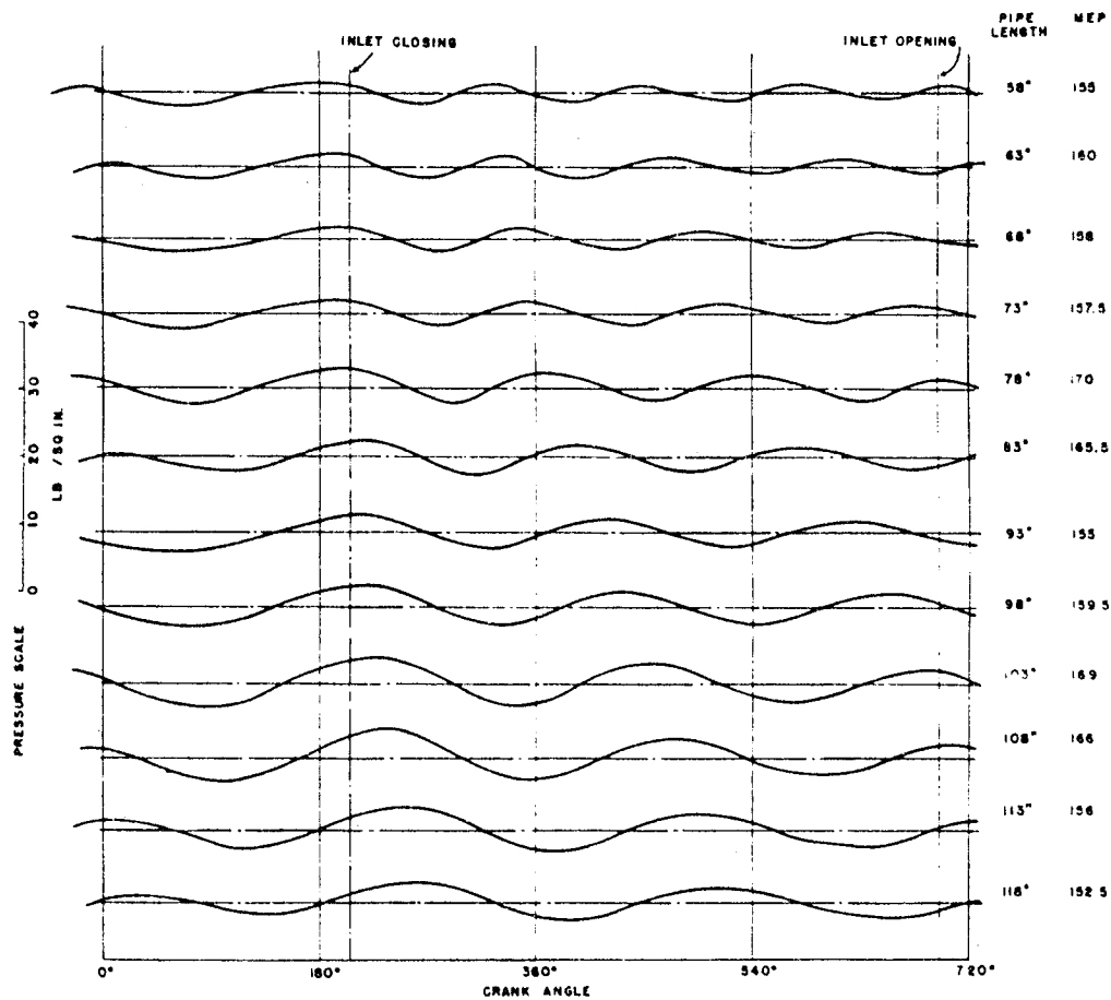
PRESSURE IN INLET PIPE FOR VARIOUS PIPE LENGTHS AT CONSTANT INLET CLOSING RPM 1220 PIPE DIAMETER 2.56 IN.
