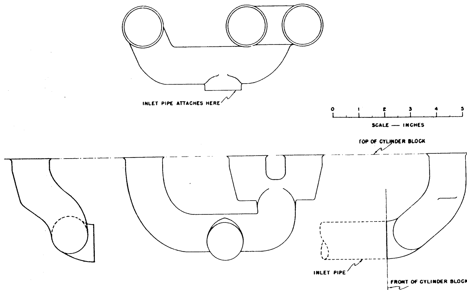
Figure 19. DETAIL OF INLET PASSAGE CORE MODIFIED TO SHOW SHAPE OF PASSAGE AFTER MACHINING
