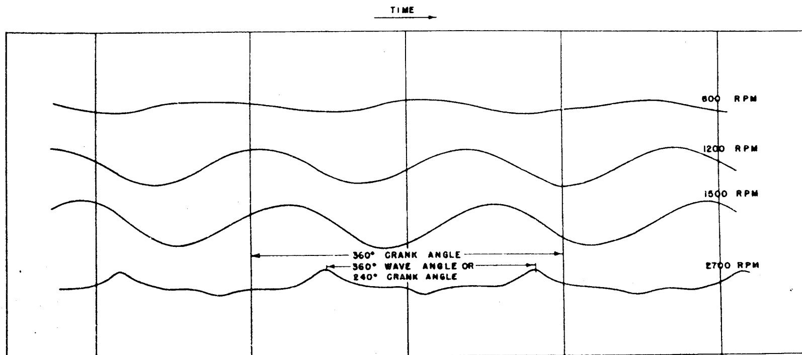
PRESSURE CURVES AT VARIOUS R P M 72 INCH PIPE
