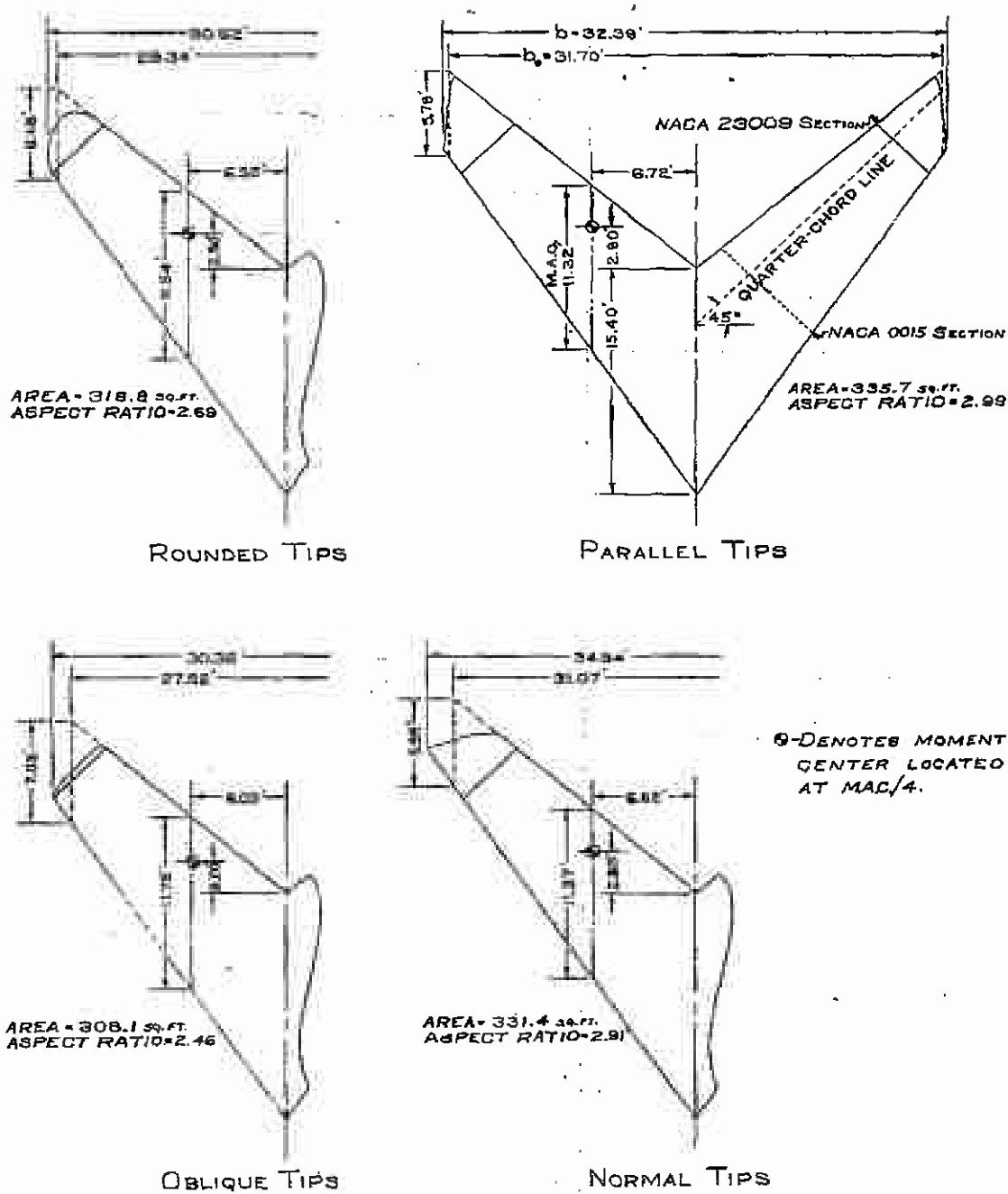
FIGURE 1.- GEOMETRIC CHARACTERISTICS OF 45-DEGREE SWEEP-FORWARD WING WITH VARIOUS TIPS.
