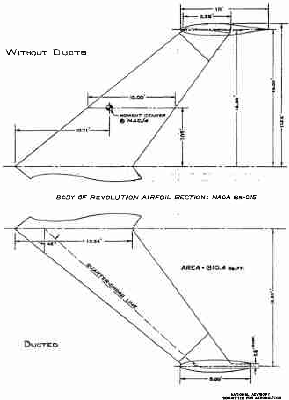
FIGURE 3.—GEOMETRIC CHARACTERISTICS OF 45-DEGREE SWEEP- BACK WING WITH BODY-OF-REVOLUTION TIPS.
