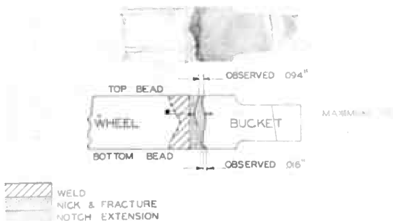
Figure 18 First Bucket Removed from Wheel-and-Bucket Design Test Specimen No. U-43 by Nick and Fracture Technique. Note that Maximum Notch Extension Has Occurred Near Center of Section Rather than at the Surface.
