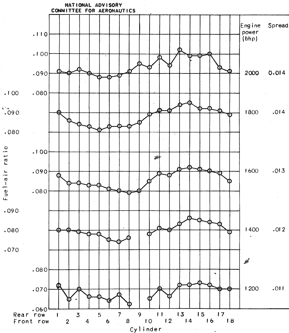
Figure 4. - Concluded. Fuel-air ratio distribution patterns obtained using NACA injection impellers in R-3350 engine.
