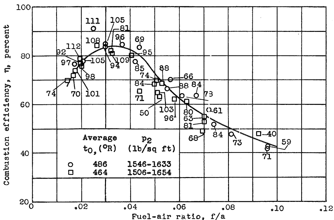
(b) Pressure altitude, 10,000 feet; combustion-chamber-inlet pressure, 1506 to 1654 pounds per square foot; average ambient-air temperature, 464° and 486° R.
