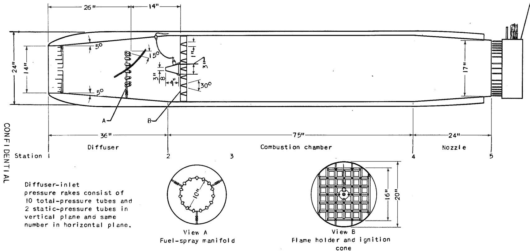
Figure 3. - Schematic cross-sectional view of 20-inch ram jet.
