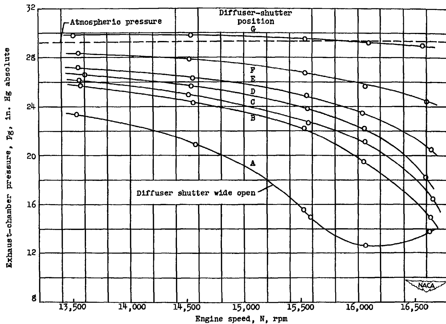
Figure 5. - Variation of exhaust-chamber pressure with engine speed for various shutter positions. Bell-shaped inlet nozzle and 1\frac{1}{2} -inch-diameter throat.
