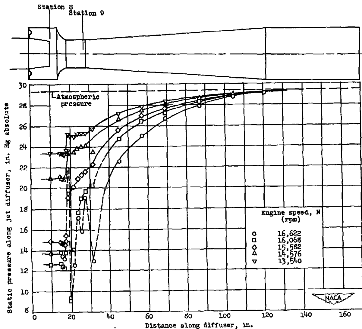
Figure 6. - Variation of static pressures along jet diffuser for wide-open shutter position. Bell-shaped inlet nozzle and 13\frac{1}{2} -inch-diameter throat.
