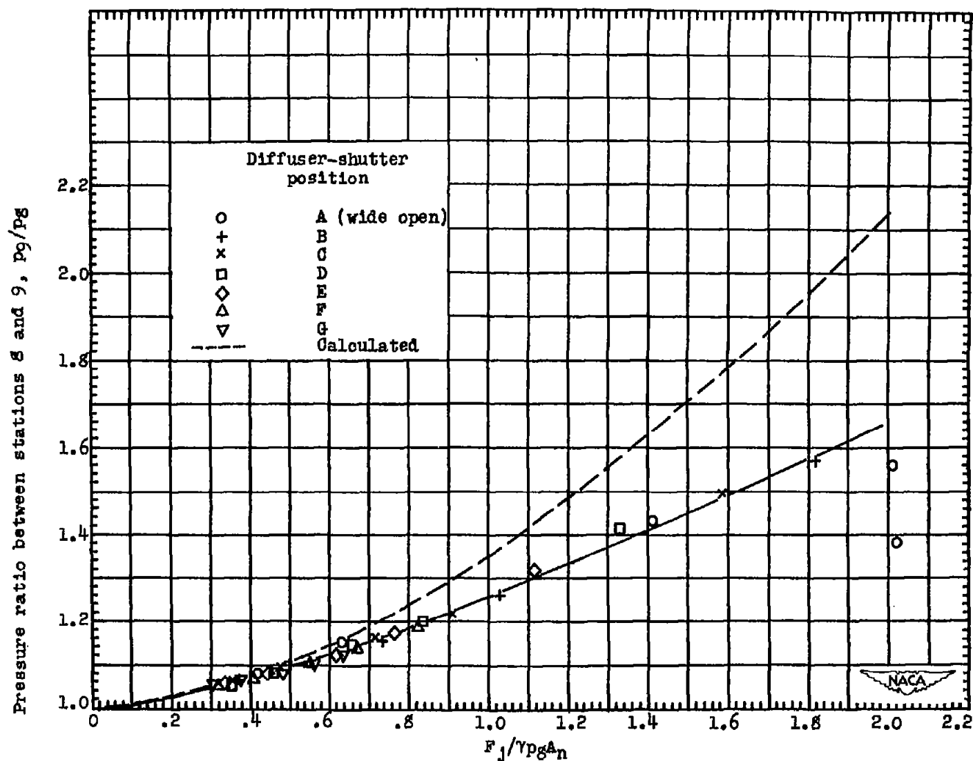
Figure 7. - Comparison of calculated and experimental values of pressure ratio between stations 8 and 9 for bell-shaped inlet nozzle and 1\frac{3}{4} -inch-diameter throat.
