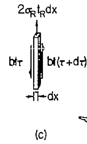
Figure 4.- Panel with finite transverse stiffness.
