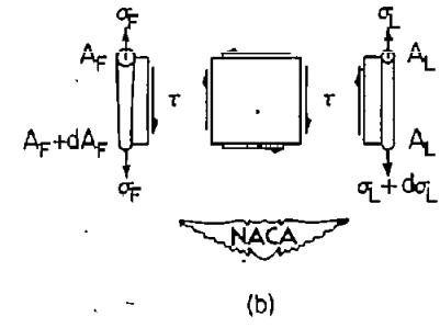
Figure 2.- Panel with constant-stress flange.
