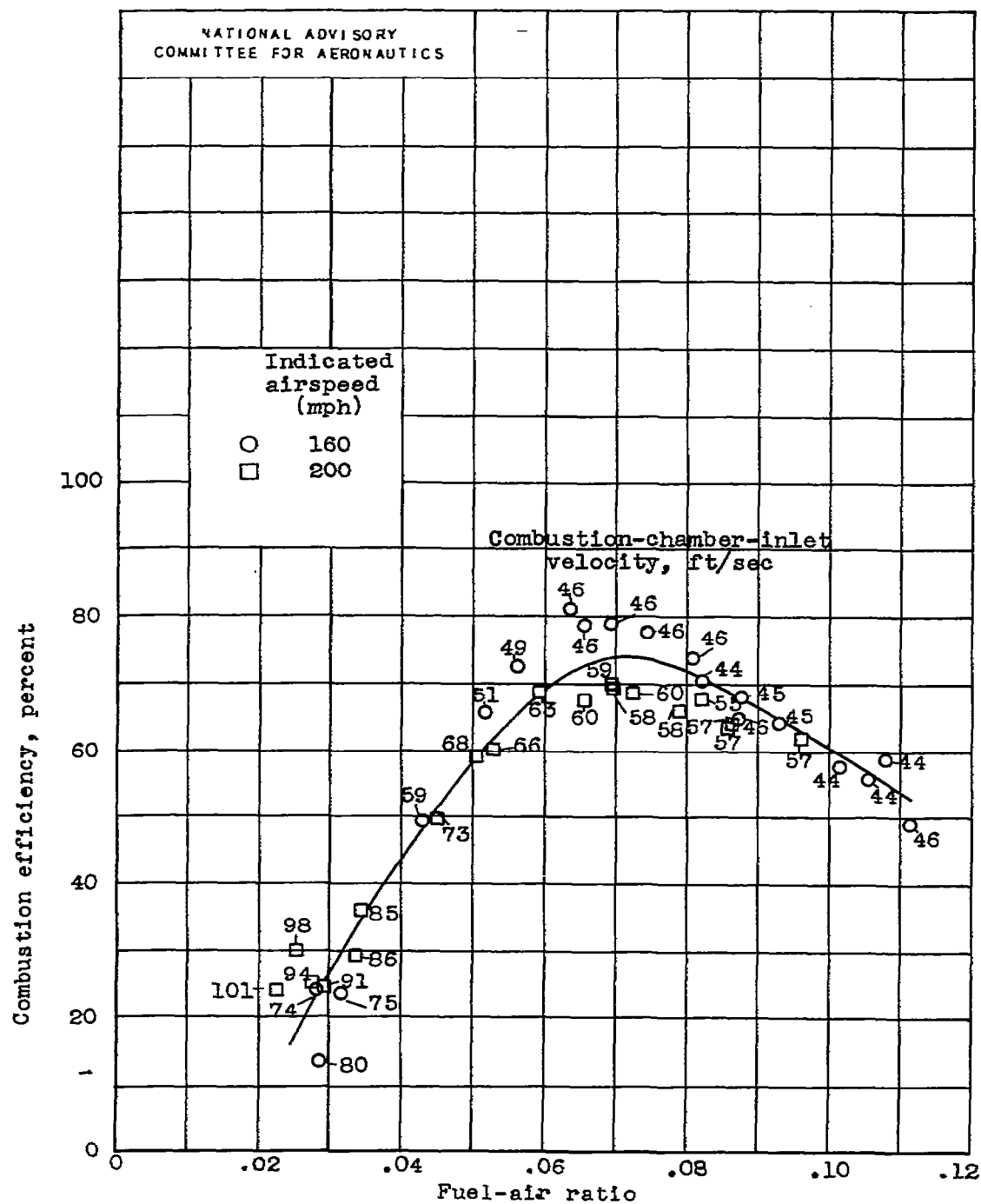
Figure 10. - Continued. Effect of fuel-air ratio on combustion efficiency.
