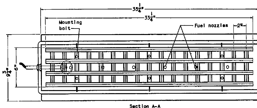
Figure 4. - Schematic drawing of rectangular ram jet incorporating four-V gutter-type flame holder.
