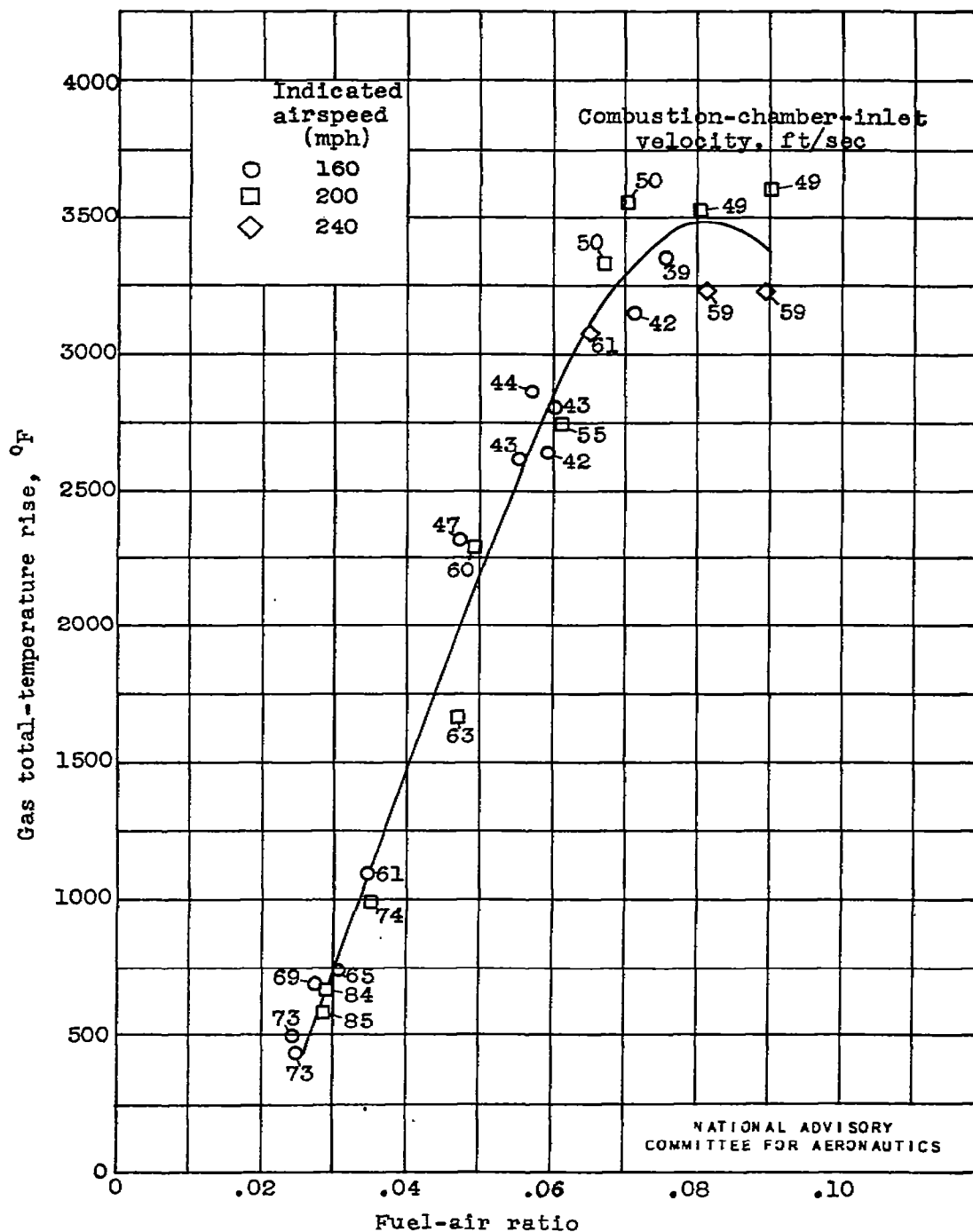
Figure 8. - Effect of fuel-air ratio on gas total-temperature rise.
