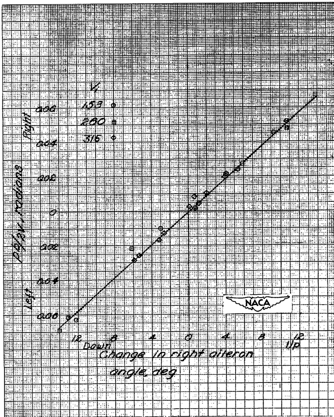
Figure 20.- Variation of helix angle pb/2V with change in right aileron deflection as measured in clean condition, rudder-fixed aileron rolls. XS-1 10-percent-thick-wing airplane.
