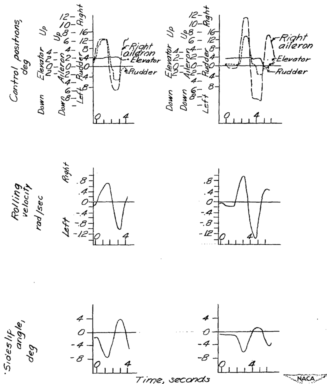
Figure 26.- Time histories of aileron rolls at 150 mph in which the pilot used more rudder than necessary to overcome the sideslip due to ailerons. XS-1 airplane.
