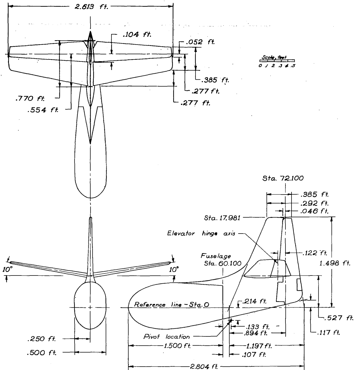
Figure 3.- Details and dimensions of 0.14-scale model of the XP-83 airplane tail unit tested in the Langley 4-by 6-foot wind tunnel.
