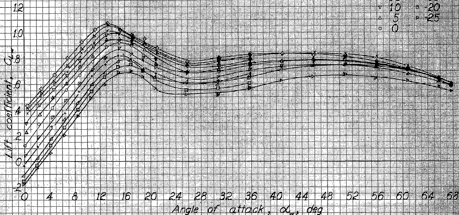
Figure 7 - Lift characteristics of aileron on left wing panel of 0.14-scale model of the XP-83 airplane.
