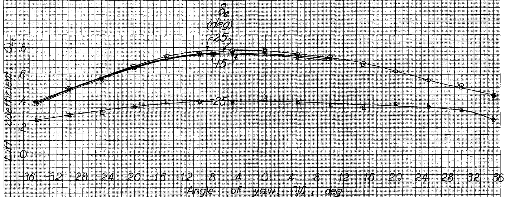
Figure 14 - (Continued) (b) \alpha_e = 50.4^\circ
