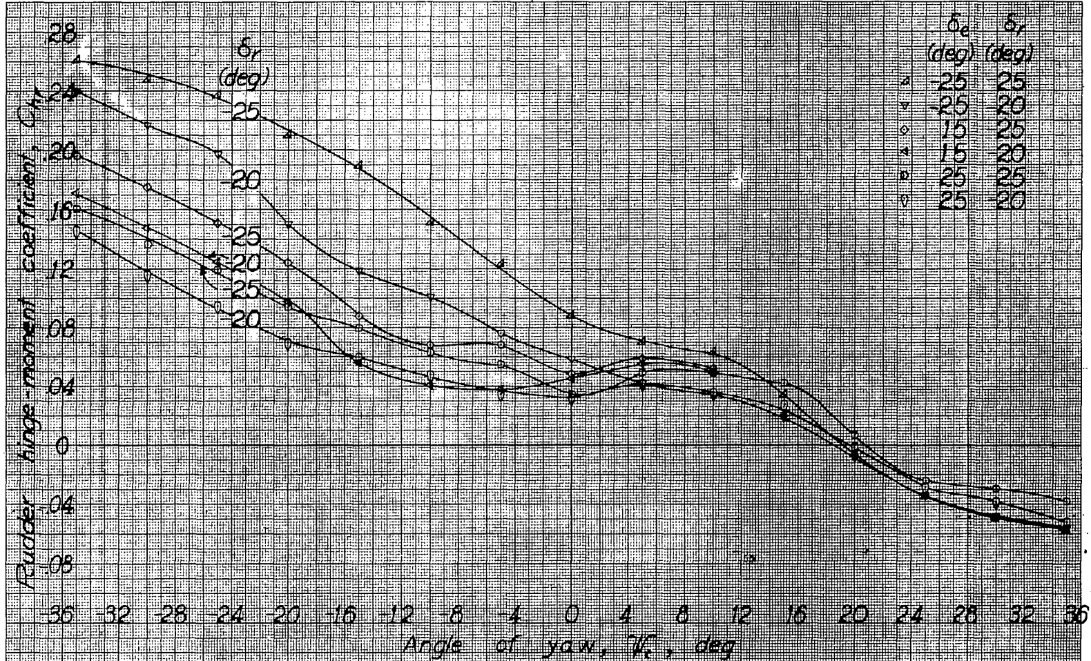
(a) Continued Figure 12 - (Continued)
