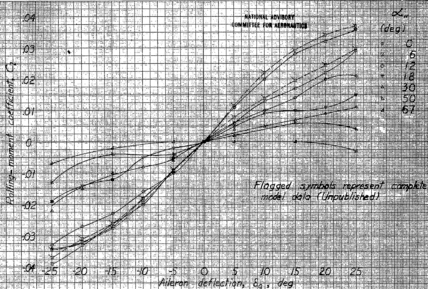
Figure 9. - Rolling-moment characteristics of complete wing of XP-83 airplane with only left aileron deflected, as estimated from left-wing-panel test data.
