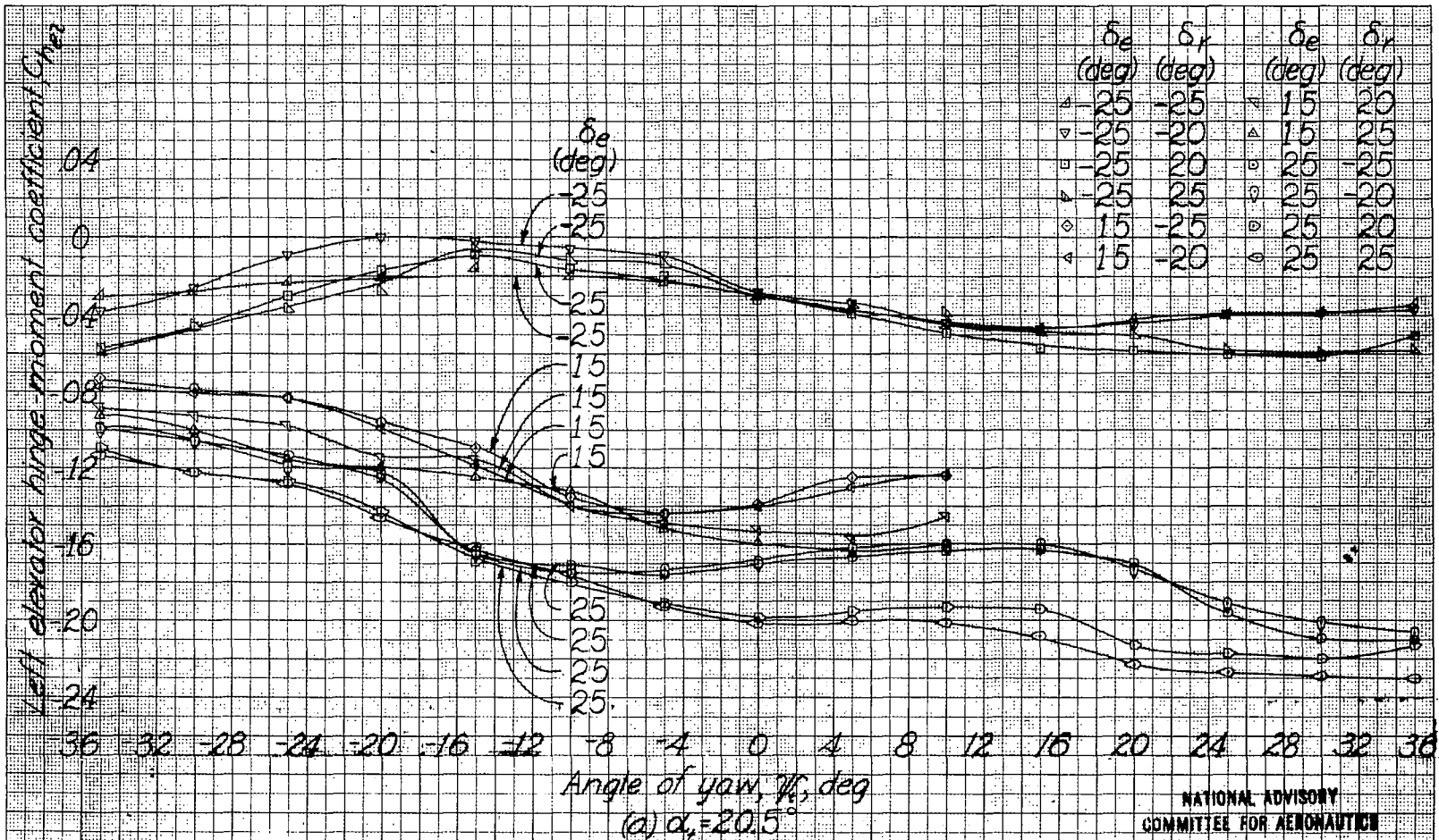
Figure 12.- Left elevator and rudder hinge-moment characteristics of 0.14-scale model of the XP-83 airplane tail surfaces as tested in the Langley 4-by 6-foot wind tunnel.
