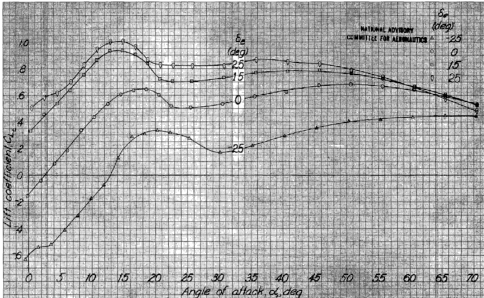
Figure 13.-Elevator lift and drag characteristics obtained from tests of 0.14-scale model of the XP-83 airplane tail surfaces (with fuselage interference) in the Langley 4-by-6-foot wind tunnel. \delta_r = 0^\circ , \eta = 0^\circ
