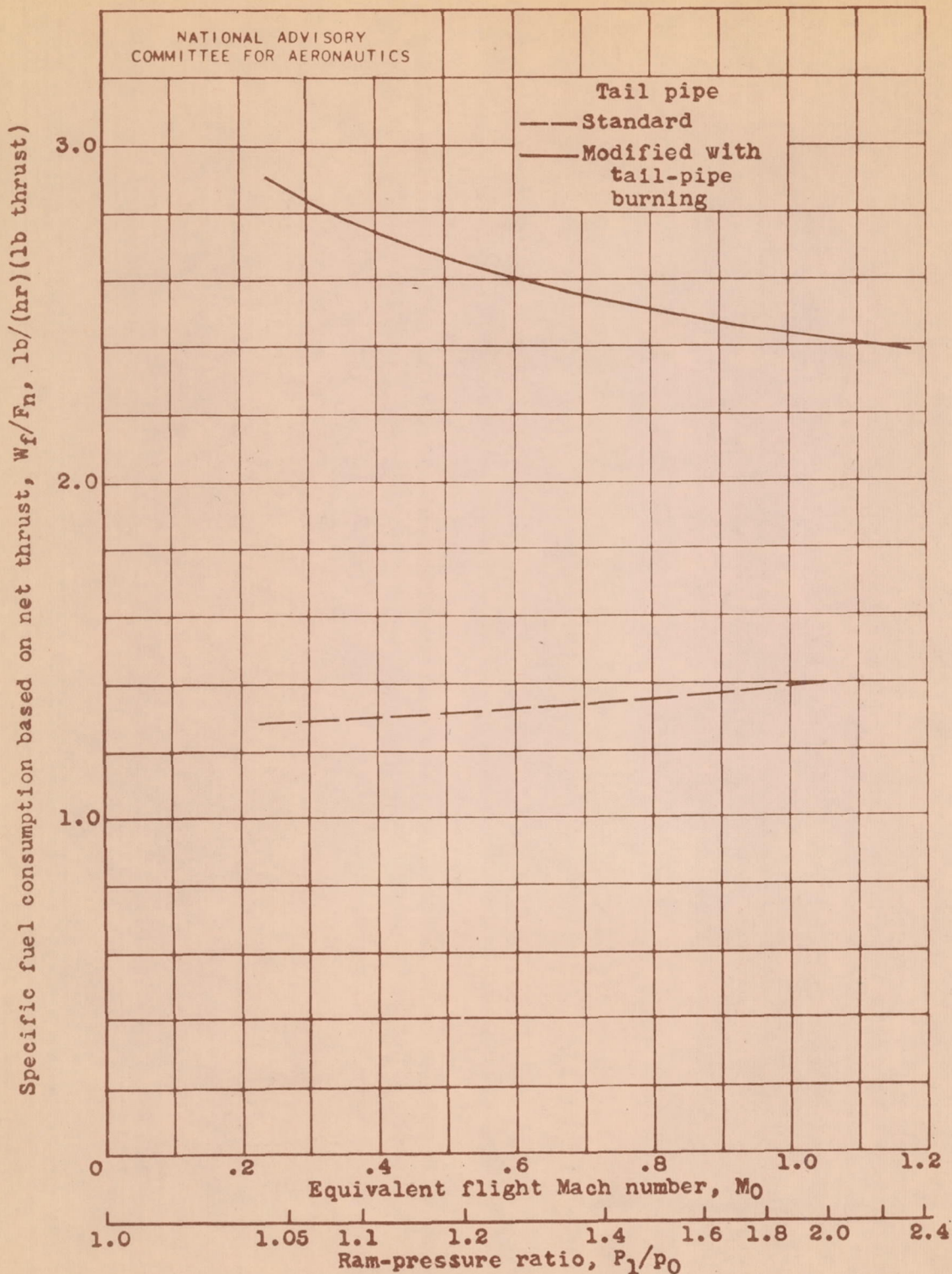
Figure 18.- Relation between equivalent flight Mach number and specific fuel consumption based on net thrust for turbojet engine with standard tail pipe and modified tail pipe with tail-pipe burning. Engine speed, 7600 rpm; turbine-outlet temperature, 1220° F; altitude, 30,000 feet.
