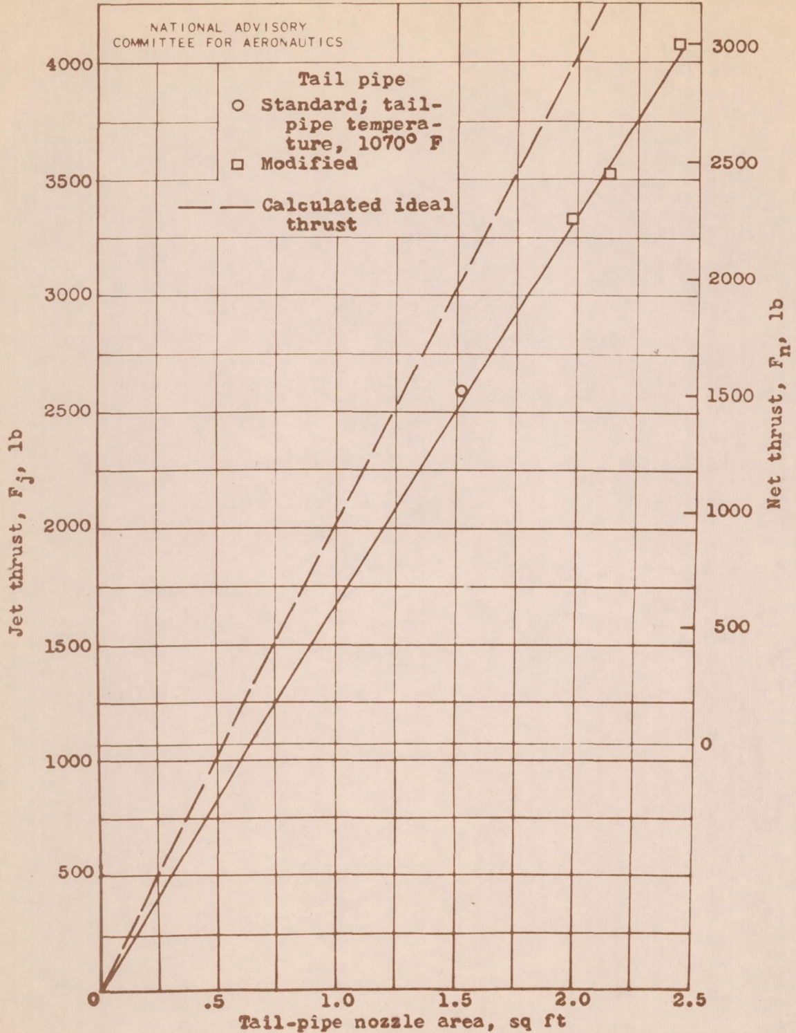
Figure 9.- Relation between nozzle area and thrust of turbo-jet engine with tail-pipe burning. Engine speed, 7600 rpm; turbine-outlet temperature, 1220° F; ram-pressure ratio, 1.66; altitude, 30,000 feet. Value of \gamma was assumed equal to 1.27 for calculation of theoretical thrust.
