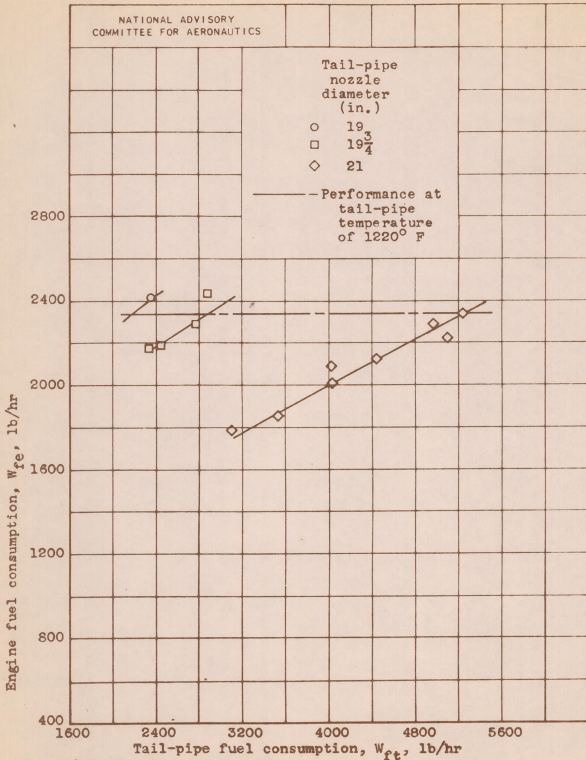
(c) Engine fuel consumption.
