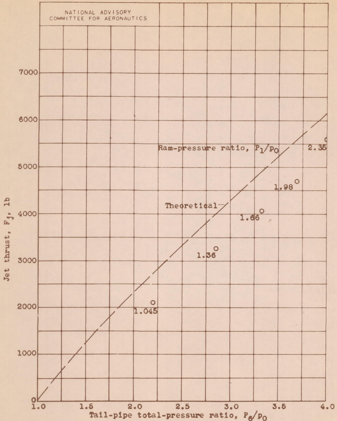
Figure 15.- Effect of ram-pressure ratio on relation between tail-pipe total-pressure ratio and jet thrust of turbojet engine with tail-pipe burning. Engine speed, 7600 rpm; turbine-outlet temperature, 1220° F; altitude, 30,000 feet.
