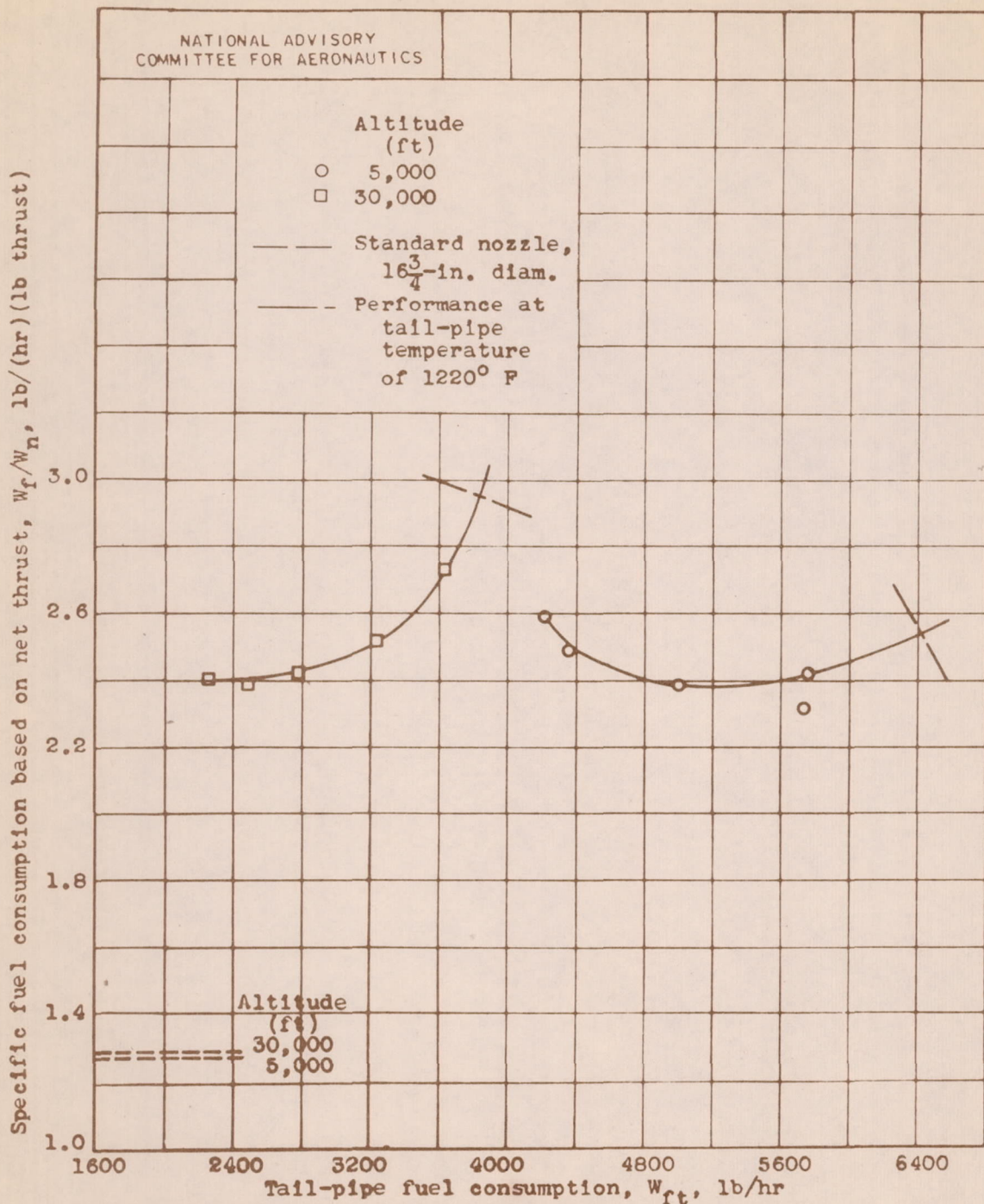
(d) Specific fuel consumption based on net thrust.
