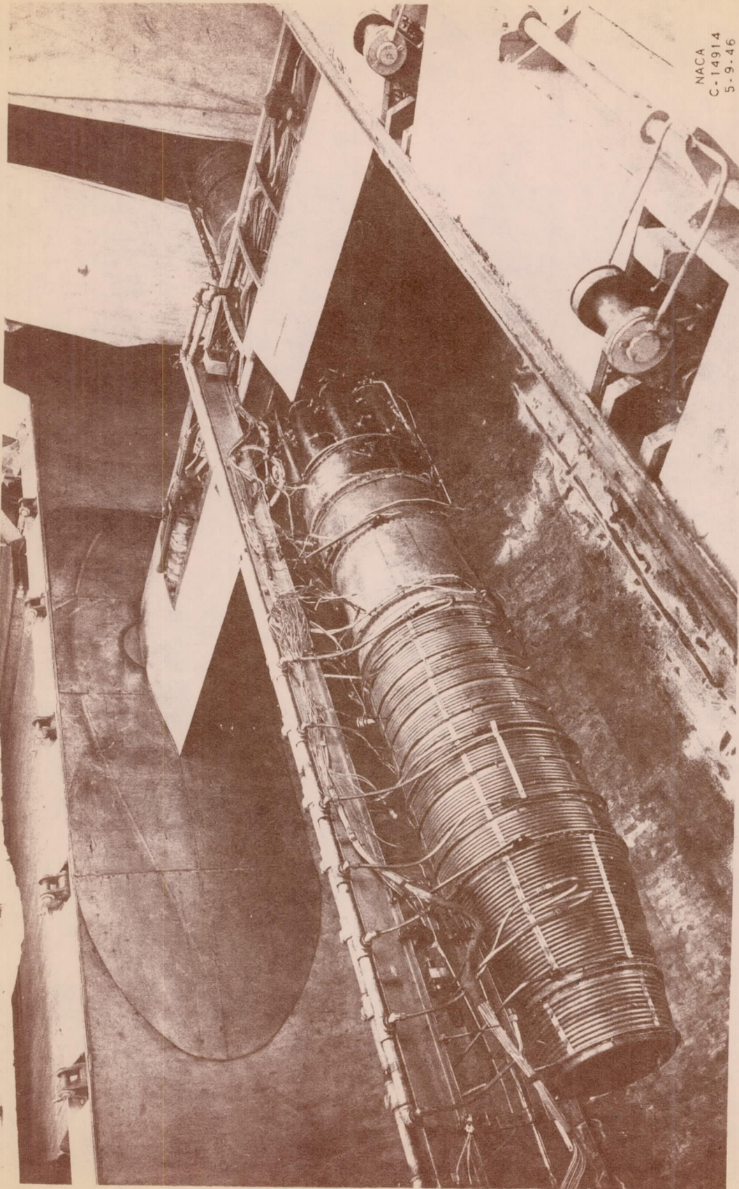
Figure 4. - Wind-tunnel installation of TG-180 turbojet engine with tail-pipe combustion chamber.
