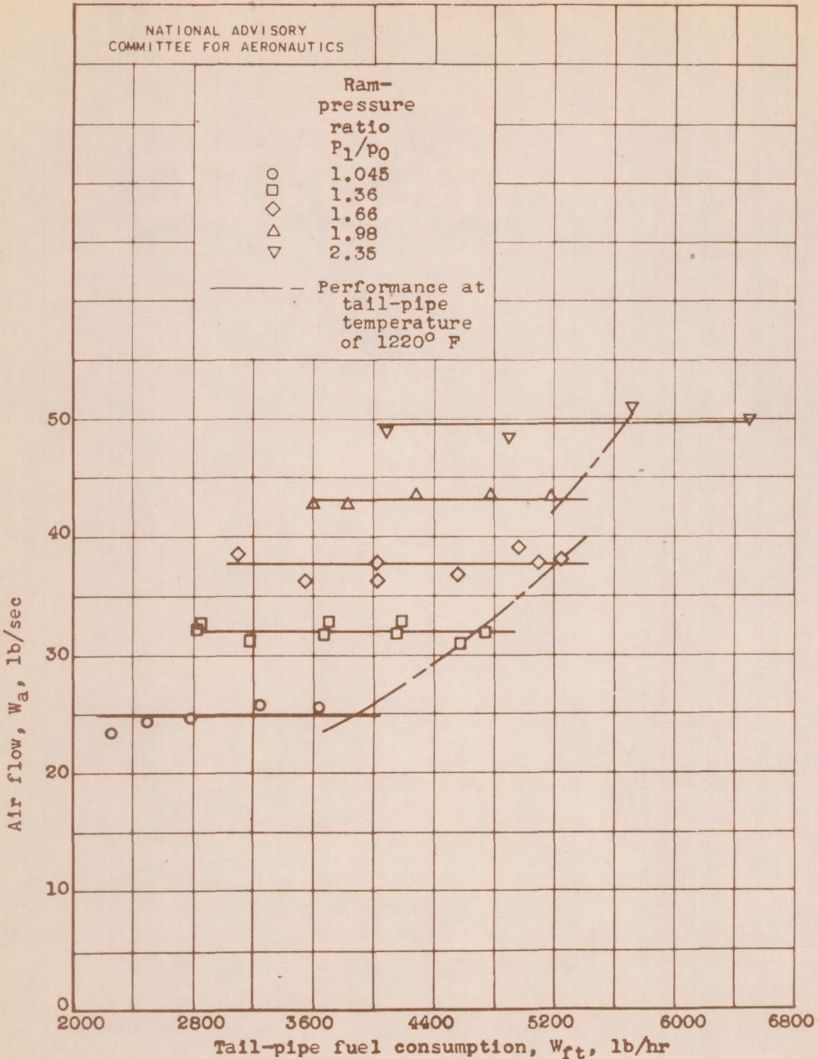
(e) Air flow.
