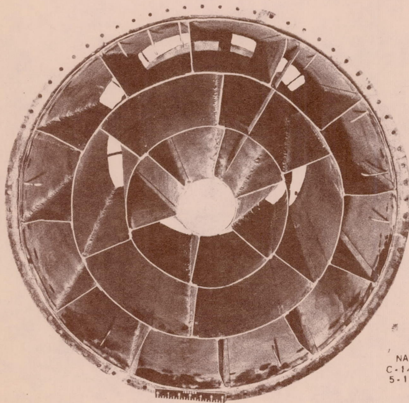
Figure 2. - Downstream end of diffuser for modified tailpipe of TG-180 turbojet engine.
