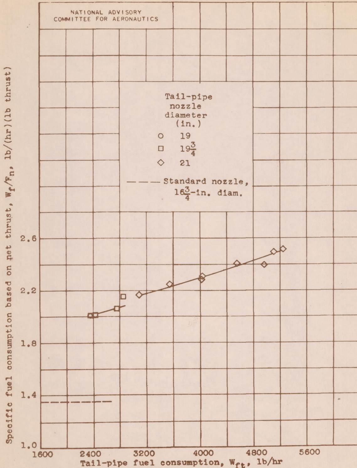
(d) Specific fuel consumption based on net thrust.
