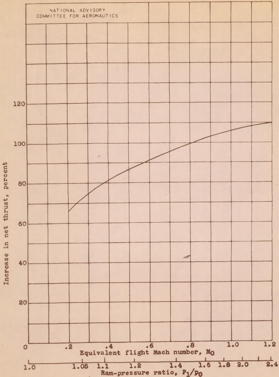
Figure 17.- Relation between equivalent flight Mach number and percentage increase in net thrust resulting from tail-pipe burning with turbojet engine. Engine speed, 7600 rpm; turbine-outlet temperature, 1220° F; altitude, 30,000 feet.
