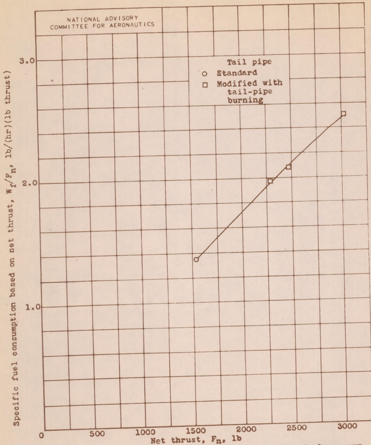
Figure 12.- Relation between net thrust and specific fuel consumption based on net thrust of turbojet engine with standard tail pipe and with modified tail pipe with tail-pipe burning. Engine speed, 7600 rpm; turbine-outlet temperature, 1220° F; ram-pressure ratio, 1.66; altitude, 30,000 feet.
