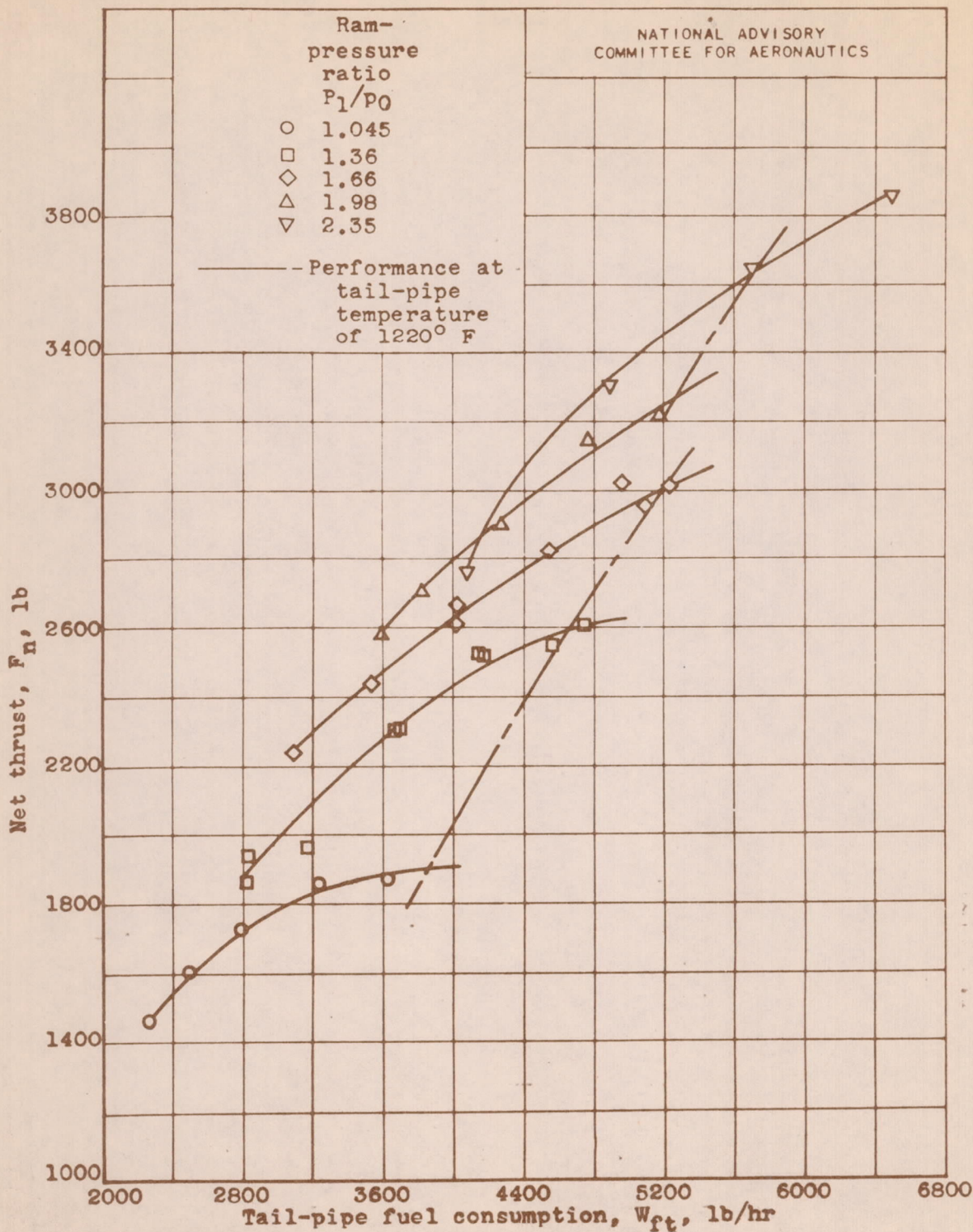
(b) Net thrust.
