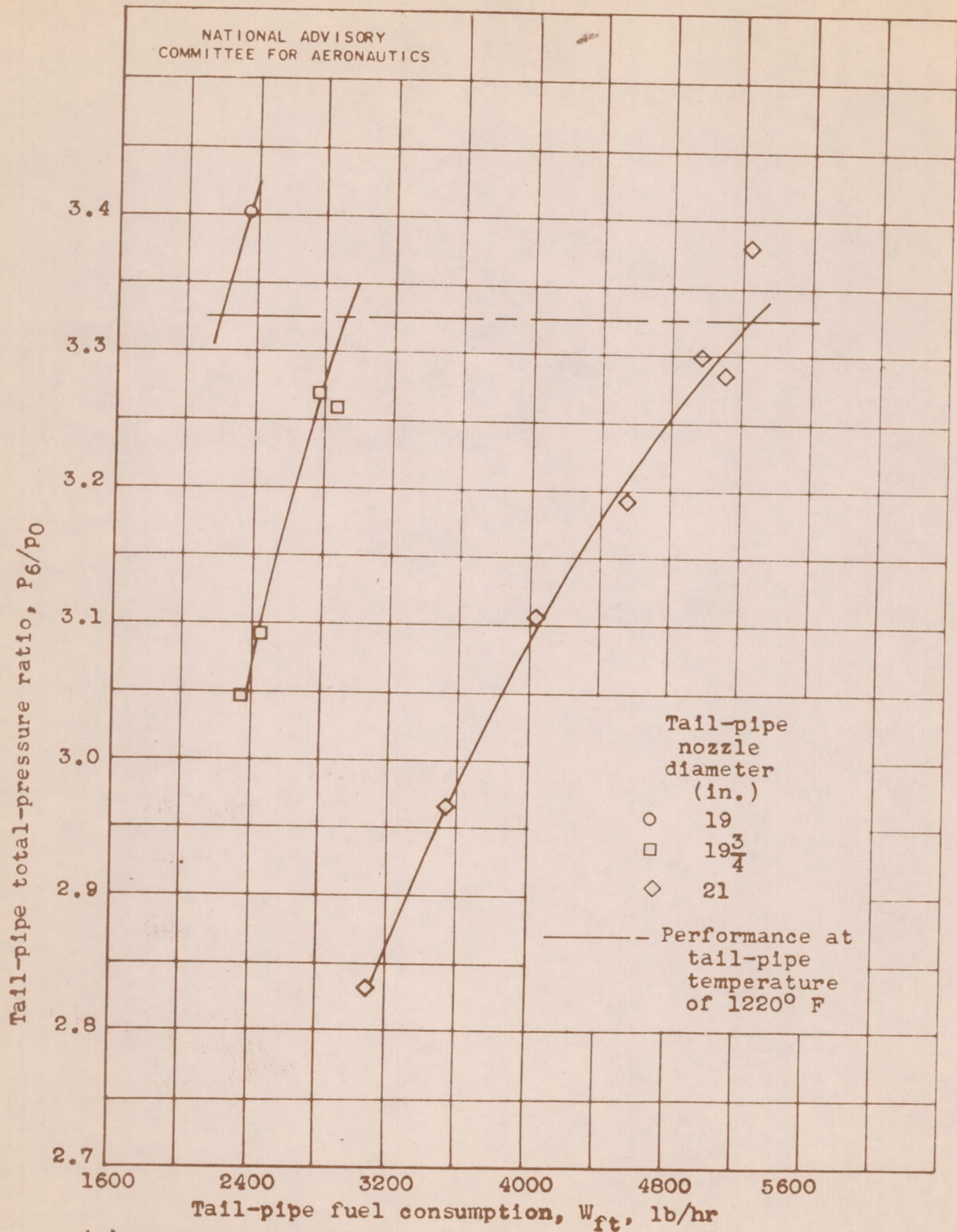
(g) Tail-pipe total-pressure ratio.
