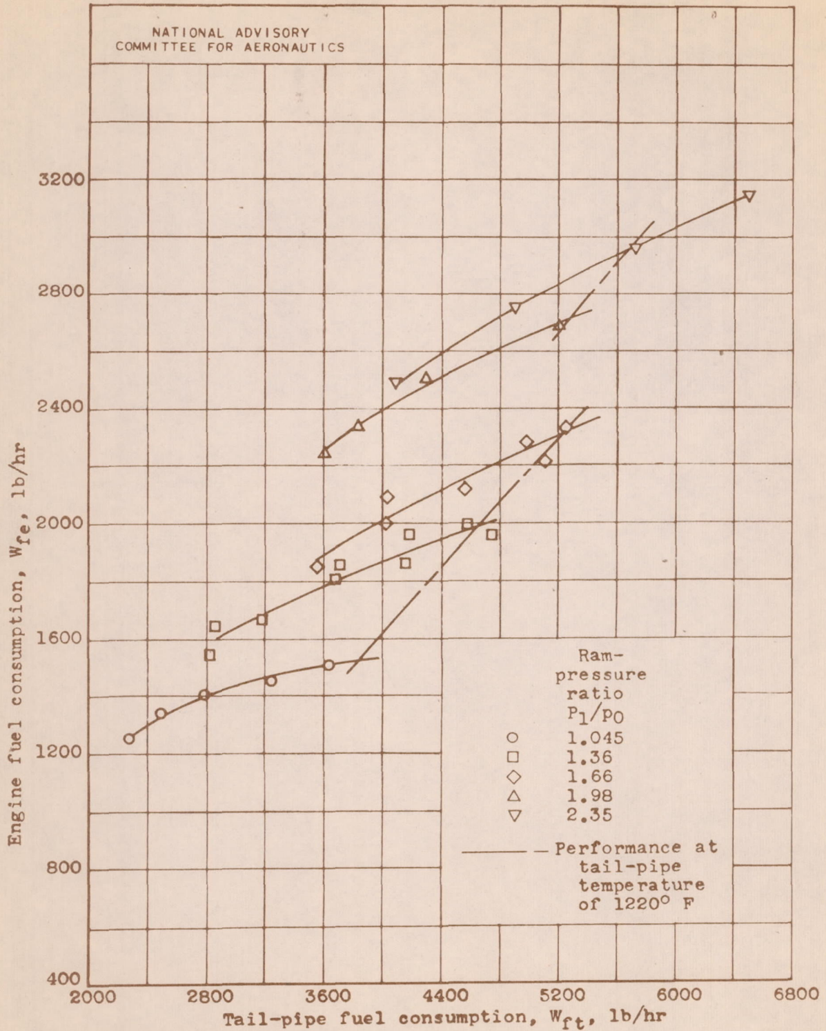
(c) Engine fuel consumption.
