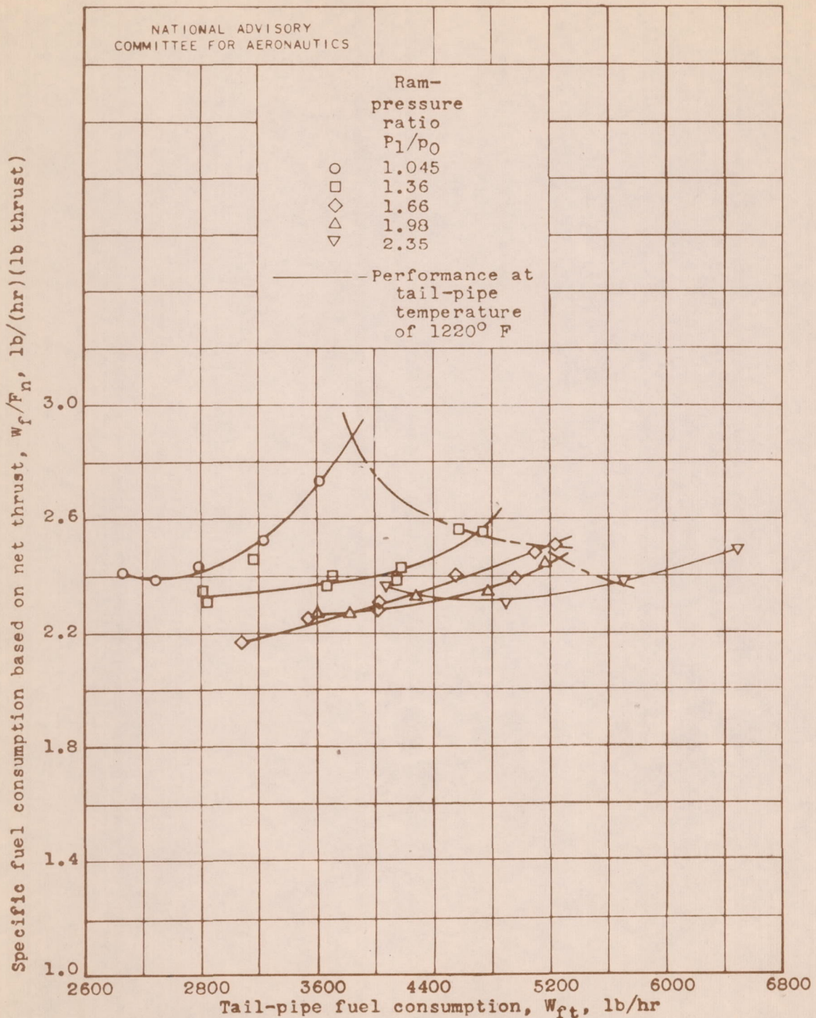
(d) Specific fuel consumption based on net thrust. Figure 8.- Continued. Variation of turbojet engine performance with tail-pipe fuel consumption for five ram-pressure ratios. Altitude, 30,000 feet; 21-inch-diameter tail-pipe nozzle.
