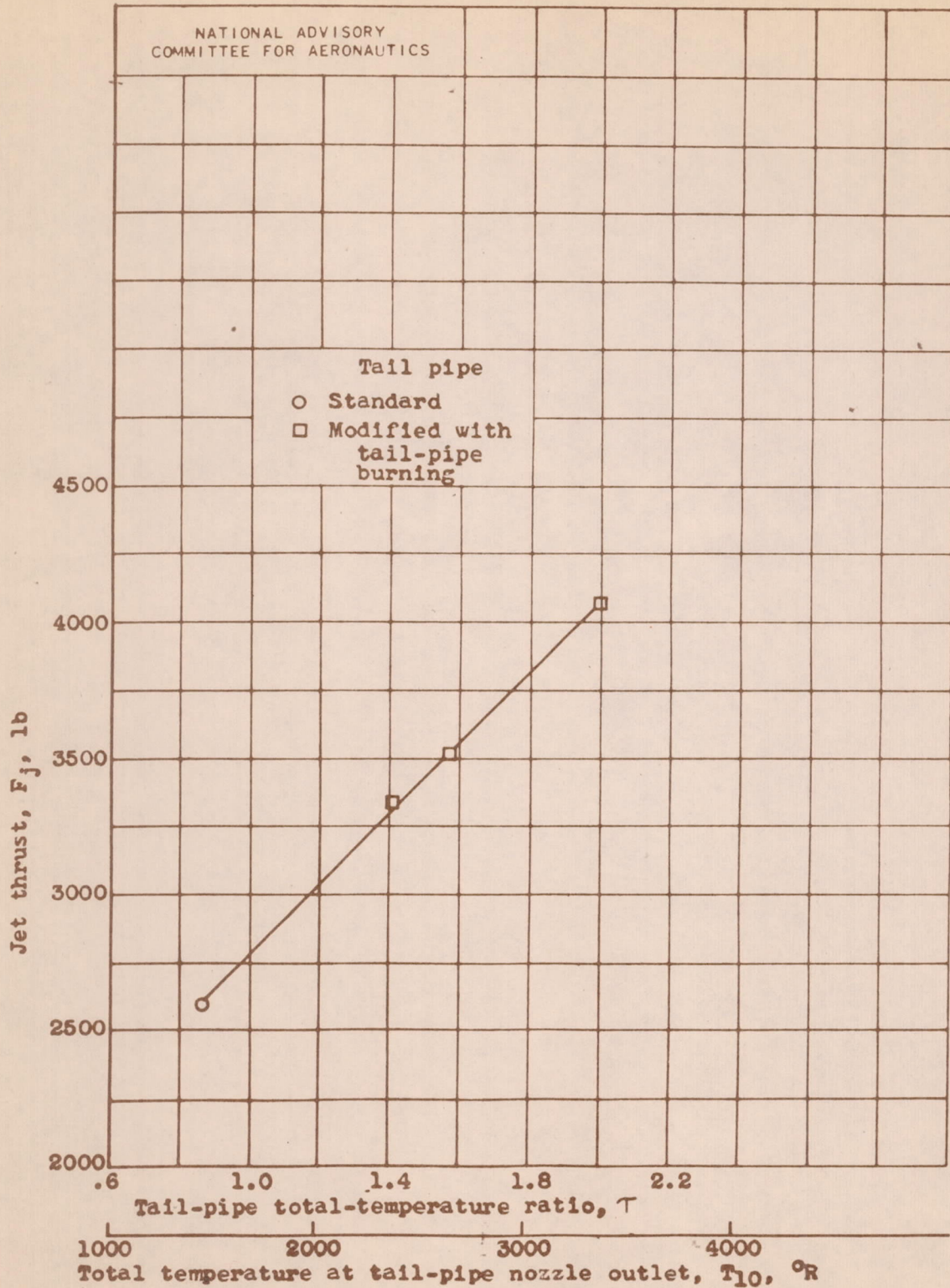
Figure 10.- Relation between jet thrust and total temperature of gases leaving tail pipe of turbojet engine with tail-pipe burning. Engine speed, 7600 rpm; turbine-outlet temperature, 1220° F; ram-pressure ratio, 1.66; altitude, 30,000 feet.
