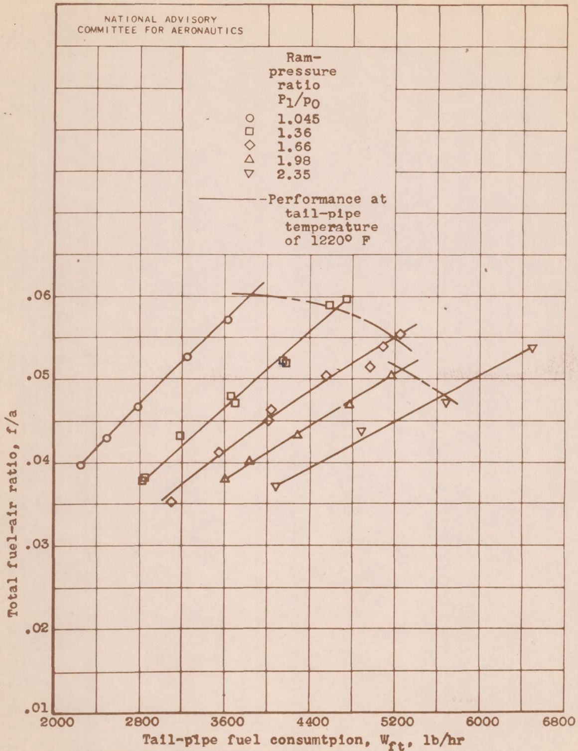
(f) Total fuel-air ratio.
