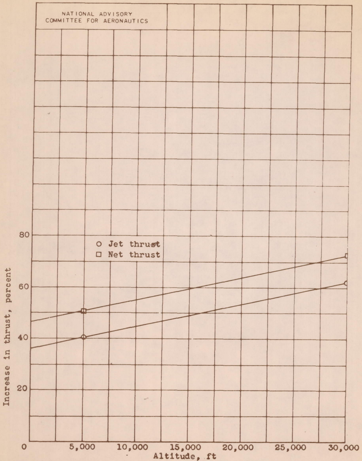
Figure 13.- Effect of altitude on percentage increase in thrust from tail-pipe burning with turbojet engine. Engine speed, 7600 rpm; turbine-outlet temperature, 1220° F; ram-pressure ratio, 1.045; 21-inch-diameter tail-pipe nozzle.
