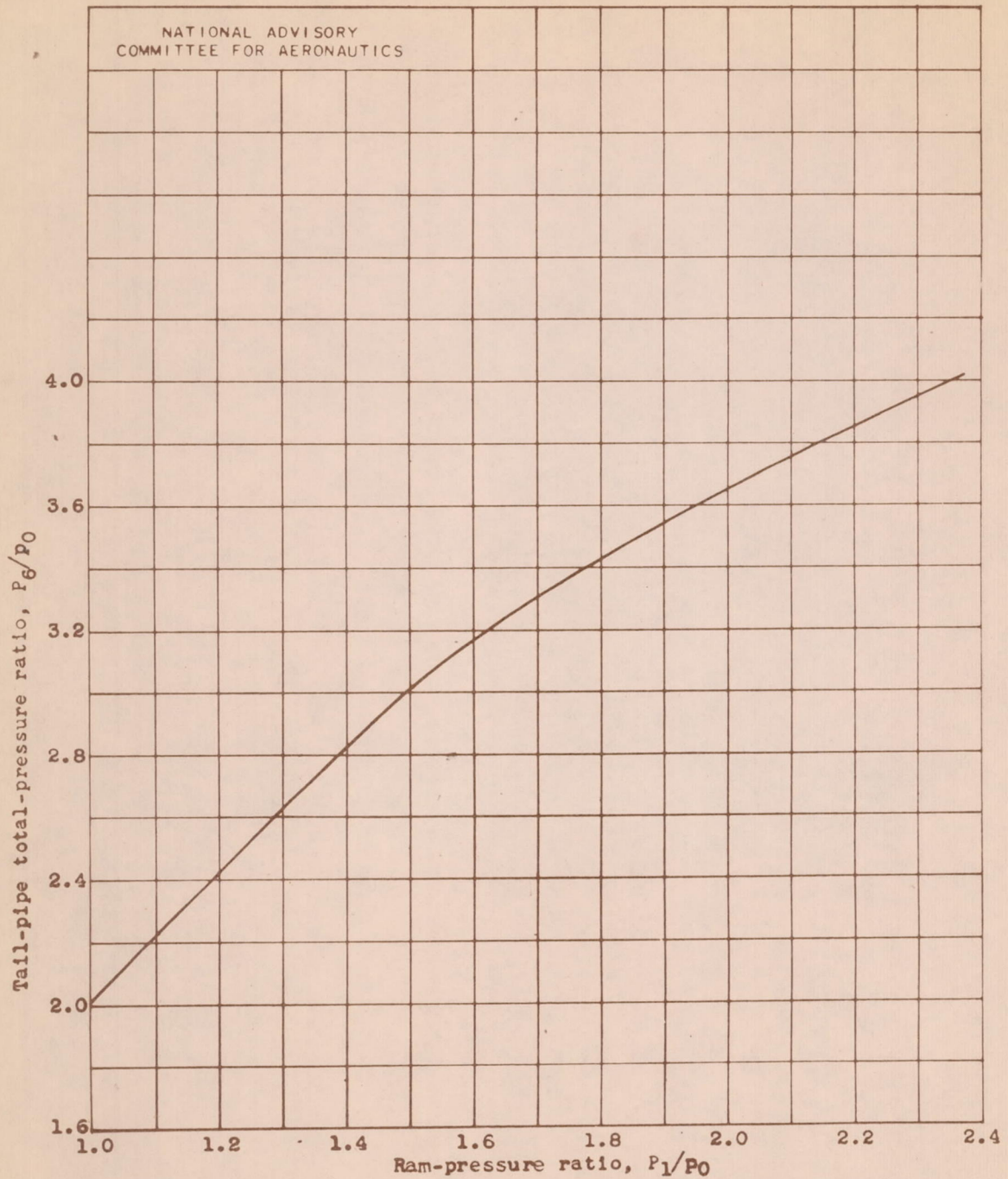
Figure 14.- Relation between tail-pipe total-pressure ratio and ram-pressure ratio for turbojet engine with tail-pipe burning. Engine speed, 7600 rpm; turbine-outlet temperature, 1220° F; altitude, 30,000 feet.
