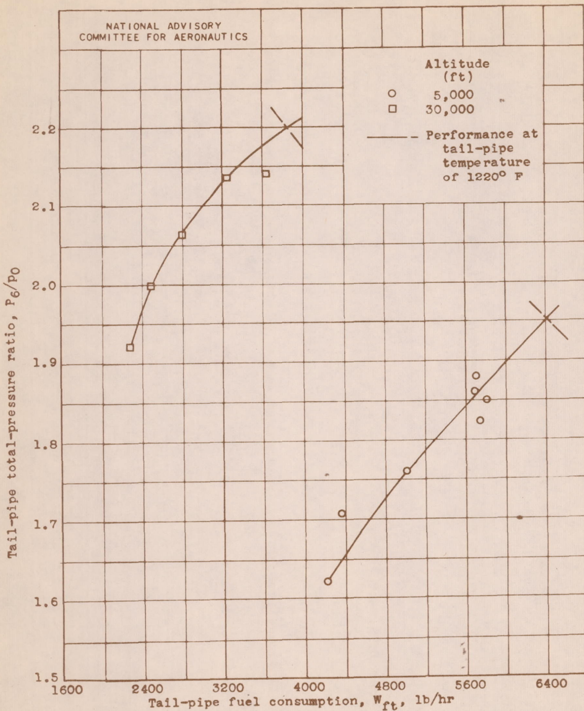
(g) Tail-pipe total-pressure ratio.
