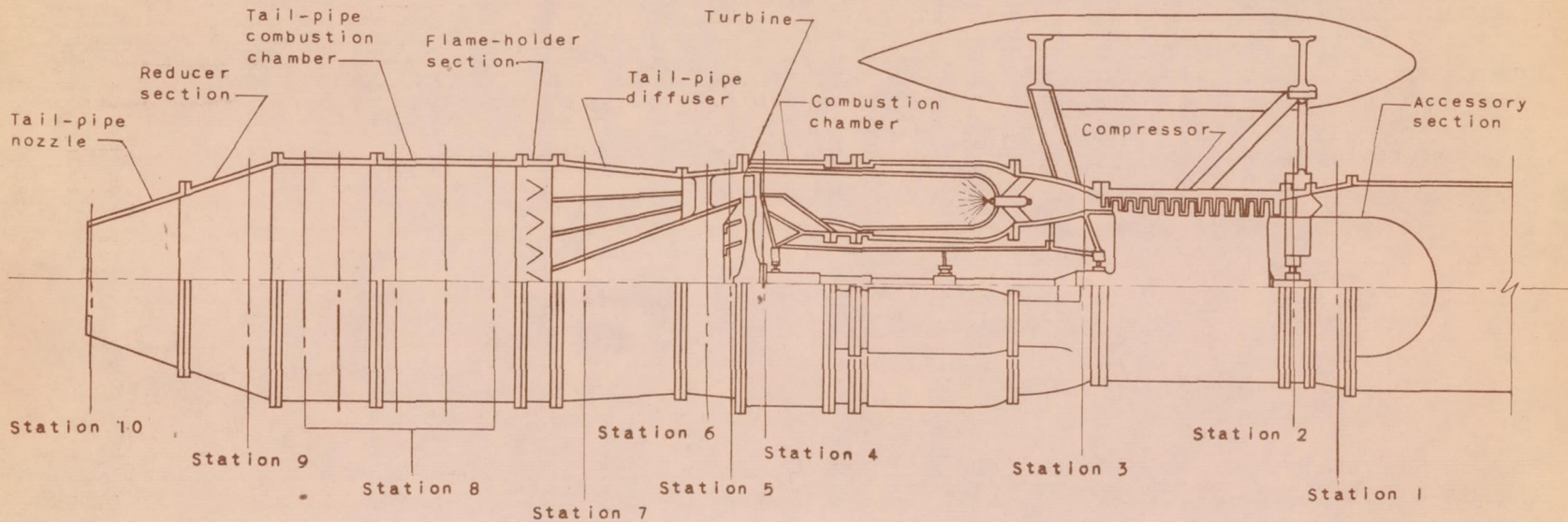
Figure 1. - Installation of TG-180 turbojet engine with tail-pipe combustion chamber showing relation of component parts and measuring stations in engine.
