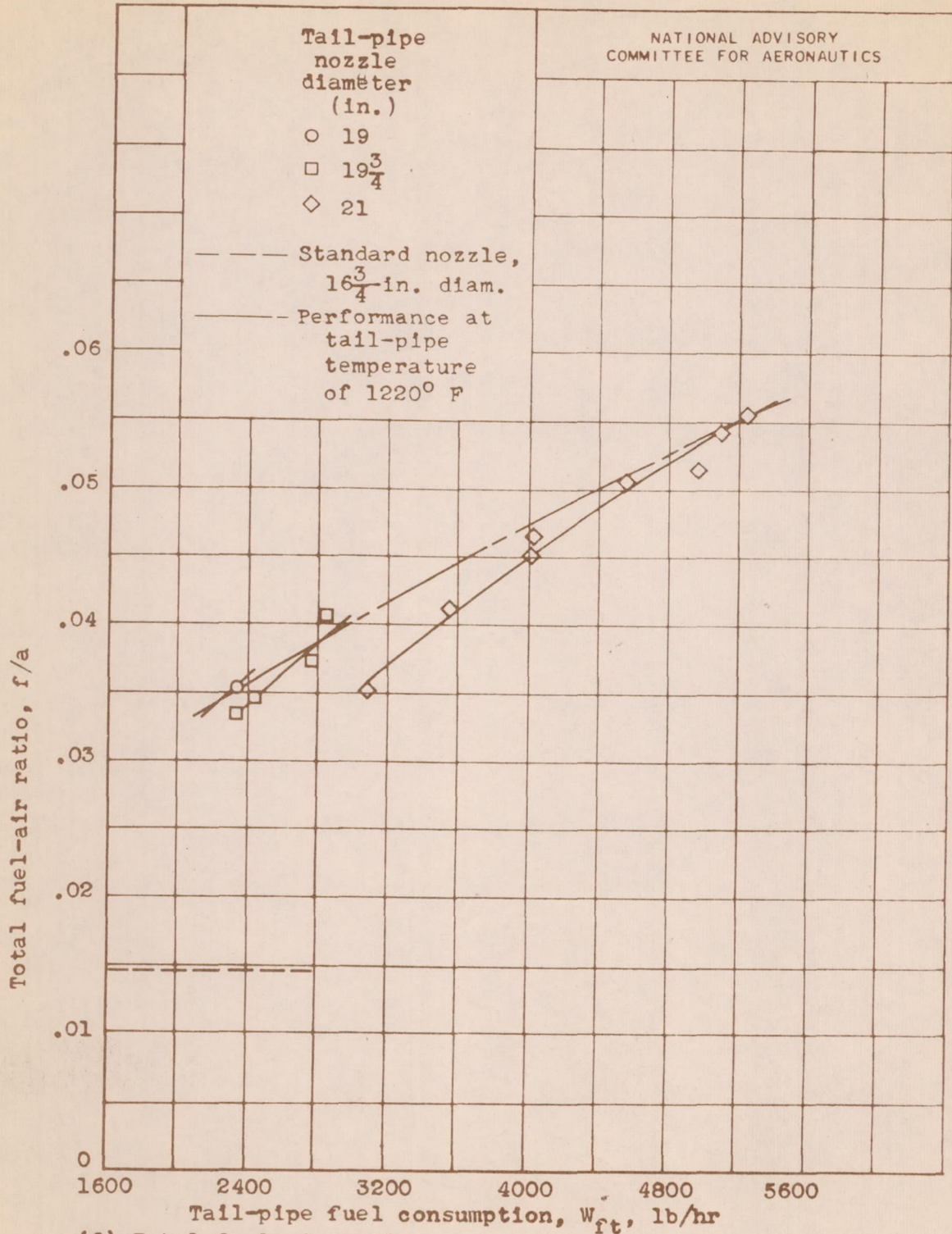
(f) Total fuel-air ratio. Figure 6.- Continued. Variation of turbojet engine performance with tail-pipe fuel consumption for three tail-pipe nozzle diameters. Engine speed, 7600 rpm; altitude, 30,000 feet; ram-pressure ratio, 1.66.
