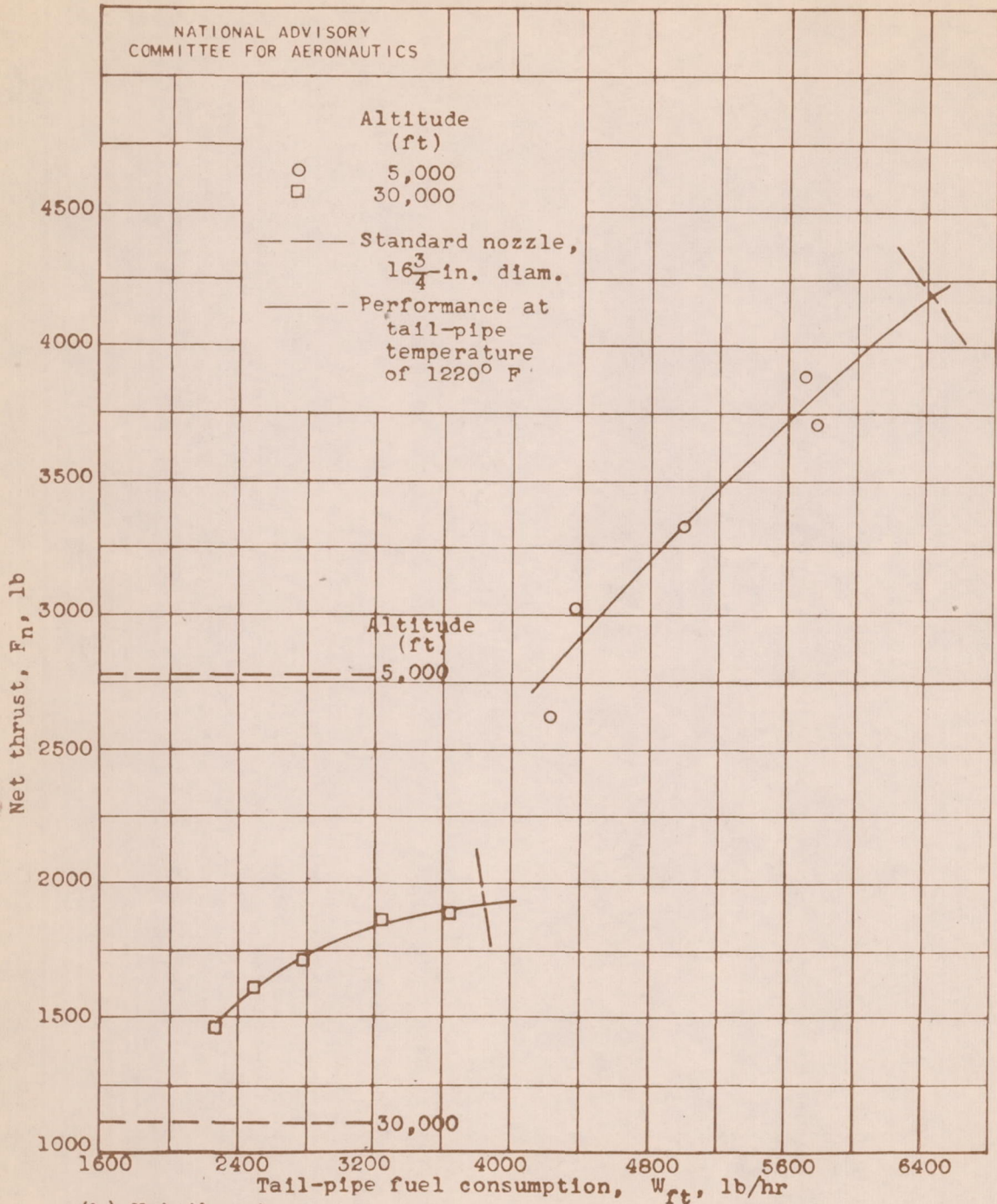
(b) Net thrust.
