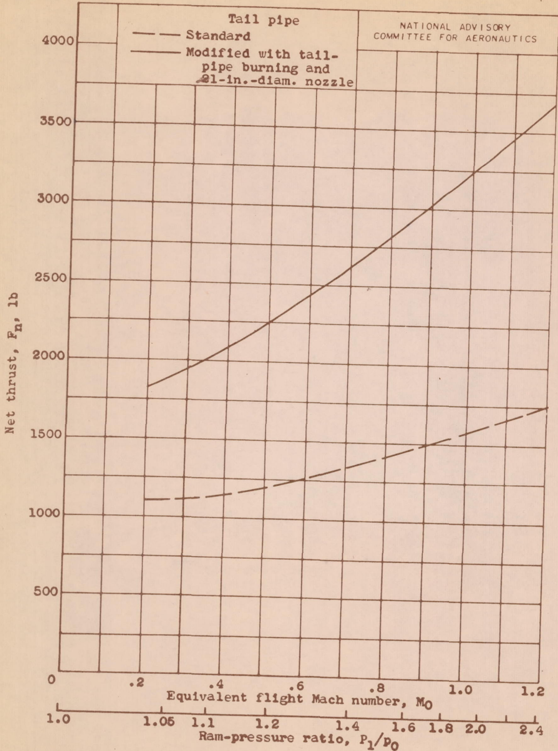
Figure 16.- Relation between equivalent flight Mach number and net thrust of turbojet engine with standard tail pipe and with modified tail pipe and tail-pipe burning. Engine speed, 7600 rpm; turbine-outlet temperature, 1220° F; altitude, 30,000 feet.
