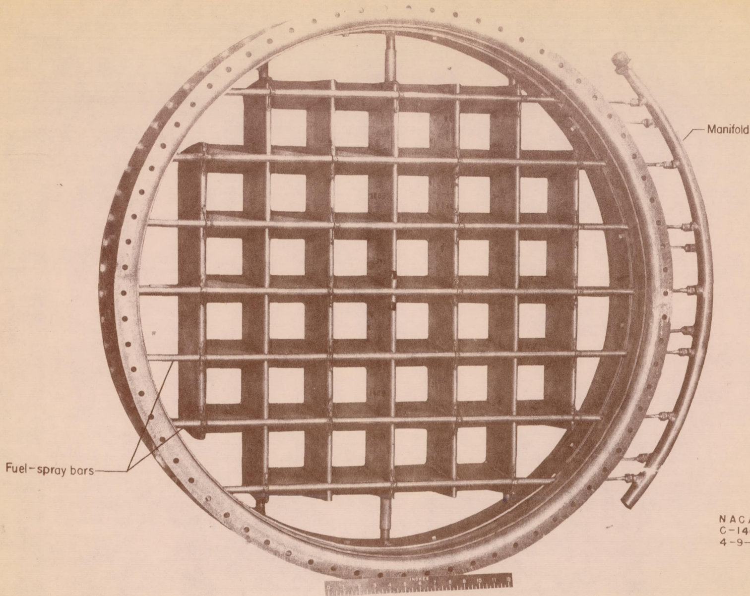
(a) Upstream view of flame holder.
