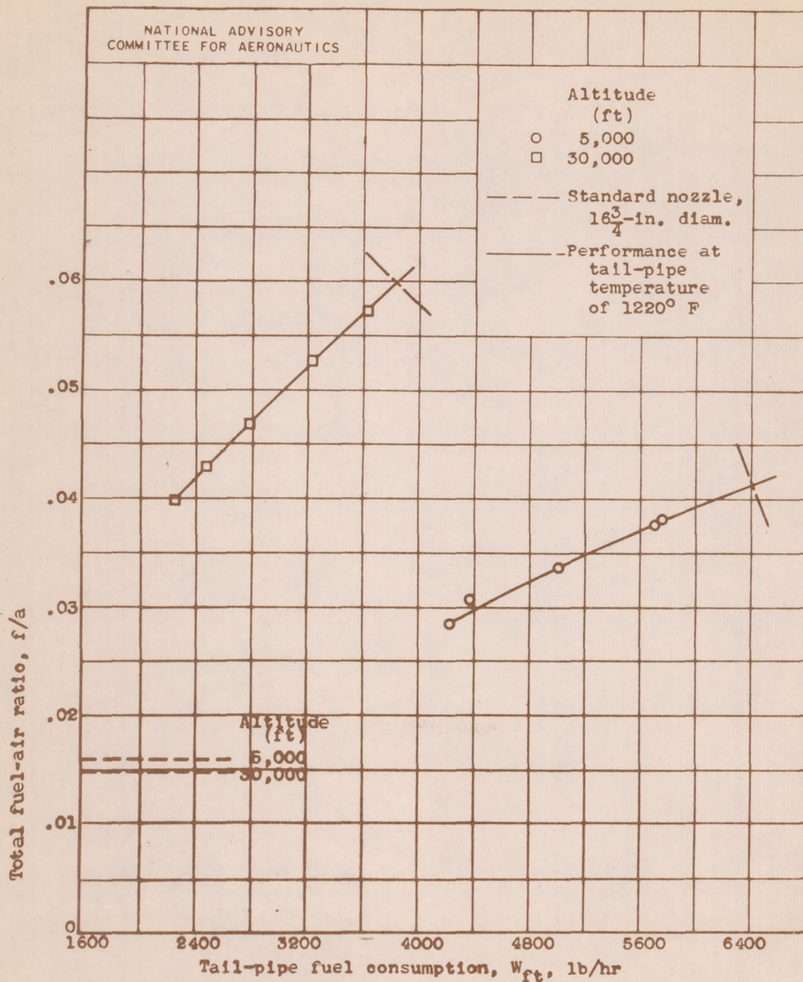
Figure 7.- Continued. Variation of turbojet engine performance with tail-pipe fuel consumption for two altitudes. Engine speed, 7600 rpm; ram-pressure ratio, 1.045; 21-inch-diameter tail-pipe nozzle.
