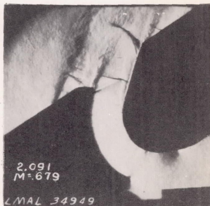
Figure 7.- Schlieren photographs of flow through original root section. \xi_r = 0.404 ; \beta = 56.5^\circ . Upper numbers indicate chamber pressures in atmospheres; lower numbers, entrance Mach numbers. Choking occurred at an entrance Mach number of 0.67.
