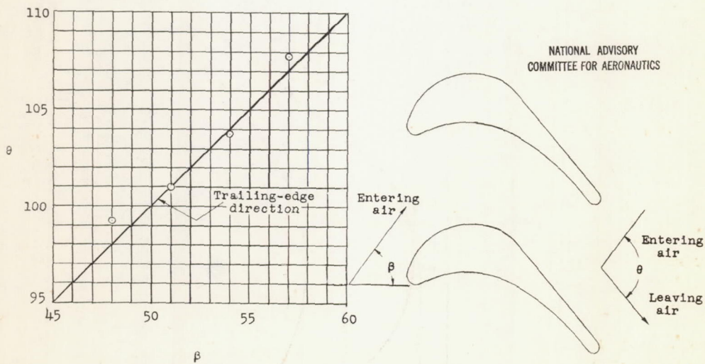
Figure 11.- Velocity distribution and turning angle of original pitch section.
