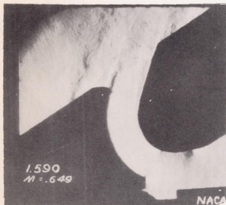
Figure 7.- Schlieren photographs of flow through original root section. \xi_r = 0.404 ; \beta = 56.5^\circ . Upper numbers indicate chamber pressures in atmospheres; lower numbers, entrance Mach numbers. Choking occurred at an entrance Mach number of 0.67.
