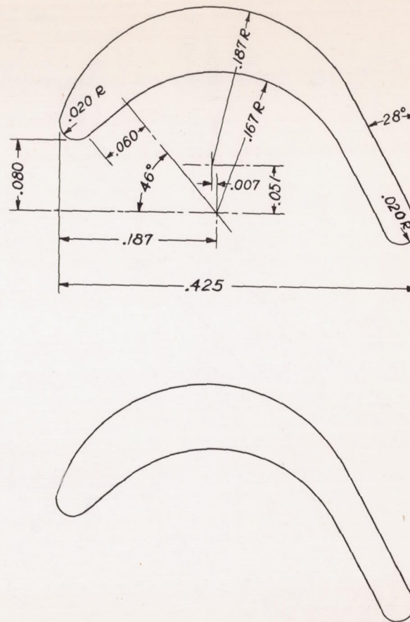
Figure 16.- Bucket tip section designed by NACA. All dimensions are in inches.
