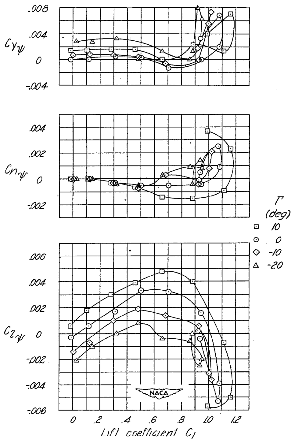
Figure 7.- Effect of dihedral angle on the variation of C_{l\psi} , C_{n\psi} , and C_{y\psi} with lift coefficient for a 45° sweptback wing of aspect ratio 2.61.
