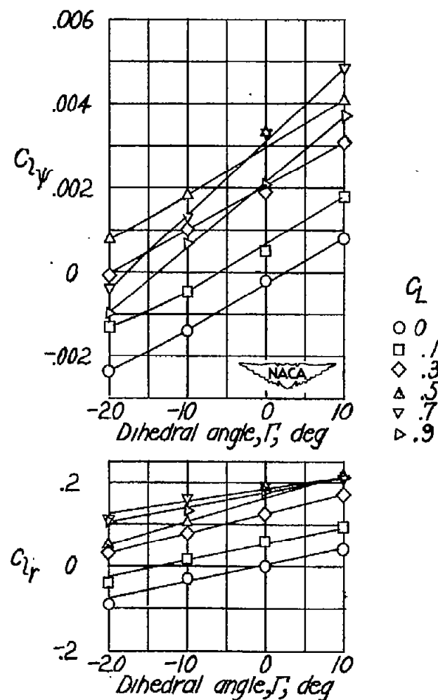
Figure 10.—Variation of C_{Ly} and C_{Lr} with dihedral angle.
