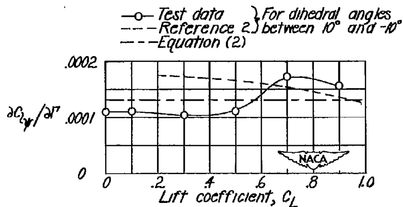
Figure 11.- Variation of \frac{\partial C_L}{\partial \Gamma} and \frac{\partial C_{L_y}}{\partial \Gamma} with lift coefficient for a 45° swept-back wing of aspect ratio 2.61.
