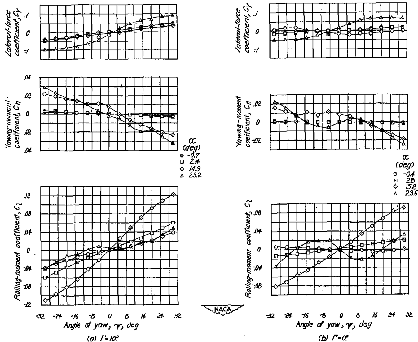
Figure 5.-Basic lateral-stability data of a 45° sweptback wing of aspect ratio 2.61 in straight flow.
