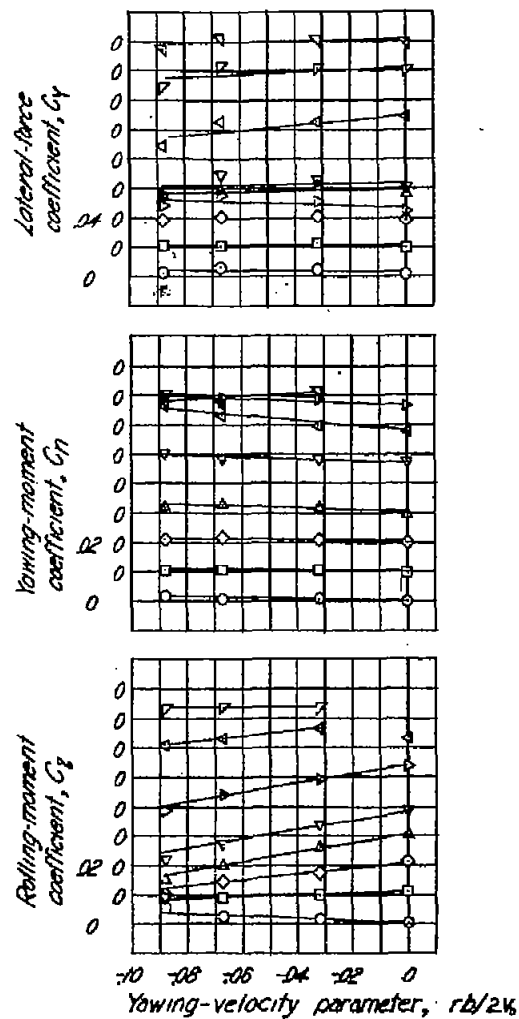
Figure 6.- Basic lateral-stability data of a 45^\circ sweptback wing of aspect ratio 2.61 in yawing flow.
