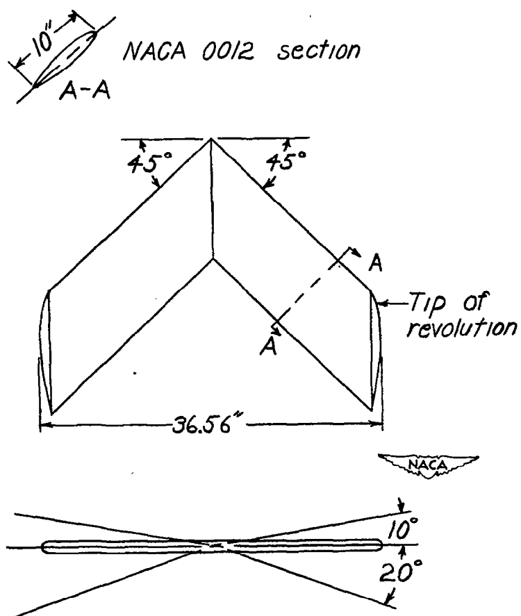
Figure 2.- Diagram of model tested.
