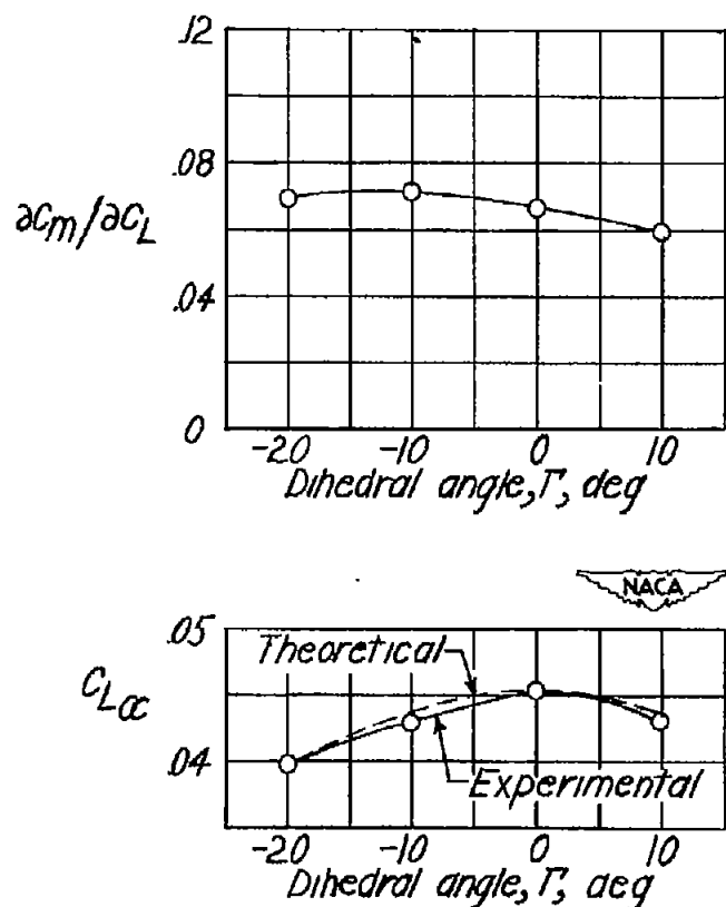
Figure 9.—Variation of C_{L\alpha} and dC_m/d\alpha with dihedral angle for a 45^\circ swept-back wing. A=2.61 ; C_L=0 .
