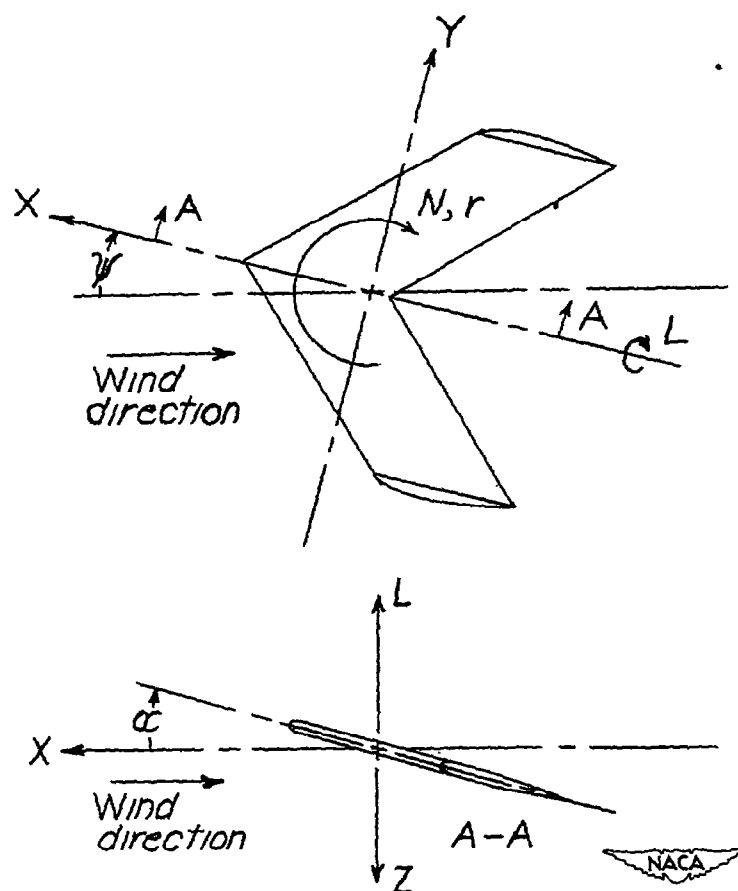
Figure 1.- The stability system of axes. Arrows indicate positive directions of forces, moments, angular velocities, and angular displacements.
