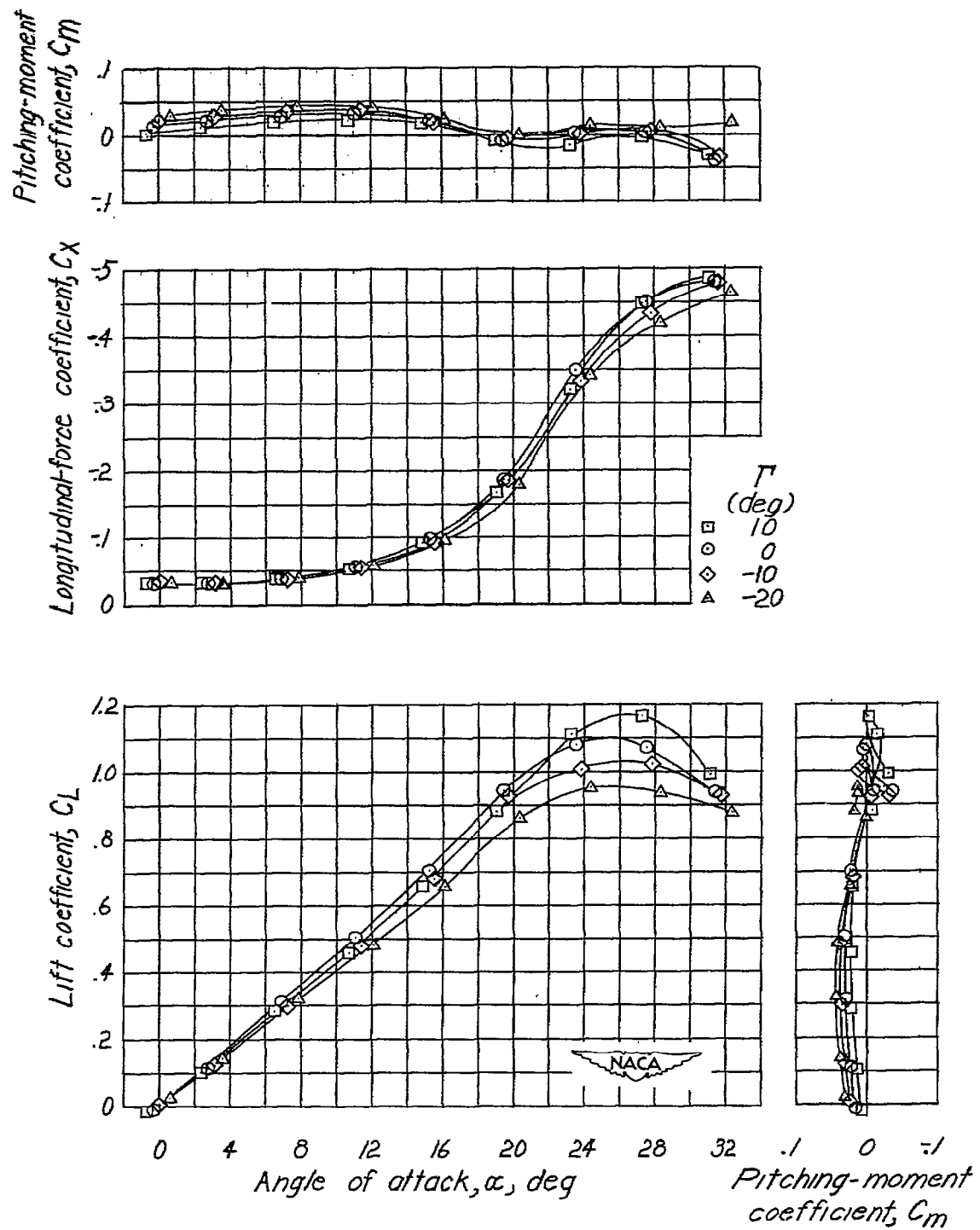
Figure 4.-Basic longitudinal-stability data of a 45^\circ sweptback wing of aspect ratio 2.61 in straight flow. \psi = 0^\circ .
