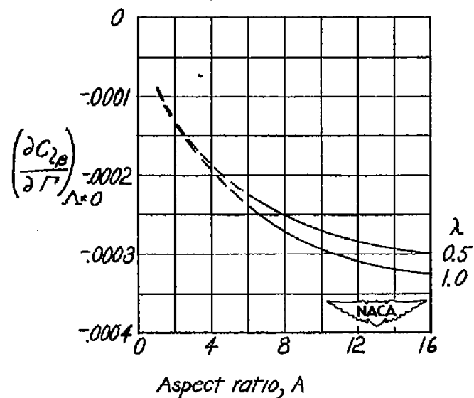
Figure 12.- Chart showing approximate values of the static dihedral-effectiveness parameter \frac{\partial C_{L_\beta}}{\partial \Gamma} for unswept wings: \alpha_0 = 5.67 .
