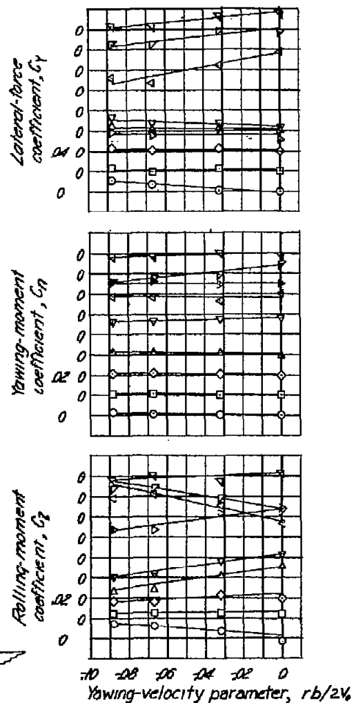
Figure 6.- Basic lateral-stability data of a 45^\circ sweptback wing of aspect ratio 2.61 in yawing flow.
