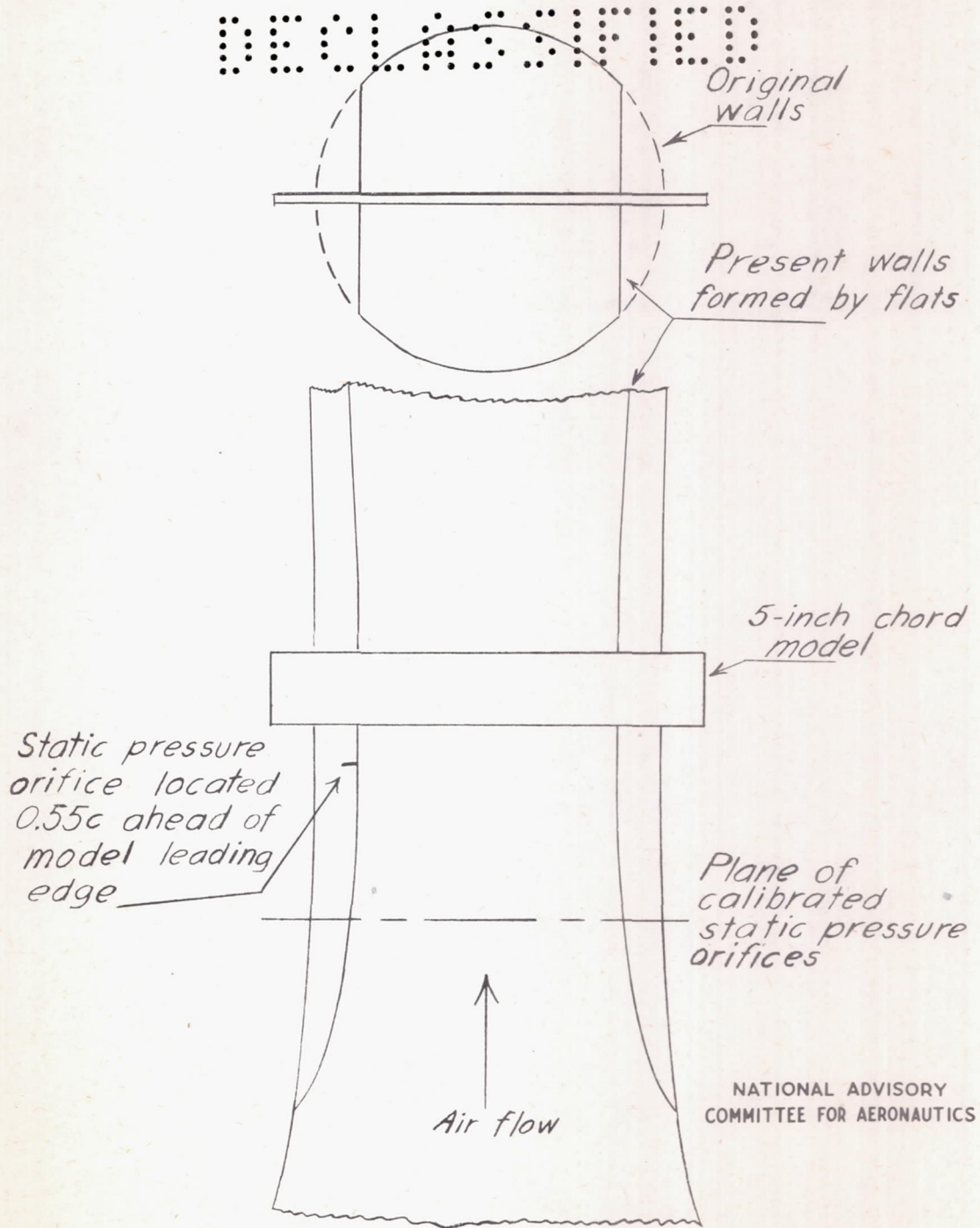
Figure 1. - Modified test section of NACA 24-inch high-speed tunnel.
