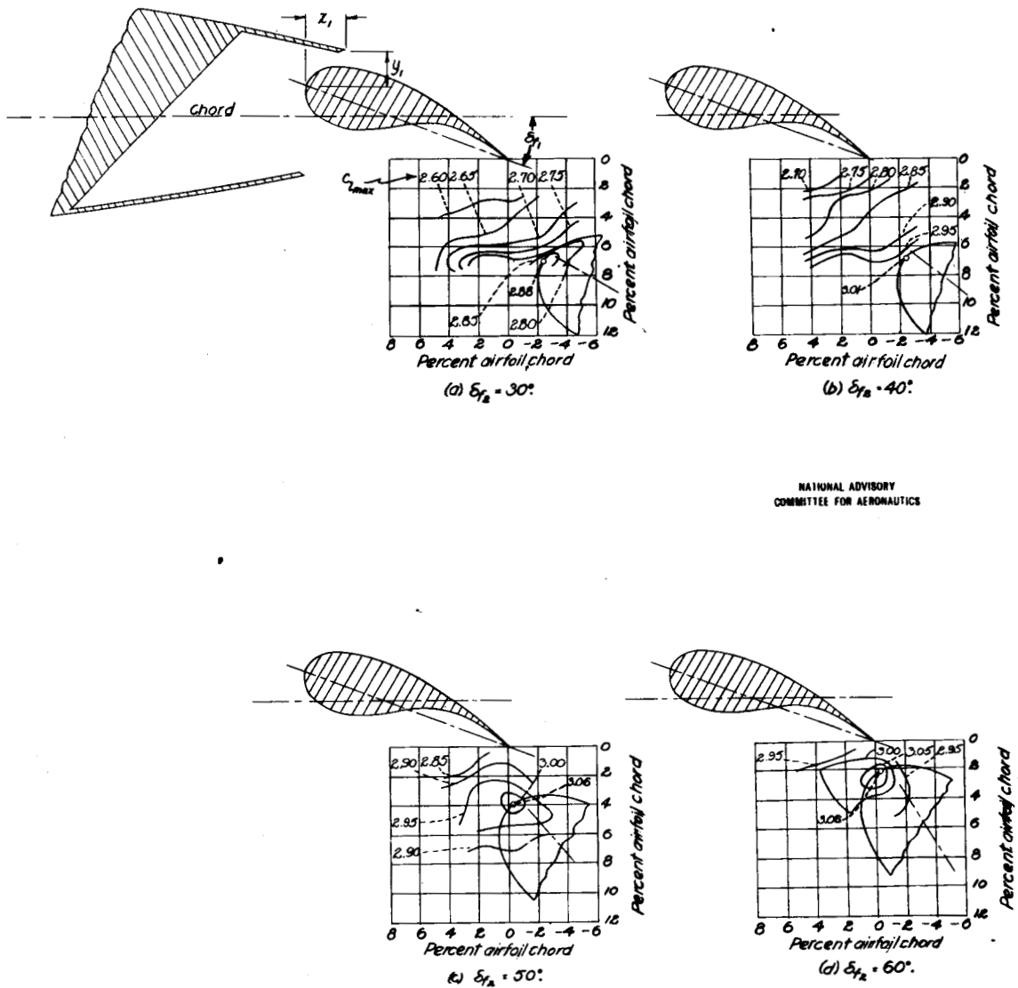
Figure 4.-Contours of rear-flap position for c_{l,max} . Position 2; \delta_f = 20^\circ ; x_f = 2.70 ; y_f = 2.45 . (Values of x_f, y_f are given in percent airfoil chord)
