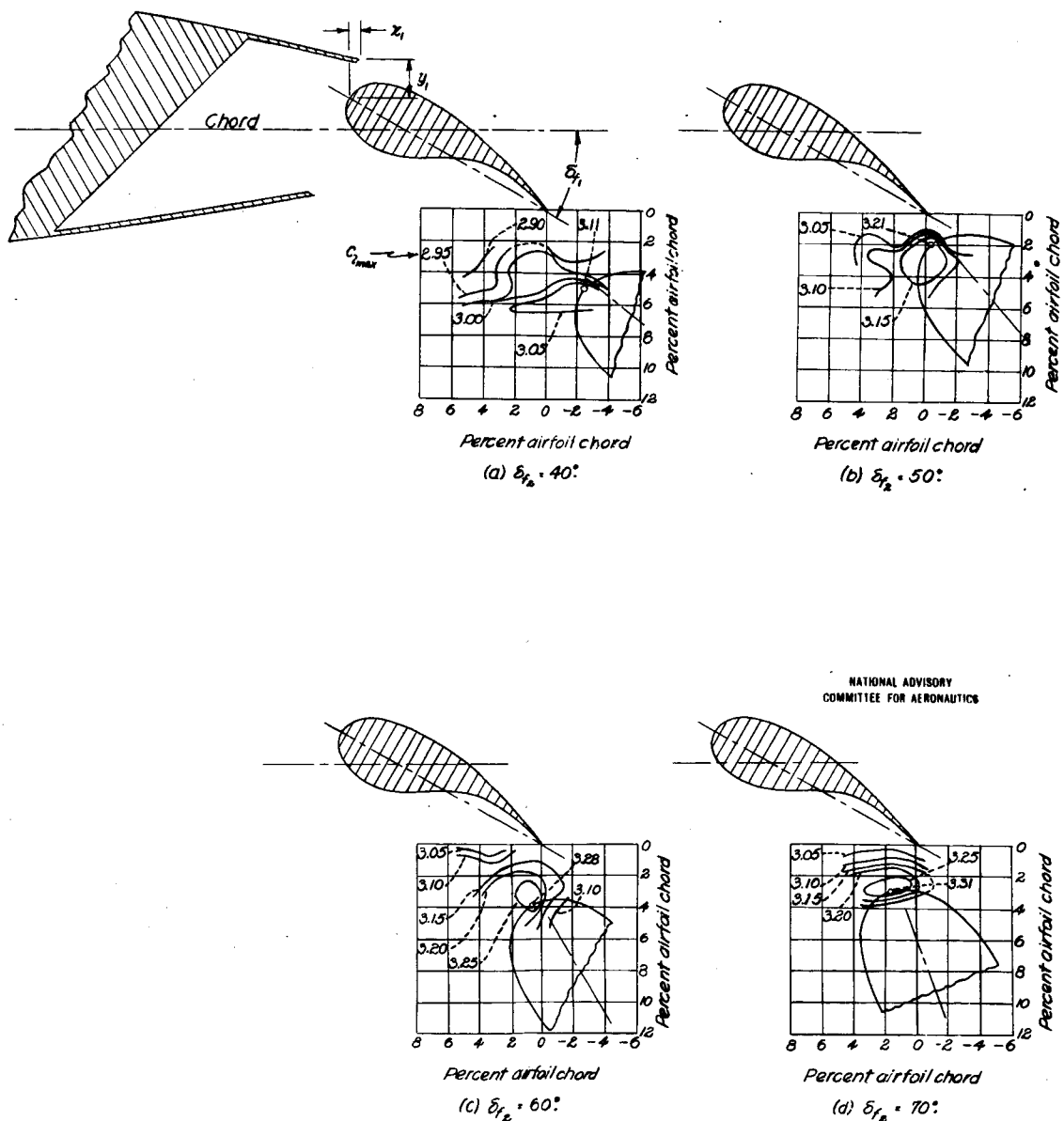
Figure 5-Contours of rear-flap position for C_{2,max} . Position 3; \delta_{f_1} = 30^\circ ; x_{f_1} = 0.70 ; y_{f_1} = 2.45 . (Values of x_i, y_i are given in percent airfoil chord.)
