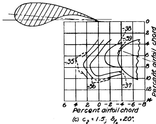
Figure 9:- Contours of rear-flap position for C_{m(a,c)_0} . Position 1, \delta_{f_1} = 5^\circ; \alpha_1 = 3.70; y_1 = 3.45 . (Values of \alpha_1, y_1 are given in percent airfoil chord.)
