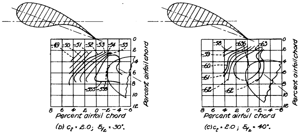
Figure 10- Contours of rear-flap position for C_{mac,h} . Position 2; \delta_{f_1} = 20^\circ ; x_1 = 2.70 ; y_1 = 2.45 . (Values of x_1, y_1 are given in percent airfoil chord)
