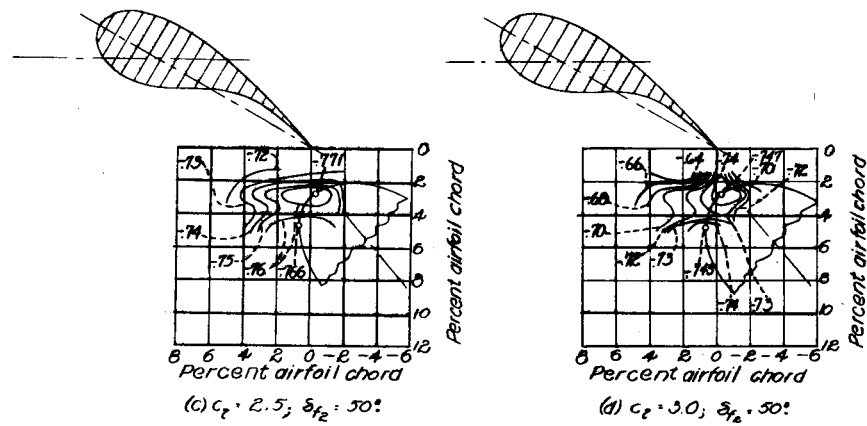
Figure 11.-Contours of rear-flap position for c_{m_{ac}} . Position 3; \delta_{f_1} = 30^\circ; x_1 = 0.70; y_1 = 2.45 . (Values of x_1, y_1 are given in percent airfoil chord.)
