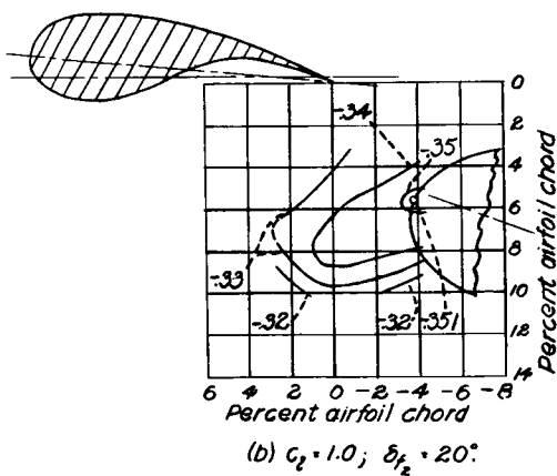
Figure 9:- Contours of rear-flap position for C_{m(a,c)_0} . Position 1, \delta_{f_1} = 5^\circ; \alpha_1 = 3.70; y_1 = 3.45 . (Values of \alpha_1, y_1 are given in percent airfoil chord.)
