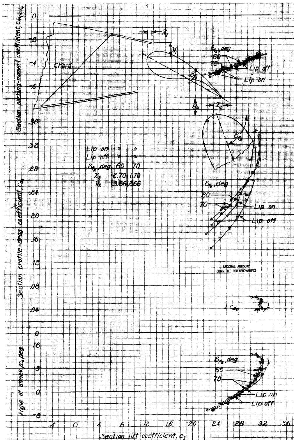
Figure 25-Aerodynamic section characteristics of the NACA 23021 airfoil with a 0.32c double slotted flap showing the effect of removing the airfoil lower lip. Position 3, \delta_f = 30^\circ ; x_1 = 0.170 ; y_1 = 2.43 . (Values of x_1 , y_1 , and x_2 , y_2 are given in percent airfoil chord.)
