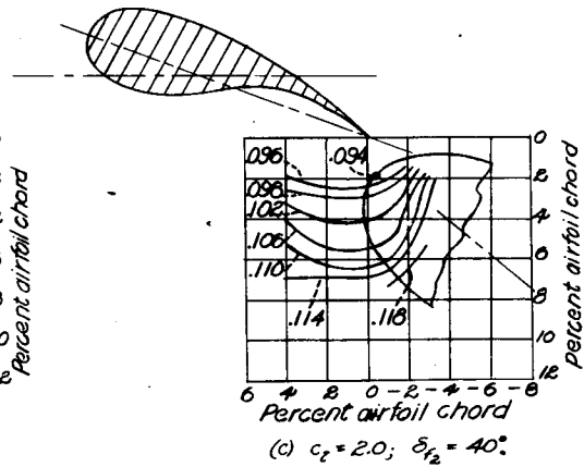
Figure 7.- Contours of rear-flap position for c_{f_2} . Position 2; \delta_{f_1} = 20^\circ ; x_1 = 2.70 ; y_1 = 2.45 . (Values of x_1, y_1 are given in percent airfoil chord.)
