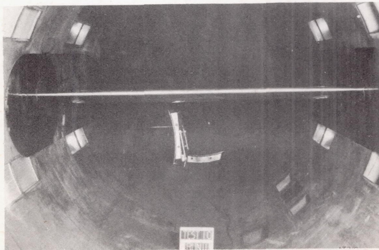
Figure 1.- The 24-inch NACA 23012-64 airfoil mounted in the 8-foot high-speed wind tunnel.
