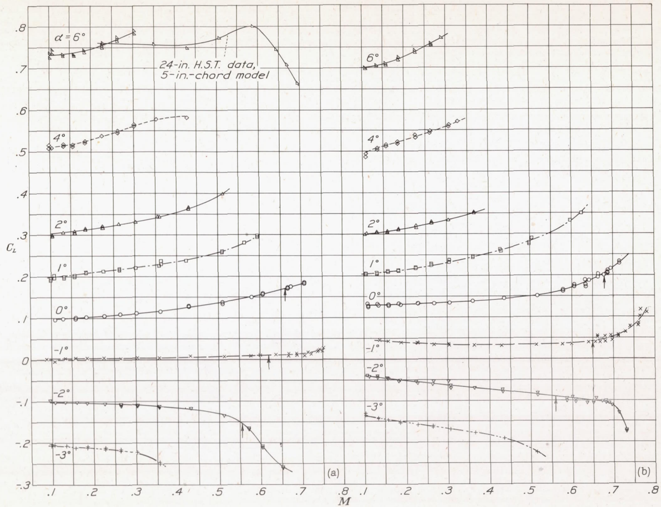
(b) NACA 23012-64 airfoil.
