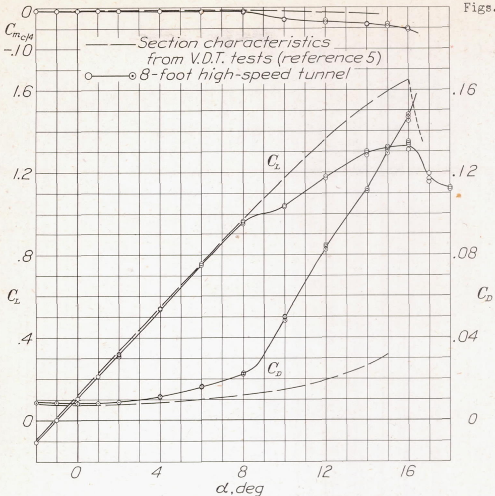
Figure 2.- Comparison of results from the 8-foot high-speed and variable-density wind-tunnels to show magnitude of interference effect due to end leakage in 8-foot high-speed tunnel. M , 0.23 ; R , 3,150,000. NACA 23012 airfoil.
