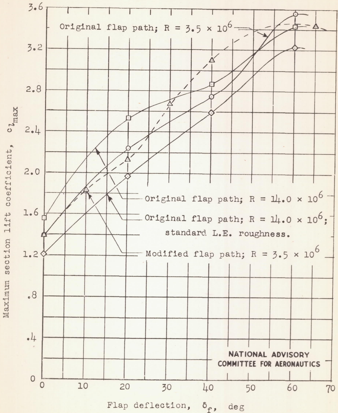
Figure 8.- Maximum section lift coefficients at various flap deflections for both flap paths.
