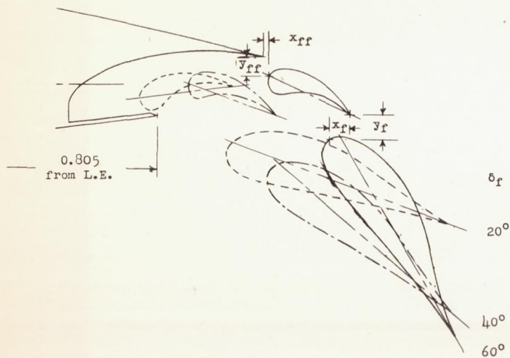
Original Flap Path
