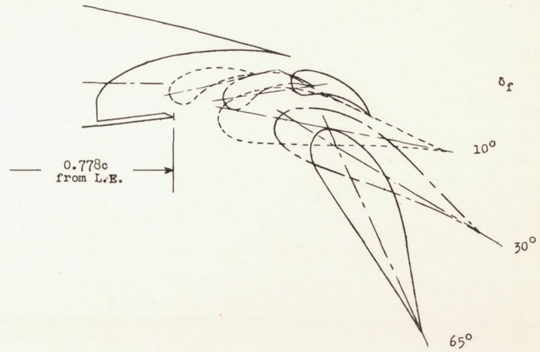
Modified Flap Path
