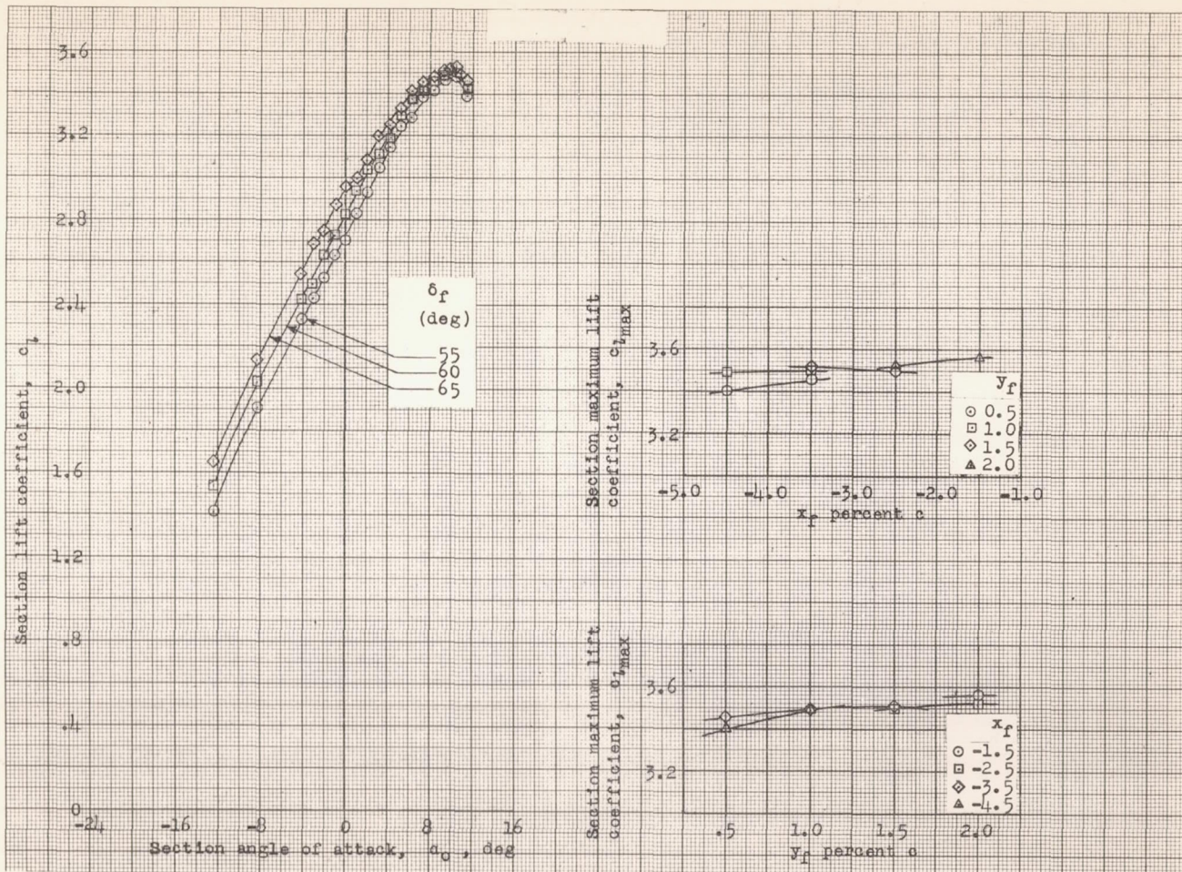
(a) Effect of flap deflection. x_f = -2.5 ; y_f = 1.5
