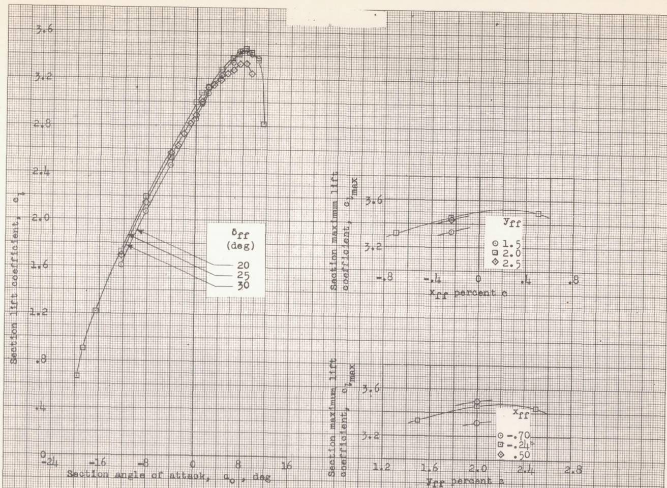
(a) Effect of fore flap deflection. x_{ff} = -0.24 ; y_{ff} = 2.0
