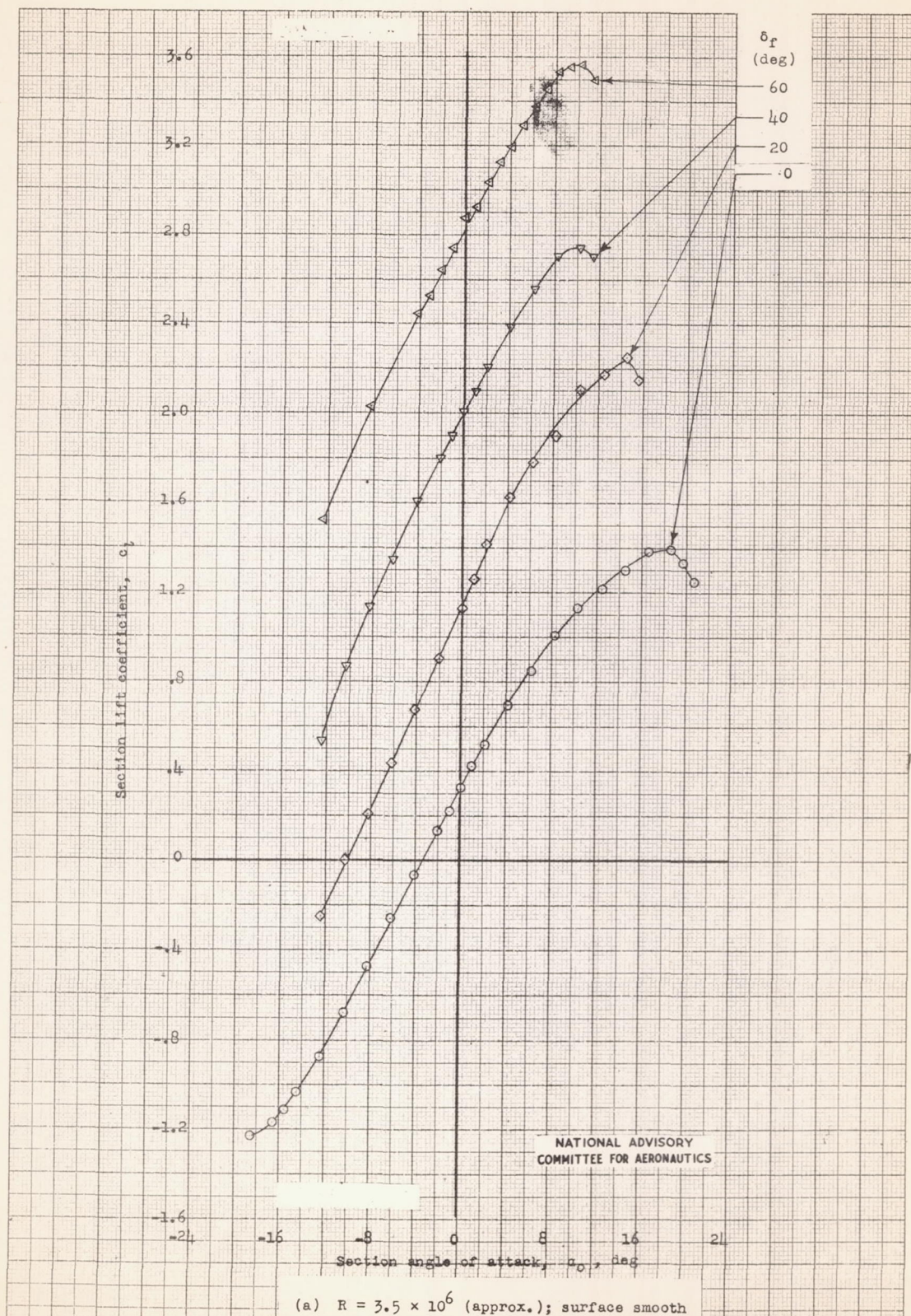
Figure 6.- Lift characteristics of a wing section for the Republic XF-12 airplane equipped with a double slotted flap. Original flap path.
