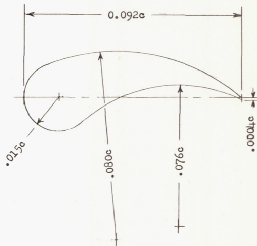
Fore Flap Dimensions
