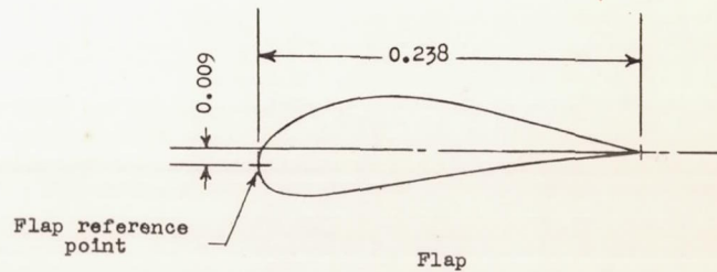
Figure 1 .- Wing, flap, and fore flap; double slotted flap model for Republic XF-12 airplane.
