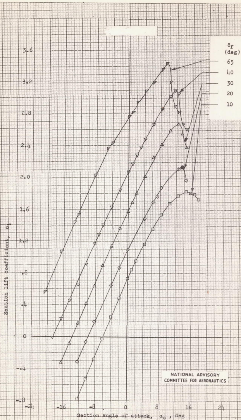
Figure 7.- Lift characteristics of a wing section for the Republic XF-12 airplane equipped with a double slotted flap. Modified flap path. R = 3.5 \times 10^6 (approx.).
