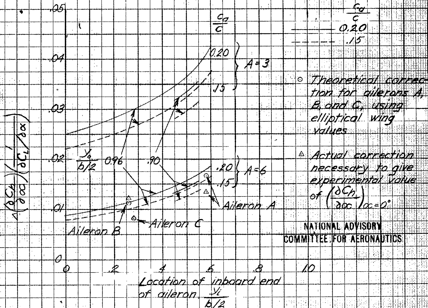
Figure 1.- Theoretical streamline-curvature correction for hinge moments of ailerons having a constant ratio of aileron chord to wing chord on elliptical wings.
