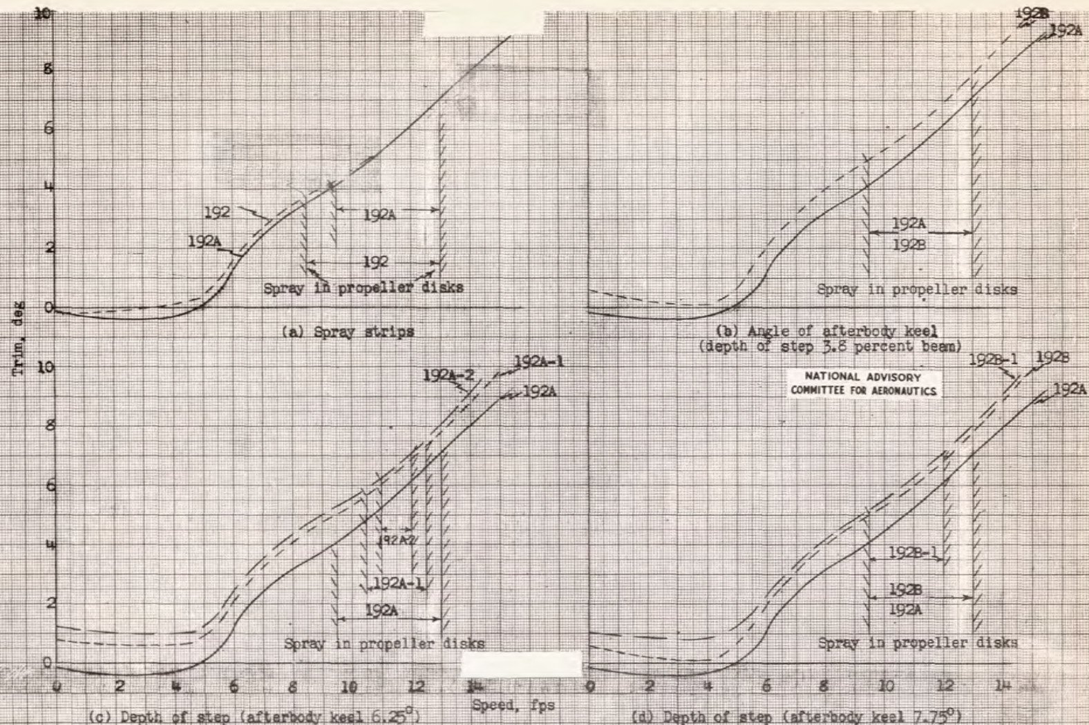
Figure 15.- Model 192. Effect of modifications on the trim, and the duration of spray in the propeller disks; with power (4335 rpm). \Delta_o 71.7 pounds (37,000 pounds, full-size); center of gravity 28 percent mean aerodynamic chord.
