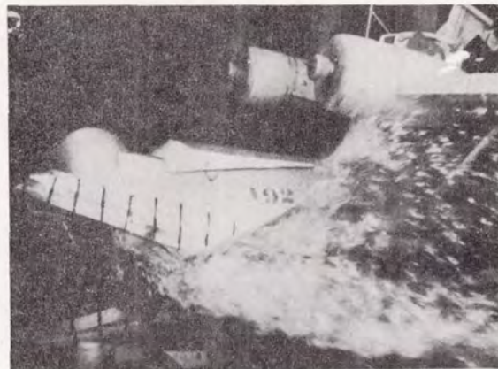
V, 10.0 fps; \tau , 5.8^\circ
