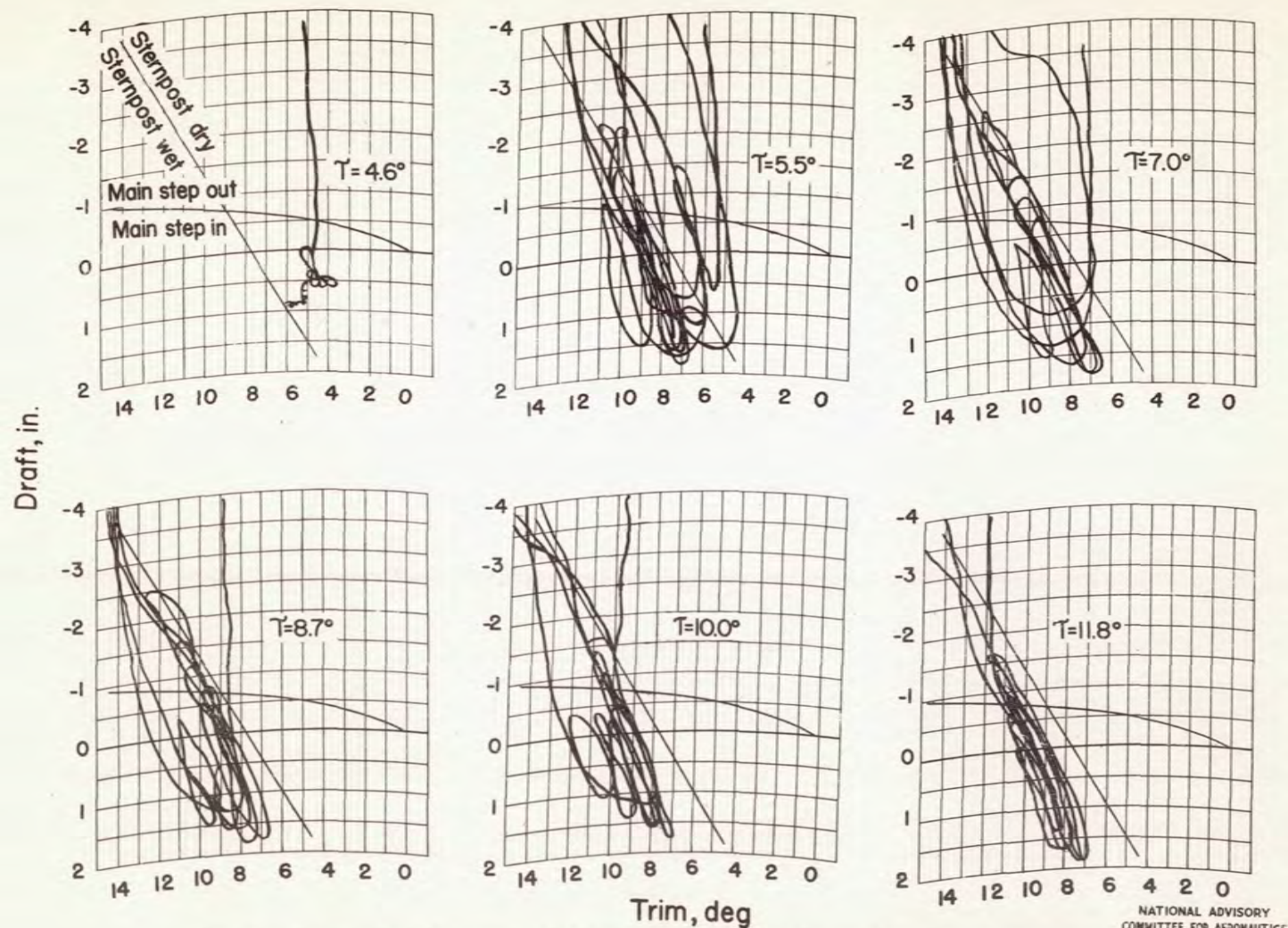
Figure 29.-Model 192B. Variation of trim and draft during landing.
