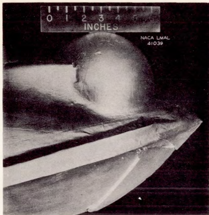
Model 192A.
