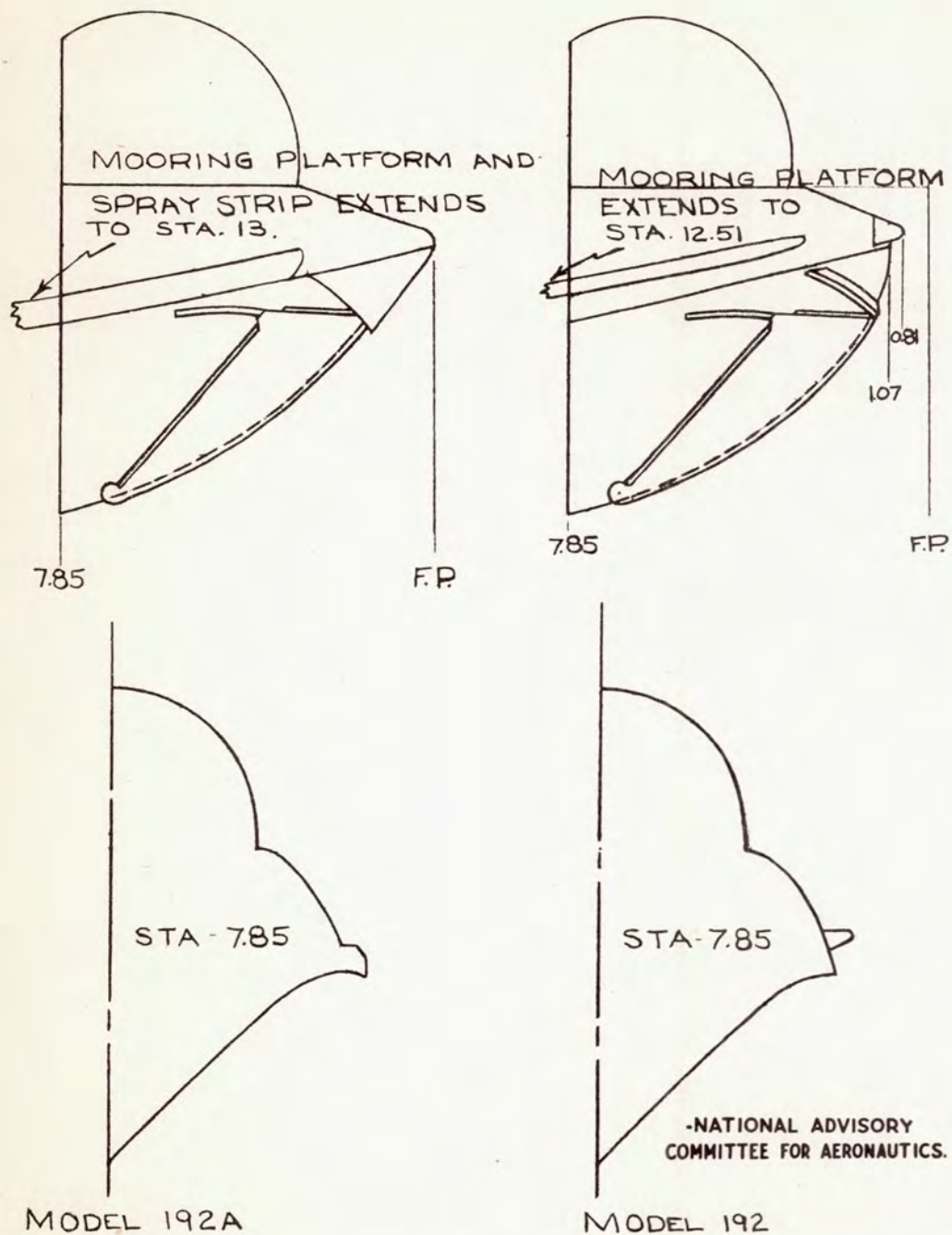
Figure 3(b).-Sketch of bows for models 192 and 192A.
