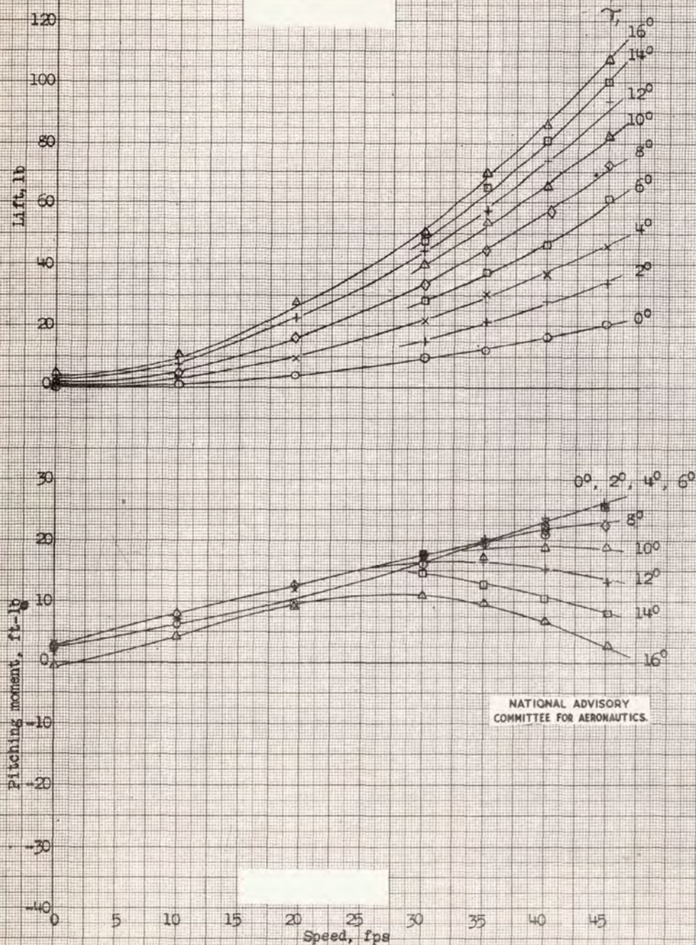
Figure 6.- Model 192.- Concluded.
