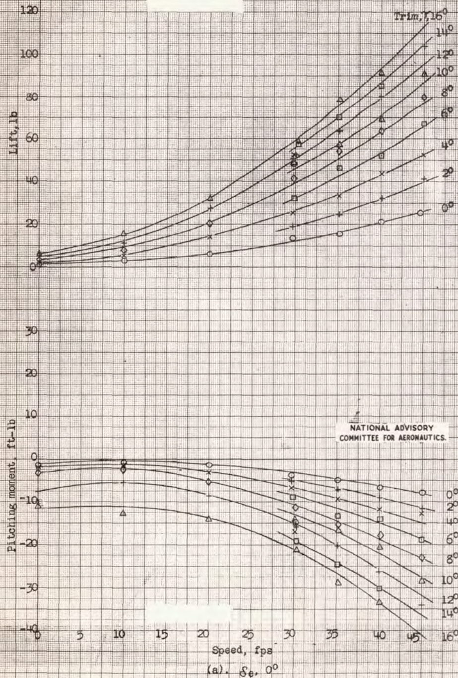
Figure 6.- Model 192. Variation of lift and pitching moment with speed. Power, 4335 rpm; \delta_s, -2^\circ to wing chord.
