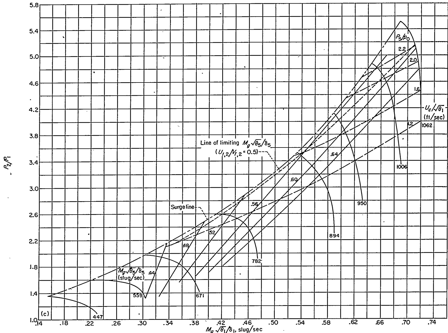
(c) Lines of constant P_3/p_0 and constant M_0\sqrt{\theta_5/\delta_5} ; Y, 0 (flight Mach number, 0).
