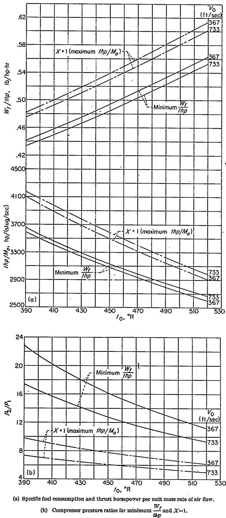
FIGURE 9.—Effects of flight speed and ambient-air temperature on performance at compressor pressure ratios for minimum specific fuel consumption and for maximum thrust horsepower per unit mass rate of air flow; T_1 , 1960° R; \eta_c , 0.85; \eta_t , 0.90; \eta_p , 0.85; \eta_b , 0.96; C_f , 0.97; h , 18,900 Btu per pound; e , 1.00.
