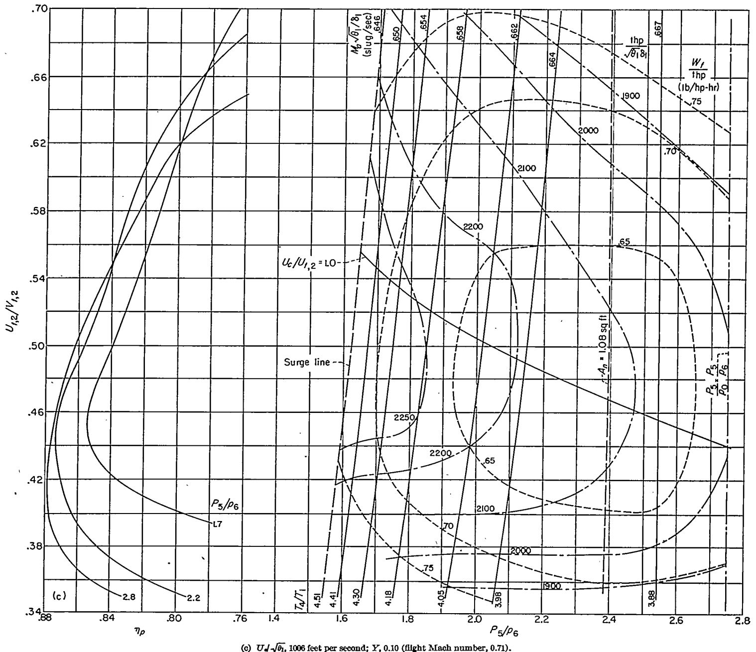
FIGURE 17.—Continued. Total-thrust-horsepower factor and specific fuel consumption of matched turbine-propeller engine; \eta_s , 0.96 C_s , 0.97; h , 18,900 Btu per pound; \Delta P_4/P_1 , 0.03; \Delta P_5/P_1 , 0.05; U_c/U_{t,1} , 1.0.
