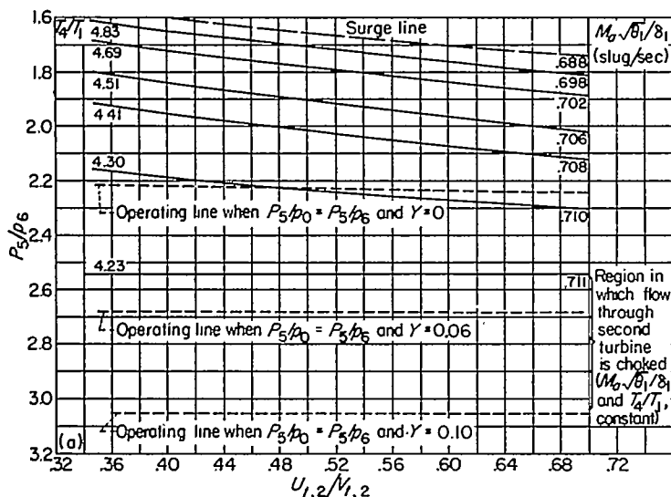
(a) U_d/\sqrt{\theta_1} , 1062 feet per second.
