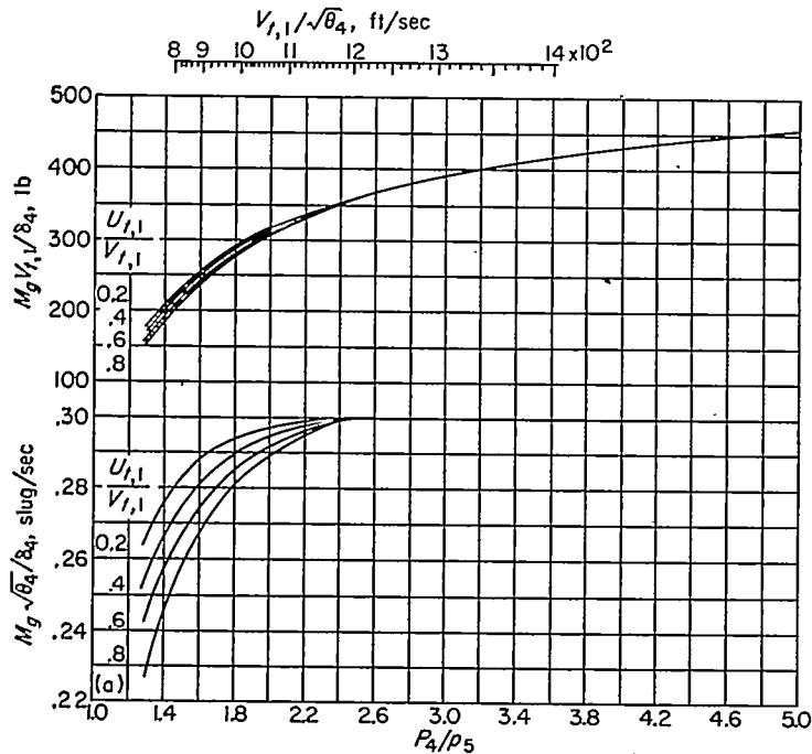
(a) Mass-flow characteristics.
