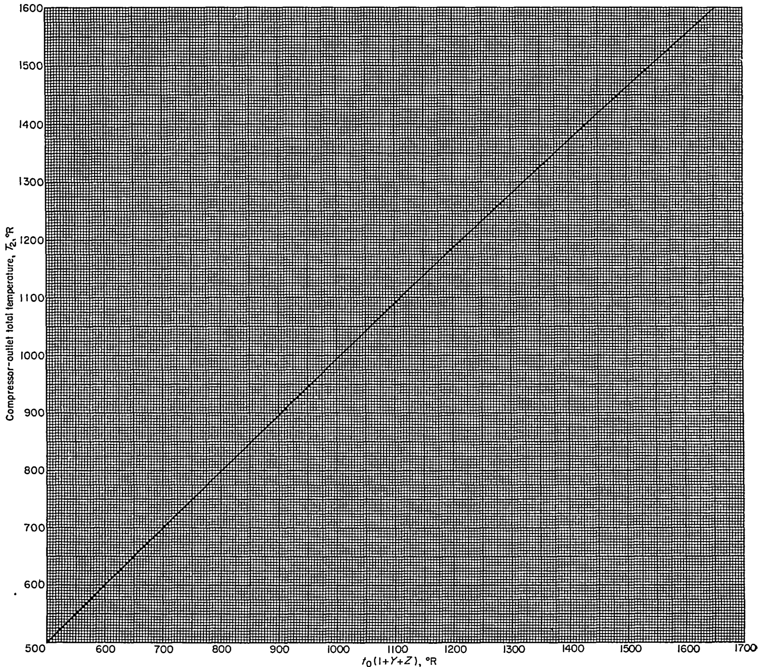
FIGURE 6.—Chart for determining T_3 for various values of t_0(1+Y+Z) .
