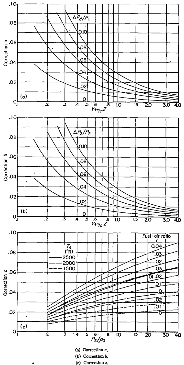
FIGURE 3.—Chart for determining factor \epsilon . ( \epsilon=1-a-b+c )
