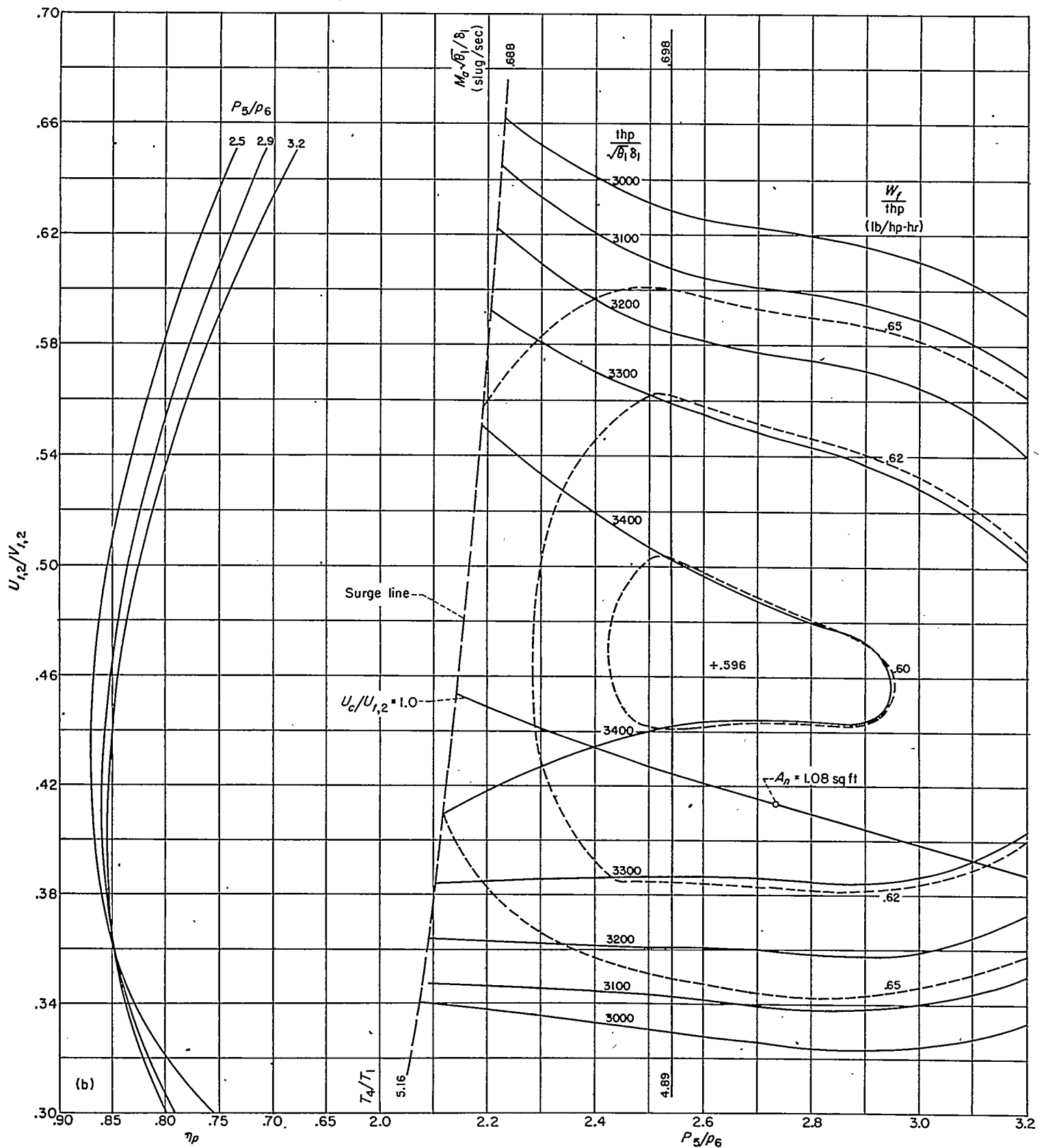
FIGURE 18.—Continued. Performance plots of matched turbine-propeller engine for various values of power output of first turbine to compressor power; U_d \sqrt{\gamma}, 1062 feet per second; Y, 0.10 (flight Mach number, 0.71); \eta_s, 0.96 ; C_s, 0.97 ; h, 18,900 Btu per pound; \Delta P_4/P_1, 0.03 ; \Delta P_2/P_3, 0.05 ; U_d/U_{1,2}, 1.0 .
