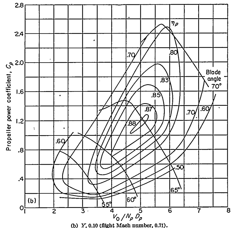
(b) Y, 0.10 (flight Mach number, 0.71). FIGURE 15.—Concluded. Characteristics of high-speed propeller.
