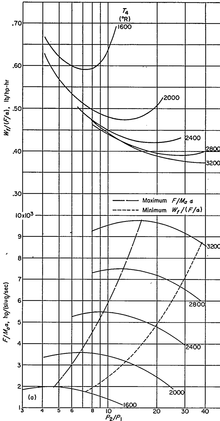
(a) V_0 , 0; t_0 , 519° R; V_1 , 144 feet per second; a , 4 pounds thrust per horsepower (to convert jet thrust to equivalent shaft horsepower).
