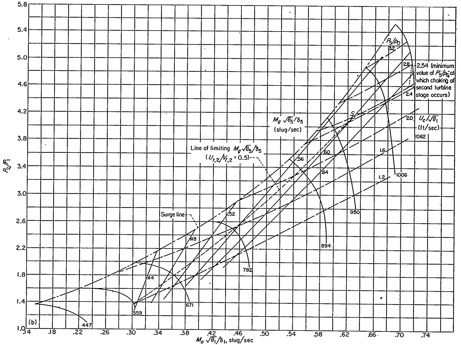
(b) Lines of constant P_4/p_5 and constant M_s\sqrt{\theta_5/\delta_5} ; Y, 0.10 (flight Mach number, 0.71). FIGURE 13.—Continued. Operating characteristics of gas generator consisting of matched compressor and turbine which drives compressor; \Delta P_2/P_2, 0.05 ; U_1/U_{1,2}, 1.0 .
