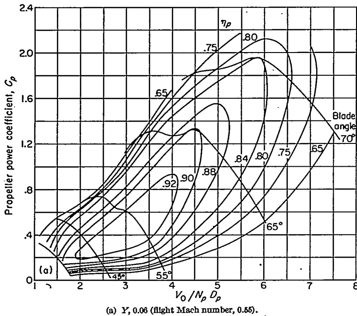
(a) Y, 0.06 (flight Mach number, 0.55). FIGURE 15.—Characteristics of high-speed propeller.
