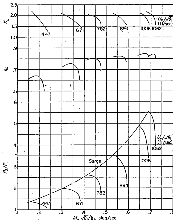
FIGURE 11.—Characteristics of axial-flow compressor.
