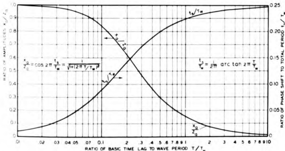
Fig. 5. Sinusoidal fluctuating ground-water pressure
