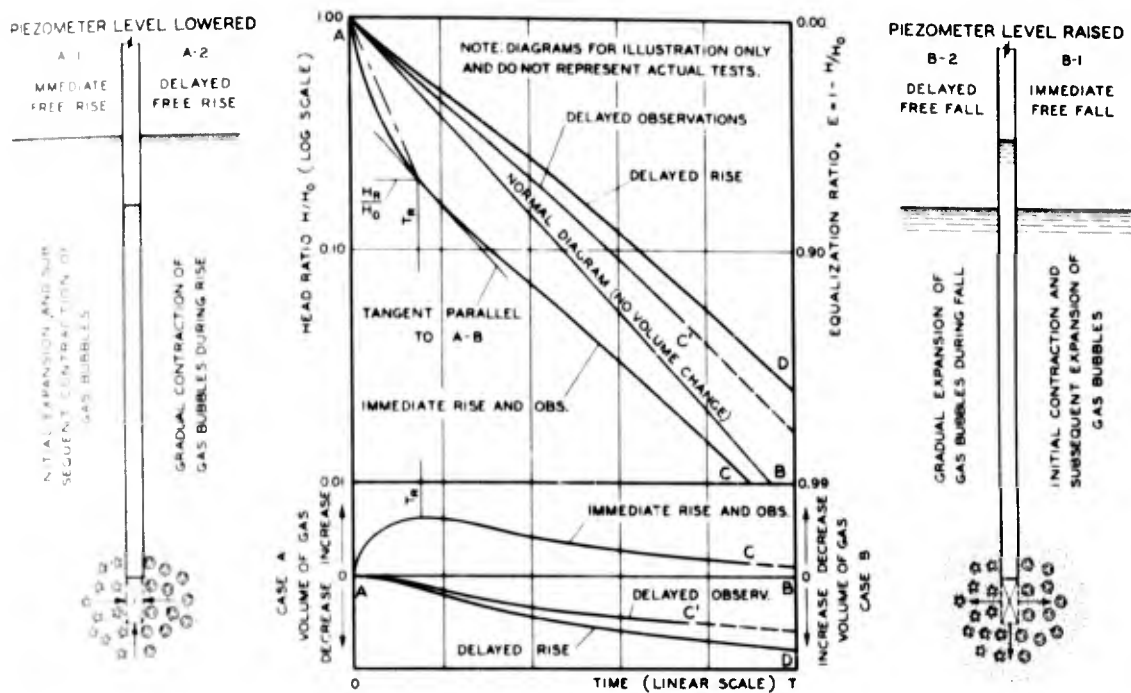
Fig. 11. Influence of volume changes of gas in soil
