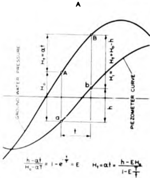
DETERMINATION OF GROUND-WATER PRESSURE METHOD OF LINEAR CHANGE IN PRESSURE
