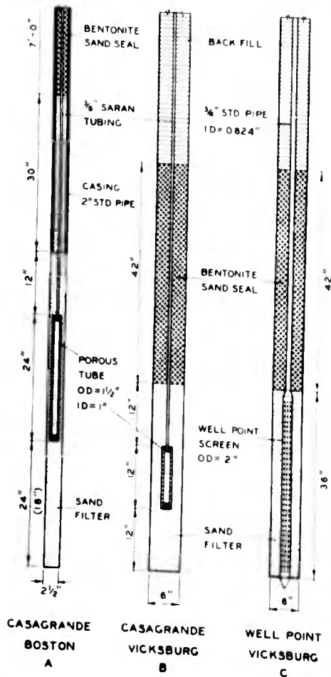
Fig. 15. Piezometers used in tests
