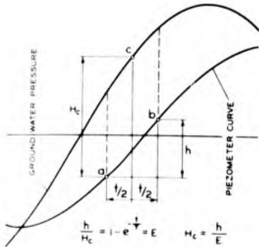
DETERMINATION OF GROUND-WATER PRESSURE METHOD OF EQUIVALENT CONSTANT PRESSURE
