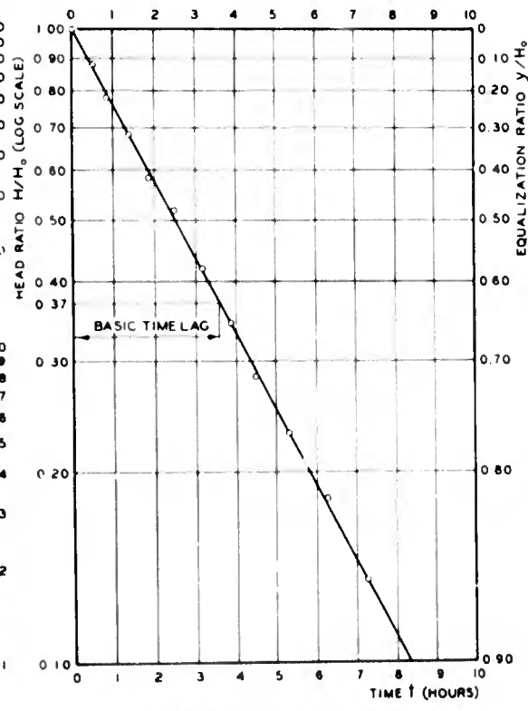
D - DETERMINATION OF BASIC TIME LAG
