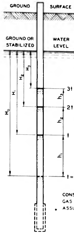
B - OBSERVATIONS AT EQUAL TIME INTERVALS
