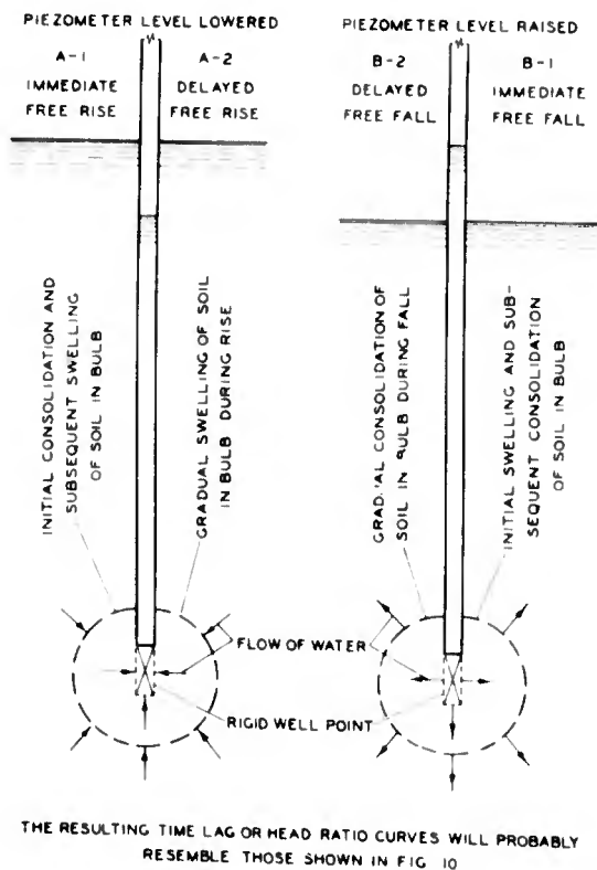
Fig. 9. Transient changes in void ratio
