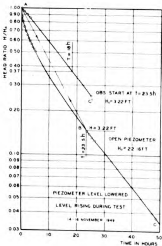
WILLOW POINT PIEZOMETER NO. 1 - CASAGRANDE TYPE FIG. 15-B
