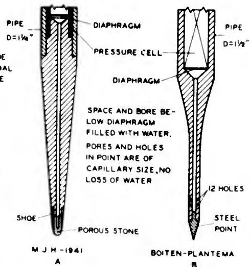
Fig. 8. Points for pressure sounding rod
