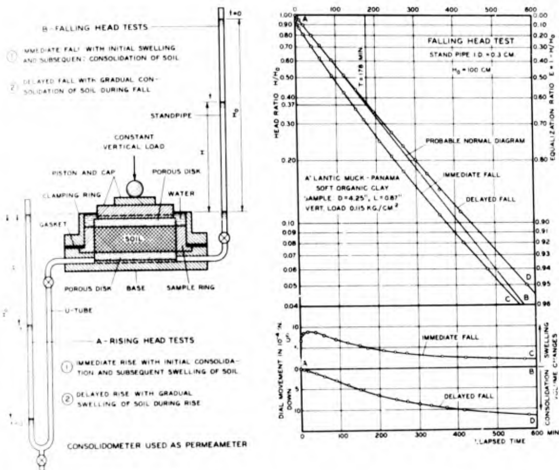
Fig. 10. Volume changes during laboratory permeability tests
