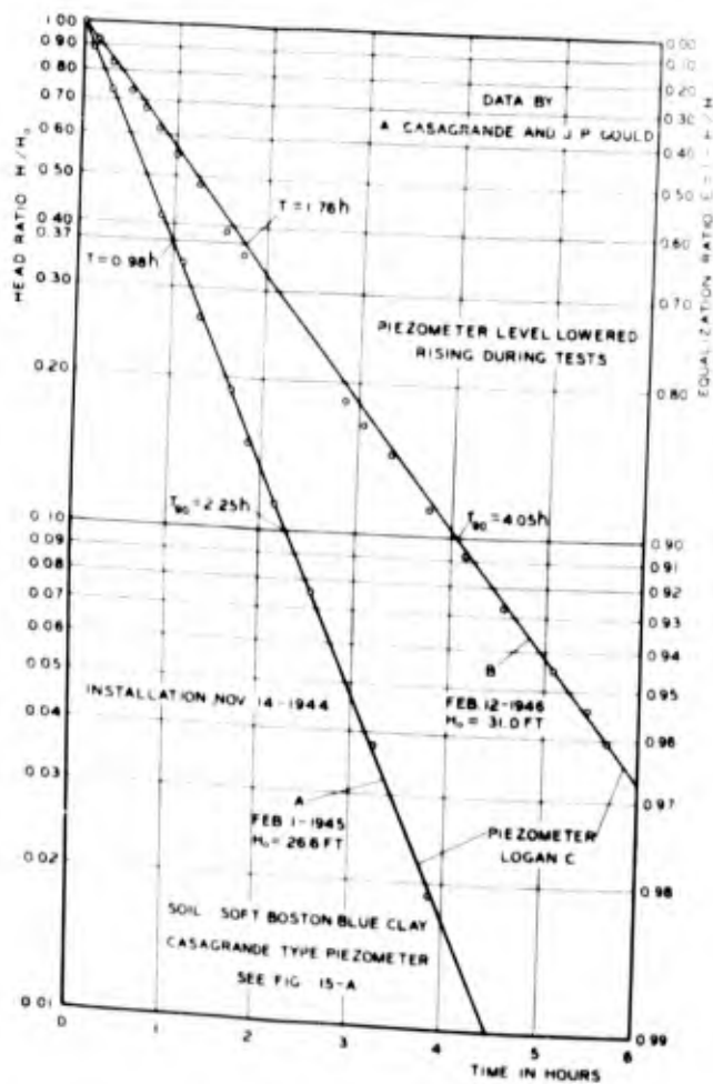
Fig. 16. Time lag tests at Logan Airport, Boston
