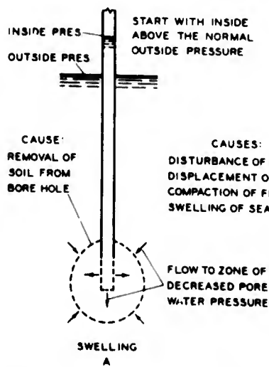
Fig. 7. Initial disturbance and stress changes
