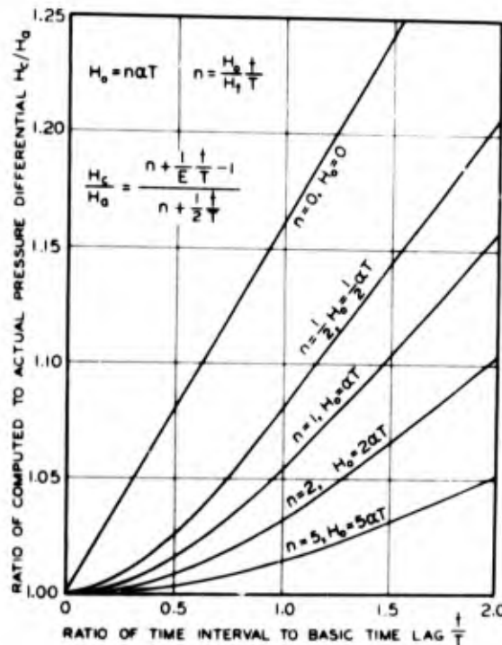
C - RELATIVE ACCURACY OF METHODS
