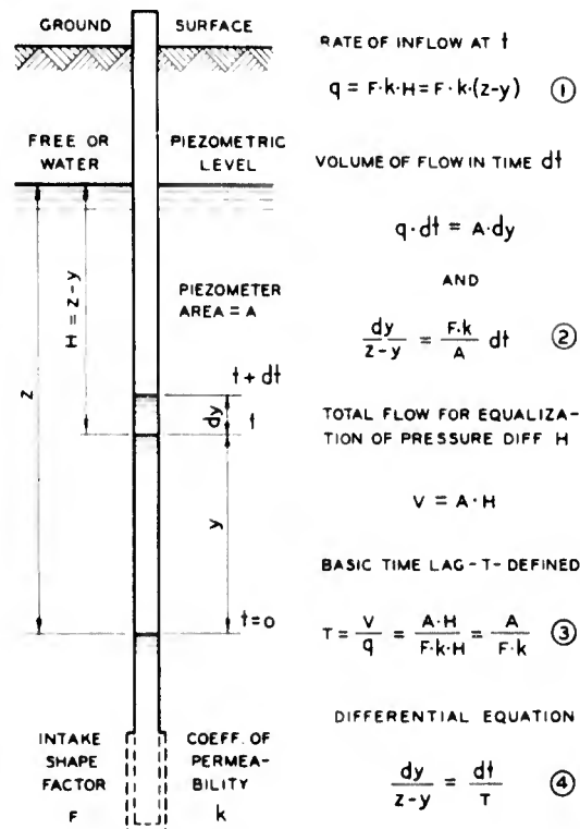
Fig. 2. Basic definitions and equations
