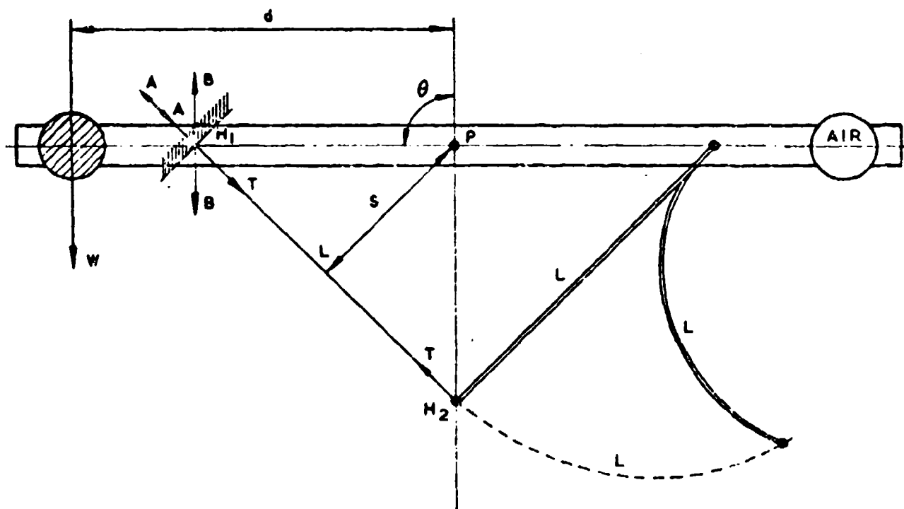
FIGURE 7. REVERSED AND INVERTED LEAF-SPRING SUSPENSION
