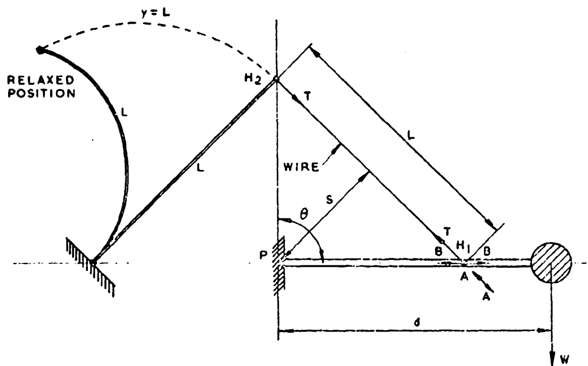
FIGURE 4. APPLICATION OF THE TRIANGULAR CANTILEVER LEAF-SPRING TO THE LA COSTE SUSPENSION
