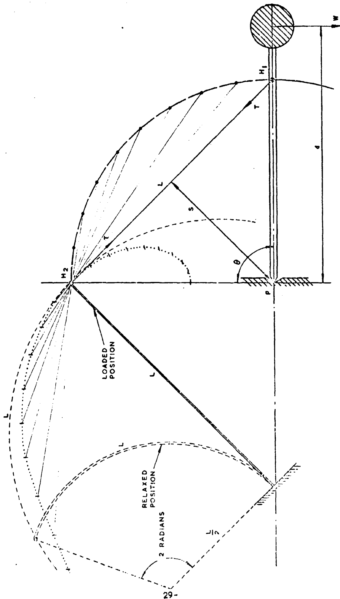
FIGURE 5. ILLUSTRATING THE APPROXIMATIONS INVOLVED IN THE USE OF A LEAF-SPRING
