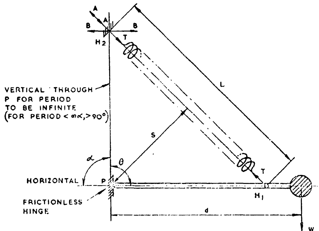
FIGURE 2. THE LACOSTE SUSPENSION
