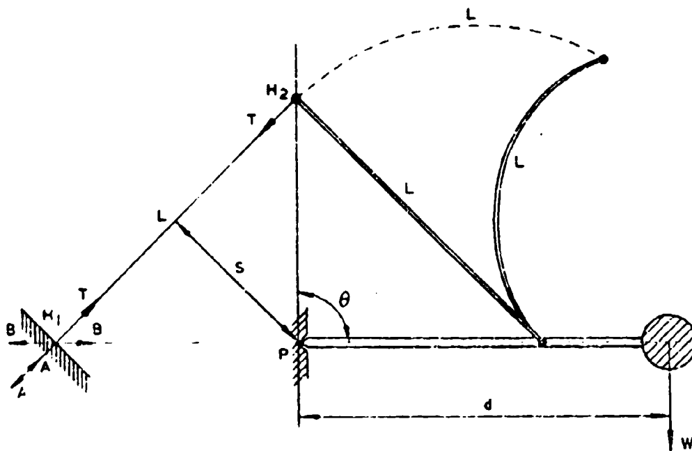
FIGURE 6. REVERSED LEAF-SPRING SUSPENSION
