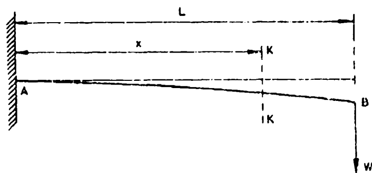
FIGURE 16. A TRIANGULAR CANTILEVER CLAMPED AT ITS BASE
