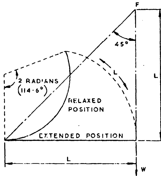
FIGURE 3. THE OPERATION OF A TRIANGULAR CANTILEVER LEAF - SPRING
