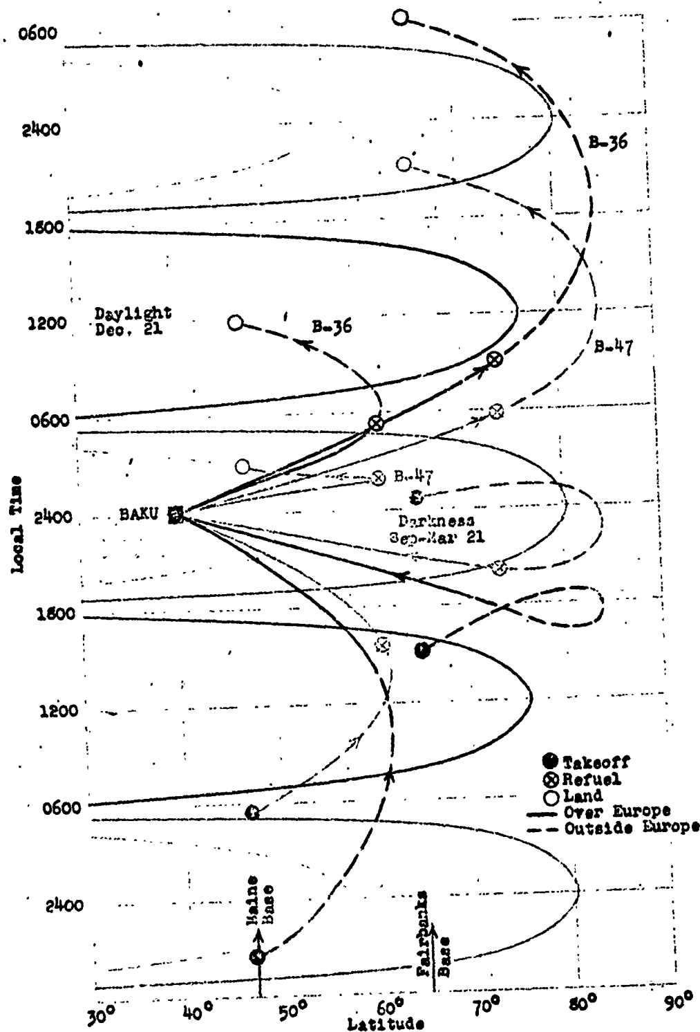
FIG. 10 HOURS OF DAYLIGHT OVER EUROPE AT 40,000 FT. Attacks On Far Targets
