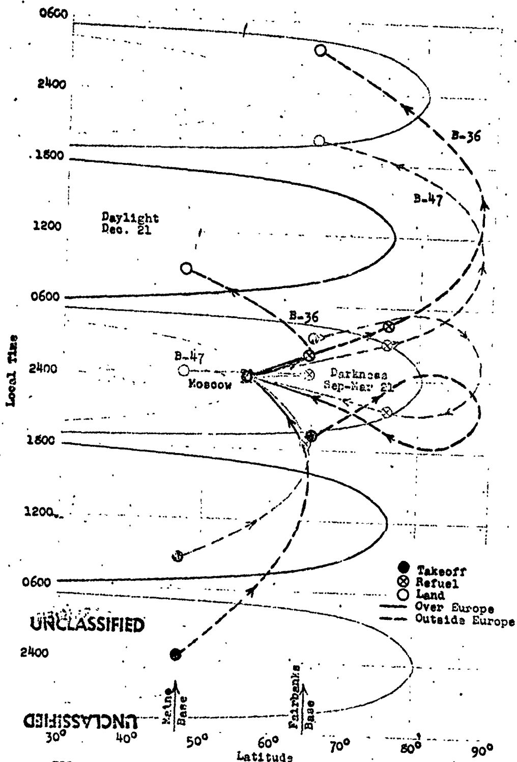
FIG. 9 HOURS OF DARKNESS OVER EUROPE AT 40,000 F.A. Attacks On Near Targets
