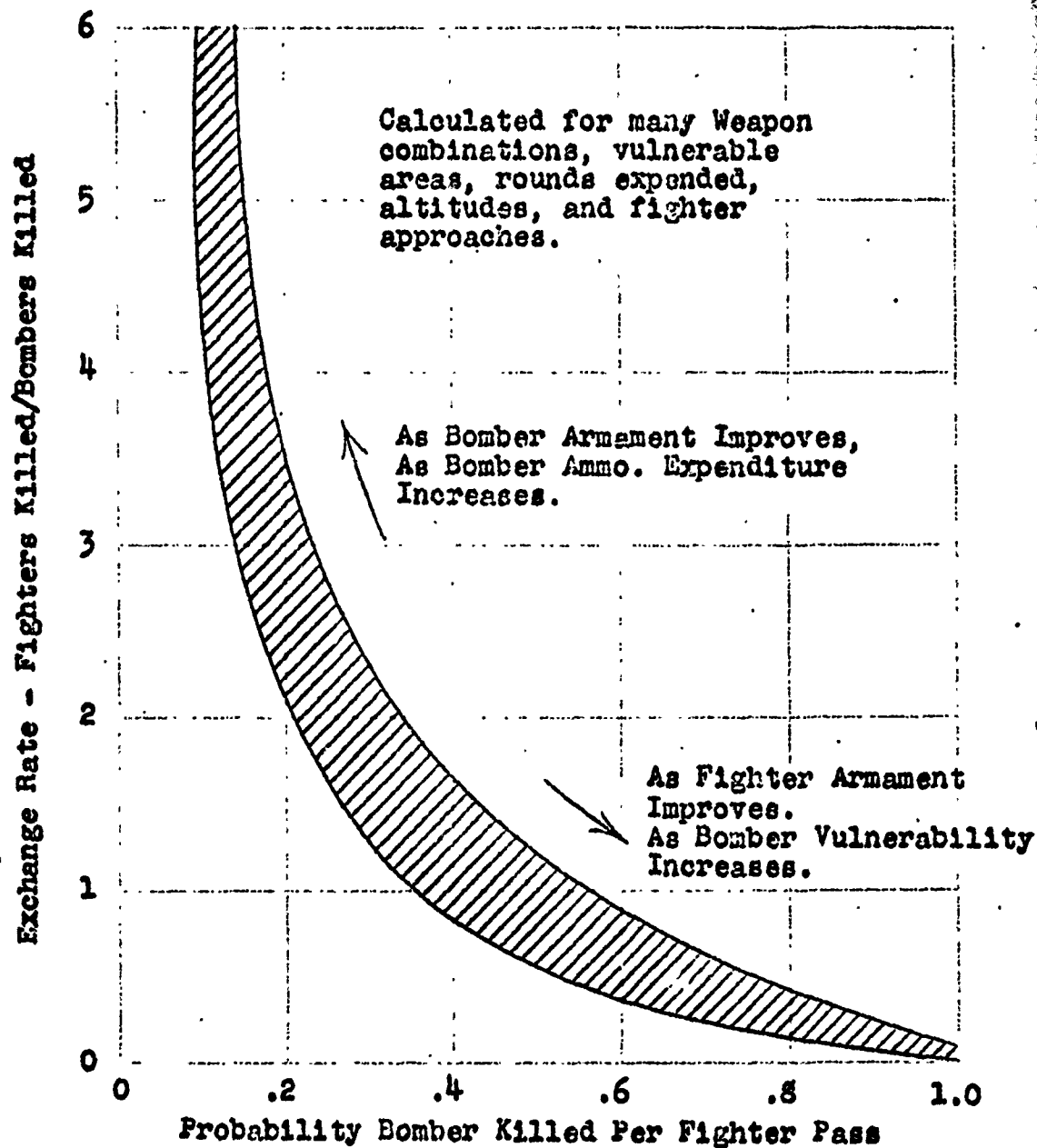
FIG. 7 RANGE OF POSSIBLE BOMBER-FIGHTER DUEL RESULTS 500 K Bomber VS 550 K Fighter
