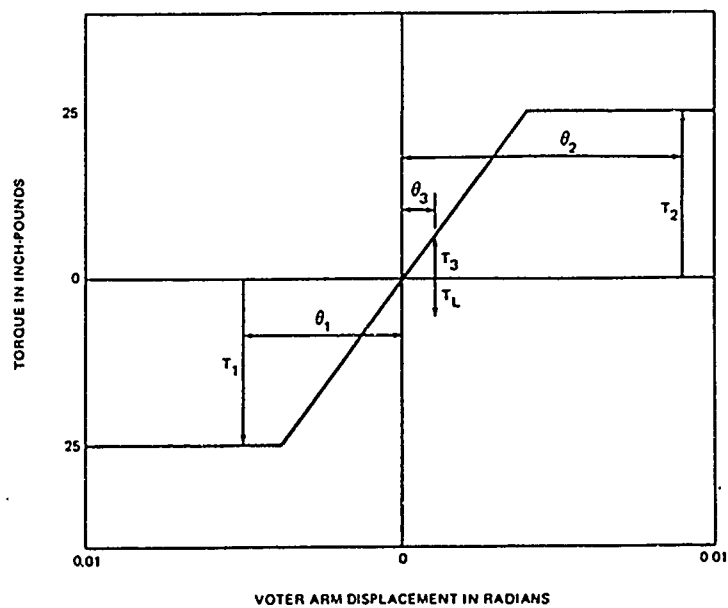
FIGURE 9. VOTER OPERATION
