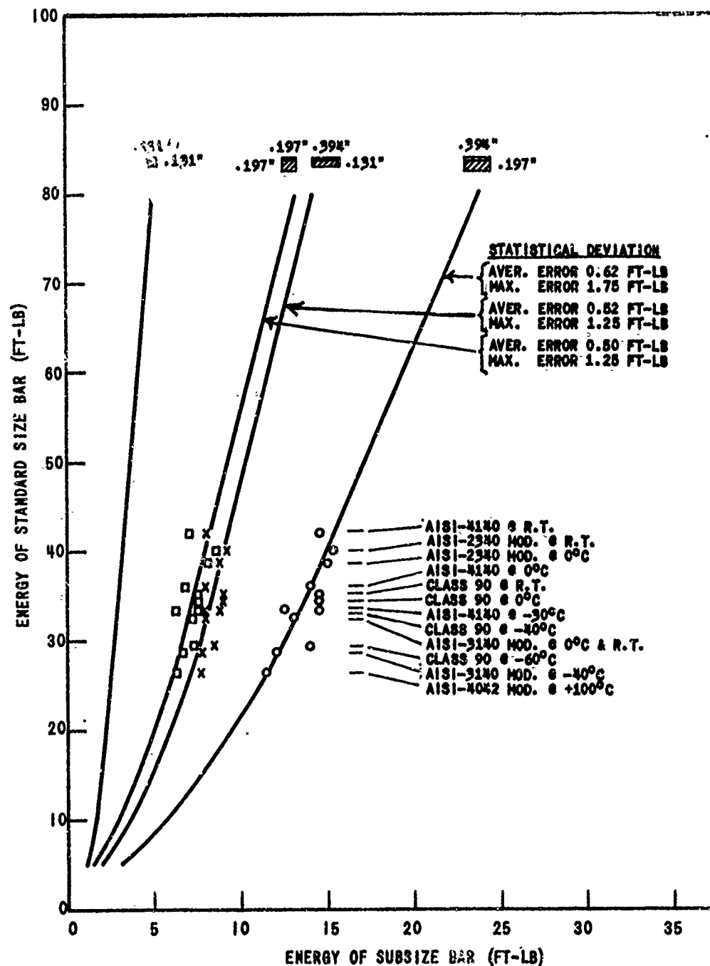
CORRELATION CURVES FOR SUBSIZE CHARPY IMPACT SPECIMENS ABOVE TRANSITION RANGE WITH DATA FROM FIVE OTHER STEELS PLOTTED ON ESTABLISHED CURVES FOR VERIFICATION OF CORRELATION
