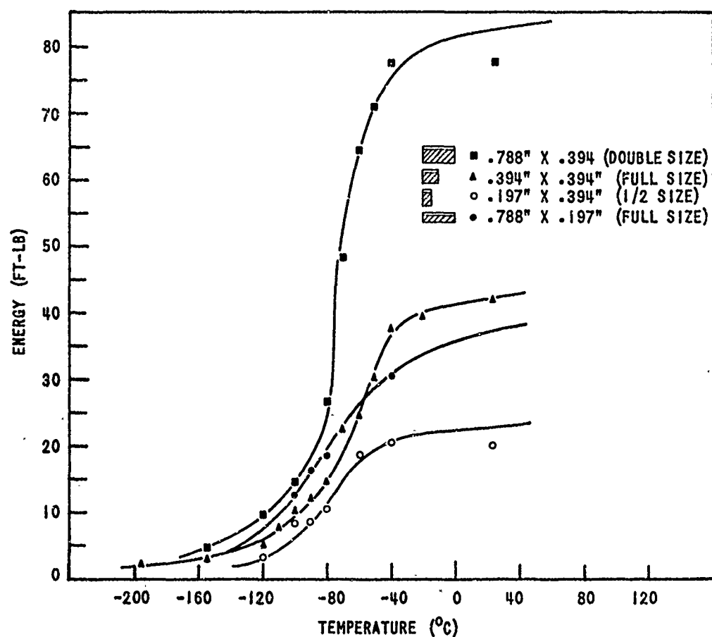
ENERGY VERSUS TEMPERATURE - CHARPY V NOTCH NICKEL STEEL (TAKEN FROM REFERENCE 3)
