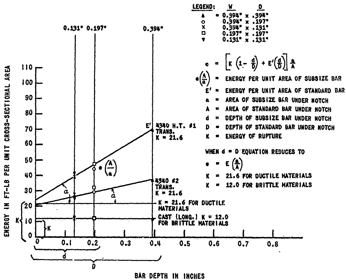
ENERGY VERSUS BAR DEPTH - SHOWING RELATIONSHIP OF RUPTURE AND DEFORMATION DATA TAKEN FROM CURVES OF FIGURES 2, 3, AND 4 AT -40°C TEST TEMPERATURE
