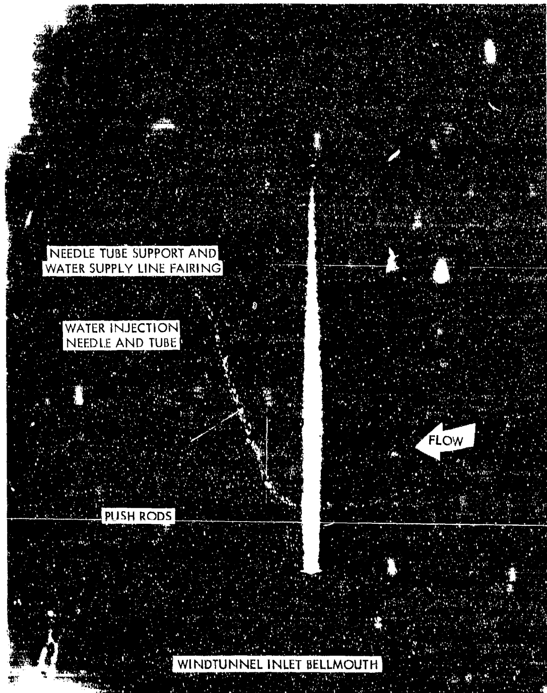
VIBRATING SINGLE-NEEDLE RAIN DISPERSION SET-UP FIGURE A-5
