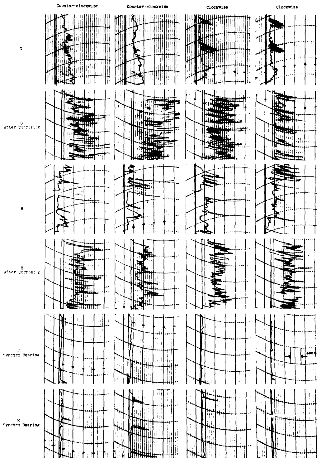
FIG. 10. STANDARD NO. 37 BEARINGS AND NO. 37 BEARINGS SPECIALLY PROCESSED FOR USE IN SYNCHRONOUS UNITS
